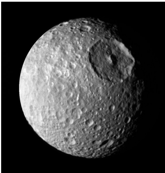
Fig. 10.5 The moon Mimas is notable for its large Herschel crater. (Image courtesy of NASA)
