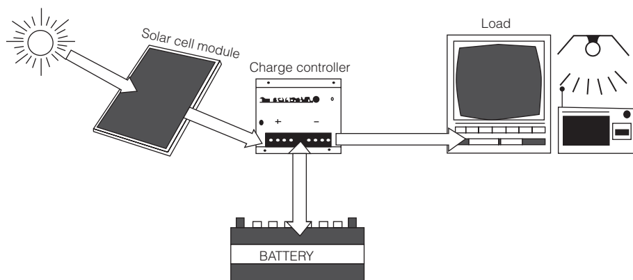
Figure 5.1 The role of a charge controller in off-grid PV systems
