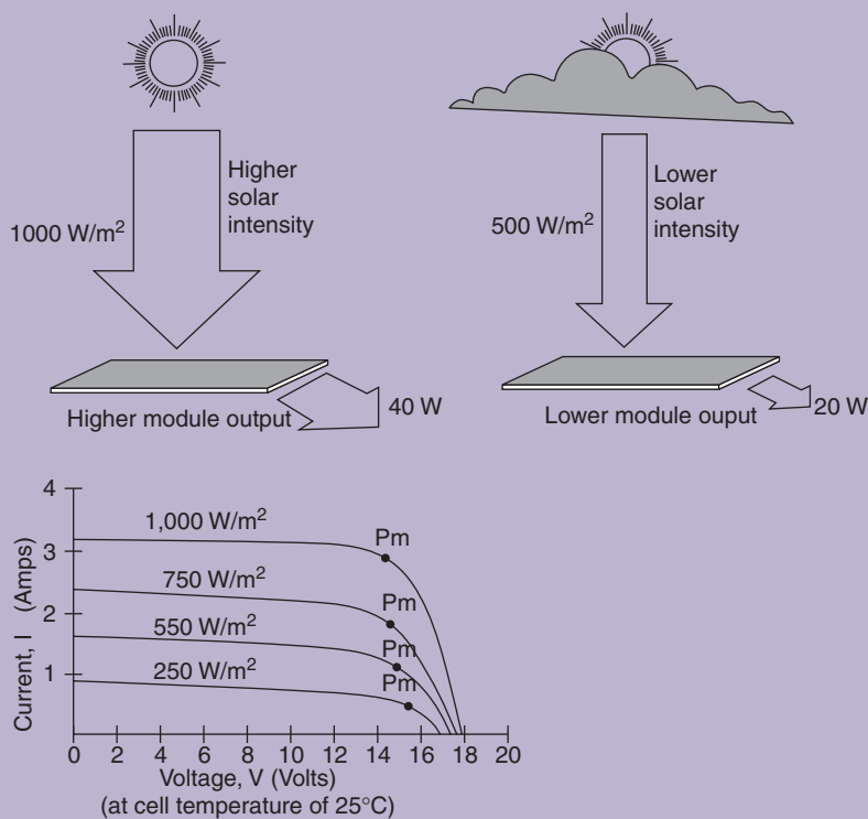
Figure 3.5 Effects of radiation intensity on module output
