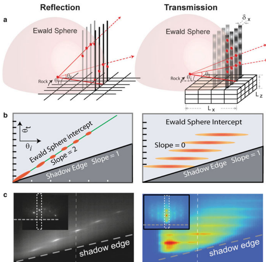
Fig. 13.5 Surface electron diffraction pattern in different conditions. (a) Ewald sphere construction in the grazing incidence angle geometry. By tilting (rocking) the angle of incidence between the electron beam and the sample, the Ewald sphere intercepts the reciprocal lattice rods (relrods) at different height. The coherent diffraction condition is satisfied when the intercept is at the reciprocal lattice node. The left panel shows diffraction from 2D surface. Because there is almost no structure within each relrod, the diffraction exhibits ring patterns simply at the locations where Ewald sphere intercept with relrods. The right panel shows diffraction from 3D finite-size materials with reciprocal nodes broadened by the finite persistence length L of the sample. Sampled by the elongated Ewald sphere intercepts, the diffraction pattern exposes the multiple periodic modulations along the relrods, characteristic of the crystal structure. (b) The simulated rocking maps for the two diffraction scenarios described in (a). (c) Experimental rocking maps taken from a smooth Si/SiO 2 surface and micrograined highly oriented pyrolytic graphite (HOPG) surface [27]
