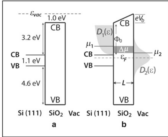
Fig. 13.18 (a) A band diagram depicting the Si/SiO 2 /vacuum interface. (b) Schematic of the energy diagram with relevant quantities used for the tunneling calculations. Electrons that tunnel through the oxide to the SiO 2 /vac interface cause the quasi-Fermi level \mu_2 to raise, making the barrier take on a trapezoidal shape. The electronic density of states is shown in light-gray for the silicon ( D_1 ) and the SiO 2 /vac interface ( D_2 ). The difference between the two levels, \Delta\mu ( dark gray band ) is the primary factor in determining the tunneling current. For a given energy ( \epsilon ), when \Delta\mu , D_1(\epsilon) , and D_2(\epsilon) are all \neq 0 , then there will be a tunneling current through the SiO 2 [33]
