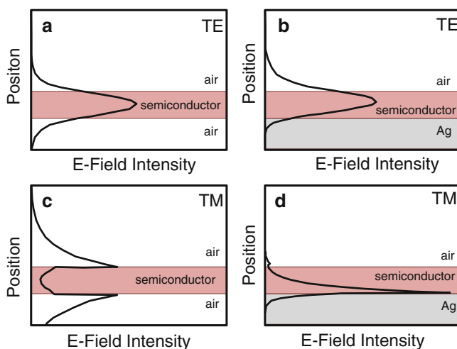
Fig. 14.16 Mode profiles for the lowest order TE [(a) and (b)] and TM [(c) and (d)] modes of a simple slab waveguide. When the backside is a metal, it is possible to excite a surface plasmon polariton, which is tightly confined to the metal–semiconductor interface (d)
