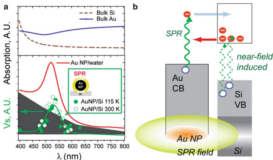
Fig. 13.13 Ultrafast transport at gold nanoparticle (NP)/SAM/silicon interface near surface plasmon resonance (SPR) excitation. (a) The maximum transient photovoltage response near SPR excitation, as compared to the absorption of the similar nanoparticles in water, bulk gold, and silicon substrate. It is evident that while both show characteristic SPR peak at \approx 525 nm the nanoparticle's V_s spectrum at surface lacks the background seen in the optical absorption spectrum of similar nanoparticles in water. (b) The enhancement of hot carrier generation at Si surface can be achieved via SPR evanescent field within the Si surface or charge carrier injection from highly excited Au nanoparticle
