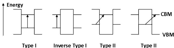
Fig. 9.7 Schematic showing the electronic band alignments for type-I, inverse type-I and type-II quantum dots, with the arrows indicating the lowest energy transitions. CBM conduction band minimum, VBM valance band maximum
