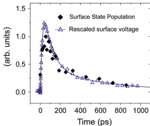
Fig. 13.8 Transient surface state population measured by photoemission [49] (diamonds) compared with the measured transient surface voltage, demonstrating very similar decay rates [25]
