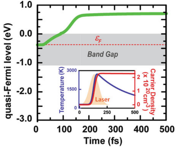
Fig. 13.20 The Boltzmann-Transport Model (BTM) calculation of the quasi-Fermi level of Si following photoexcitation is plotted. The fluence, wavelength, pulse width, and thickness are 35 \text{ mJ/cm}^2 , 800 \text{ nm} , 45 \text{ fs} , and 50 \text{ }\mu\text{m} , respectively. Inset: Zoom-in view of the first 500 fs of evolution in the carrier density, and the carrier temperature, together with the laser temporal profile [33]
