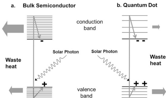
Fig. 9.1 (a) Absorption of a solar photon in a bulk semiconductor initially produces a “hot” electron–hole pair that rapidly cools to the band edge so that the absorbed photon energy in excess of the band gap is lost as waste heat. (b) In a quantum dot, however, the process of MEG can become competitive with cooling and uses some or all of the excess photon energy to produce additional excitons that contribute to the photocurrent and thereby improve the performance of a solar cell
