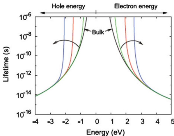
Fig. 9.9 Impact ionization lifetime against the energy of the photoexcited carriers for PbS. Arrows indicate the decrease in size of the QDs and consequent increase in the band gap. Reprinted with permission from [57]. Copyright 2011 American Chemical Society
