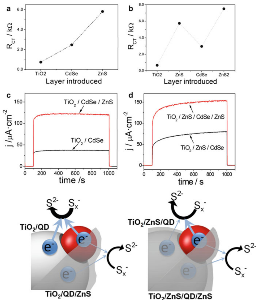
Fig. 1.14 Charge transfer resistances in contact with a polysulfide solution after the successive introduction of the different layers forming TiO 2 /CdSe/ZnS (a) and TiO 2 /ZnS/CdSe/ZnS (b) electrodes. Photocurrent transients for TiO 2 /CdSe and TiO 2 /CdSe/ZnS (c) and TiO 2 /ZnS/CdSe and TiO 2 /ZnS/CdSe/ZnS photoanodes (d). Drawings summarizing the effects of the introduction of the ZnS layers are depicted. The thickness of the arrows is proportional to the rate of the corresponding process. Adapted from [151]—reproduced with permission of the PCCP Owner Societies
