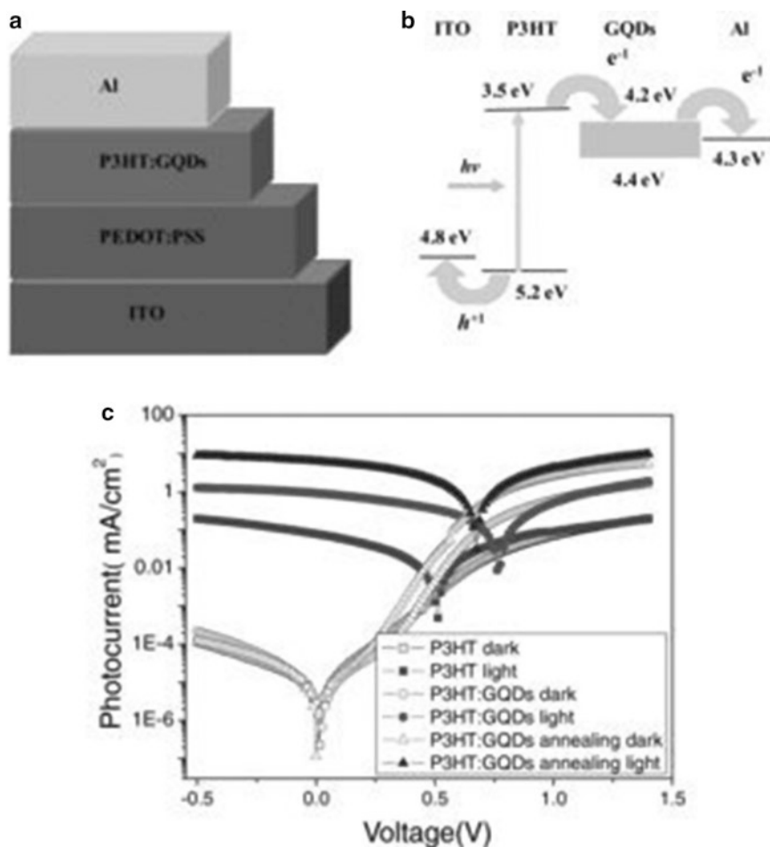
Fig. 10.4 Schematic (a) and energy band (b) diagrams of the ITO/PEDOT:PSS/P3HT:GQDs/Al device. (c) J-V characteristic curves for the ITO/PEDOT:PSS/P3HT/Al, ITO/PEDOT:PSS/P3HT:GQDs/Al and ITO/PEDOT:PSS/P3HT:GQDs/Al devices after annealing at 140^\circ\text{C} for 10 min, single log scale (reprinted with permission from [22]. Copyright (2011) John Wiley and Sons)
