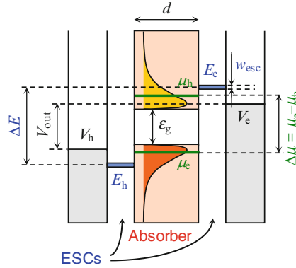
Fig. 8.3 Schematic energy diagram of a hot-carrier solar cell (HC-SC). \epsilon_g : bandgap, d : thickness, \mu_e, \mu_h : quasi-Fermi levels for electrons and holes, respectively, E_e, E_h : ESC energy levels, V_e, V_h : Fermi levels in the electrodes, w_{esc} : ESC energy-selection width. Reproduced with permission from [21]. © 2009, The American Institute of Physics
