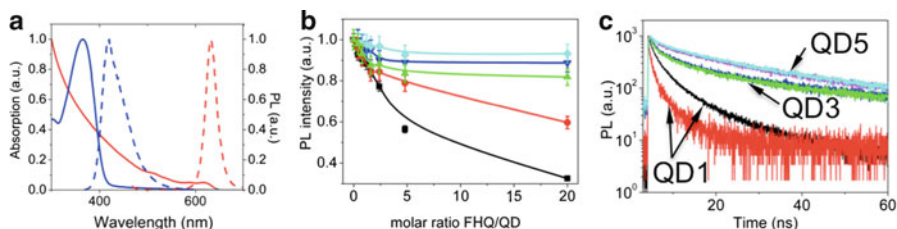
Fig. 4.4 (a) UV-vis (solid) and PL (dash) spectra of QD-1 (red) and FHQ (blue) in aqueous solution. (b) PL intensity vs FHQ/QD molar ratio, R_{\text{FHQ/QD}} , for hybrids based on QD-1 (black square), QD-2 (red dots), QD-3 (green triangles), QD-4 (blue triangles), and QD-5 (magenta rhombs). (c) PL decays of QD-1 (black) and FHQ/QD-1 ( R_{\text{FHQ/QD}} = 20 , red), of QD-2 (green) and FHQ/QD-2 ( R_{\text{FHQ/QD}} = 20 , blue) and of QD-3 (cyan) and FHQ/QD-3 ( R_{\text{FHQ/QD}} = 20 , magenta). Reproduced in part from [23]
