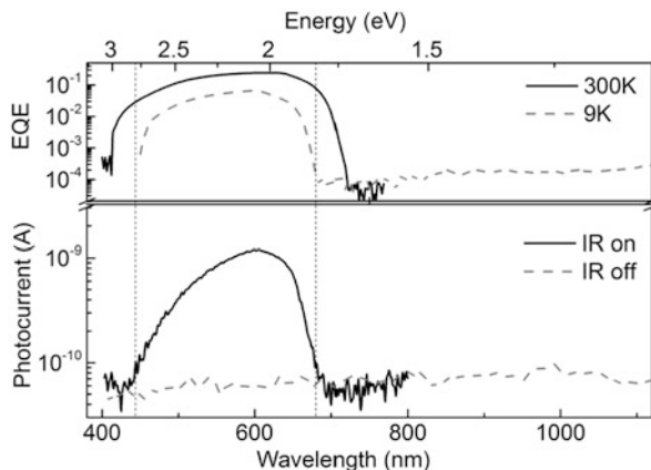
Fig. 7.13 External quantum efficiency (EQE) of device REF for 300 K ( solid curve ) and for 9 K ( dashed curve ). The lower graph shows the generated photocurrent produced by an additionally pulsed IR light source. If the IR source is on, an IR photocurrent was measured in the range between 440 and 680 nm ( black solid curve ). Without IR illumination, no additional photocurrent was detected ( dashed gray curve )
