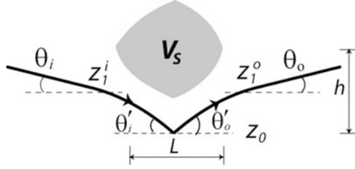
Fig. 13.21 General refraction geometry for grazing incident electron beam. The effective bending of the incident (exit) beam, caused by the local field associated with V_s in the nanostructures, differs depending on the entry (exit) point z_1^i(z_1^o) . Since the relative change of the transverse momentum remains small ( V_s \ll V_0 ), the slab model can be extended to treat the general refraction effect considering an angle- and position-dependent correction factor (see text) [27]
