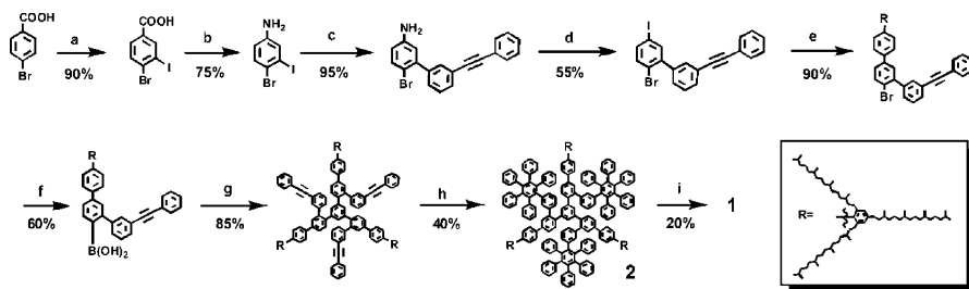
Fig. 10.2 Synthesis of graphene quantum dot 1. Steps are as follows: (a) \text{NaIO}_4 , \text{I}_2 , concentrated \text{H}_2\text{SO}_4 , room temperature. (b) Heated with diphenylphosphoryl azide in triethylamine and tert -butanol at 80^\circ\text{C} , followed by treatment with \text{CF}_3\text{COOH} in dichloromethane at room temperature. (c) Suzuki condition with 3-(phenylethynyl) phenylboronic acid, \text{Pd}(\text{PPh}_3)_4 , \text{K}_2\text{CO}_3 in water, ethanol, and toluene mixture, 60^\circ\text{C} . (d) Iodine and tert -butyl nitrite in benzene, 5^\circ\text{C} to room temperature. (e) Suzuki condition with substituted phenyl boronic acid, \text{Pd}(\text{PPh}_3)_4 , \text{K}_2\text{CO}_3 in water, ethanol, and toluene mixture, 80^\circ\text{C} . (f) Treatment with butyllithium in tetrahydrofuran (THF) at -78^\circ\text{C} , then with triisopropyl borate at -78^\circ\text{C} , followed by treatment with acidic water at room temperature. (g) Suzuki condition with 1,3,5-triiodobenzene, \text{Pd}(\text{PPh}_3)_4 , \text{K}_2\text{CO}_3 in water and toluene mixture, 80^\circ\text{C} . (h) Tetraphenylcyclopentadienone in diphenylether, 260^\circ\text{C} . (i) \text{FeCl}_3 in nitromethane and dichloromethane mixture, room temperature (reprinted with permission from [13]. Copyright 2010 American Chemical Society)
