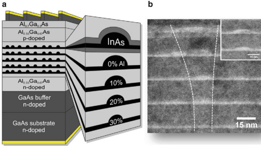
Fig. 7.5 (a) Sketch of the layer sequence of SC samples and magnification of the QD region of devices with “normal” QD arrangement. (b) STEM image of the QD region of SC-1. White dashed lines indicate the alignment of the QDs through the stack
