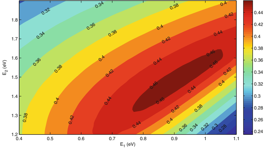
Fig. 6.4 Limiting efficiency of the IBSC with one intermediate band as a function of the two energy transitions E_1 and E_2 for un-concentrated light X = 1 . The color bar on the right-hand side of the contour plot summarizes what efficiencies the various colors represent
