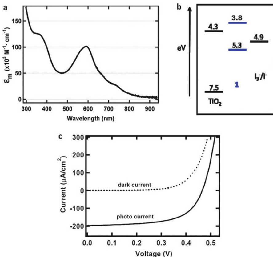
Fig. 10.3 Absorption spectrum of 1 and its application as a sensitizer in nanocrystalline solar cells. (a) Absorption spectrum (molar extinction coefficient \epsilon_m ) of 1 in dichloromethane. (b) The calculated HOMO and LUMO energy levels of 1 , band levels of \text{TiO}_2 , and reduction potential of \text{I}_3^-/\text{I}^- . All values are below the vacuum level in electron volts. The calculated bandgap of 1 is 0.1 eV larger than that measured optically. It nevertheless suffices to illustrate the possible sensitizing effect of 1 on \text{TiO}_2 . (c) The current–voltage characteristics of a typical nanocrystalline \text{TiO}_2 solar cell sensitized by 1 , in the dark and under illumination, respectively (reprinted with permission from [13]. Copyright 2010 American Chemical Society)
