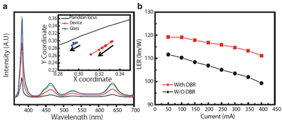
Fig. 3.17 (a) The relative emission spectrum of the QDLED with a DBR structure under various drive currents (50, 150, 250, and 350 mA, from bottom to top curves). The inset is the zoomed-in CIE1931 chromaticity diagram with traces of our QD material when dispensed on glass or packaged in the QDLED format under various pumping powers (for glass) or drive currents (for the QDLED device). (b) The luminous efficacy of optical radiation of UV chips with a DBR structure under currents between 50 and 400 mA [30]
