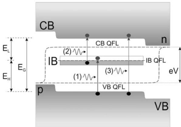
Fig. 7.1 Schematic band diagram of an IBSC with the band gap E_G and the sub band gaps E_H and E_L , respectively. Via a two photon absorption process VB-IB (1) and IB-CB (2) photons with energies less than the bandgap energy can produce electrons with high output voltage
