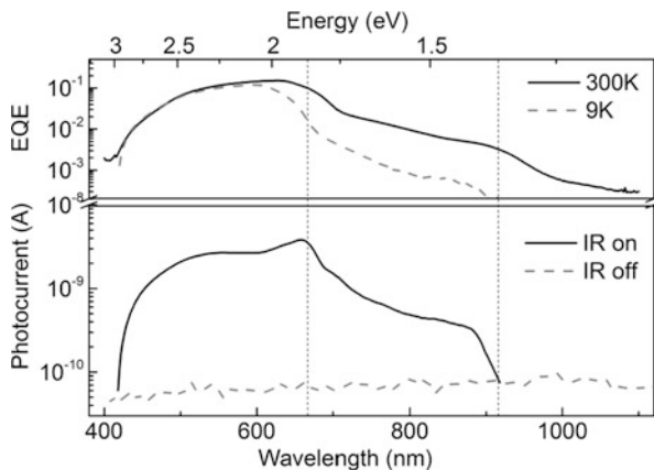
Fig. 7.14 External quantum efficiency (EQE) of device SC-2 for 300 K (solid curve) and for 9 K (dashed curve). The lower graph shows the photocurrent generated of an additionally pulsed infrared (IR) light source. If the IR source is on, a photocurrent produced by this IR source was measured in the range between 420 and 920 nm (black solid curve). Without IR illumination, no additional photocurrent was detected (dashed gray curve)
