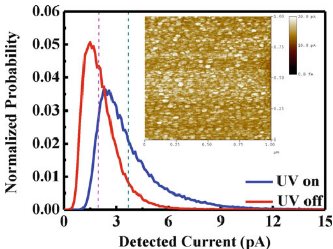
Fig. 3.13 The distribution of detected currents of QD on GaAs surface with and without UV lamp on. The pink and blue vertical lines indicate the average currents from the measurement. When UV lamp is off, the average current is 2.10 pA. If we turn on the UV lamp, the average jump up to 3.69 pA (an 76 % increase). The inset is the conductive AFM scanning plot [49]
