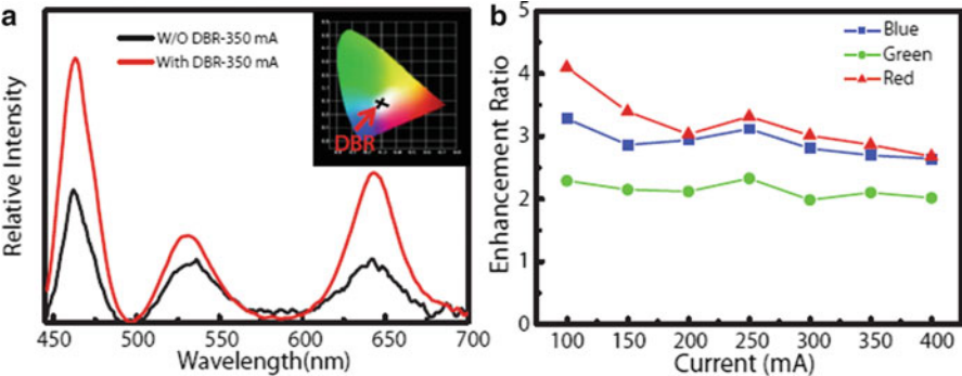
Fig. 3.14 (a) The relative intensity of the large-area samples with and without DBR operated under 350 mA. The inset shows the CIE color coordinates of the large-area samples with DBR. (b) Enhancement ratio of the intensity of large-area samples with and without DBR under various diode currents from 100 to 400 mA [30]
