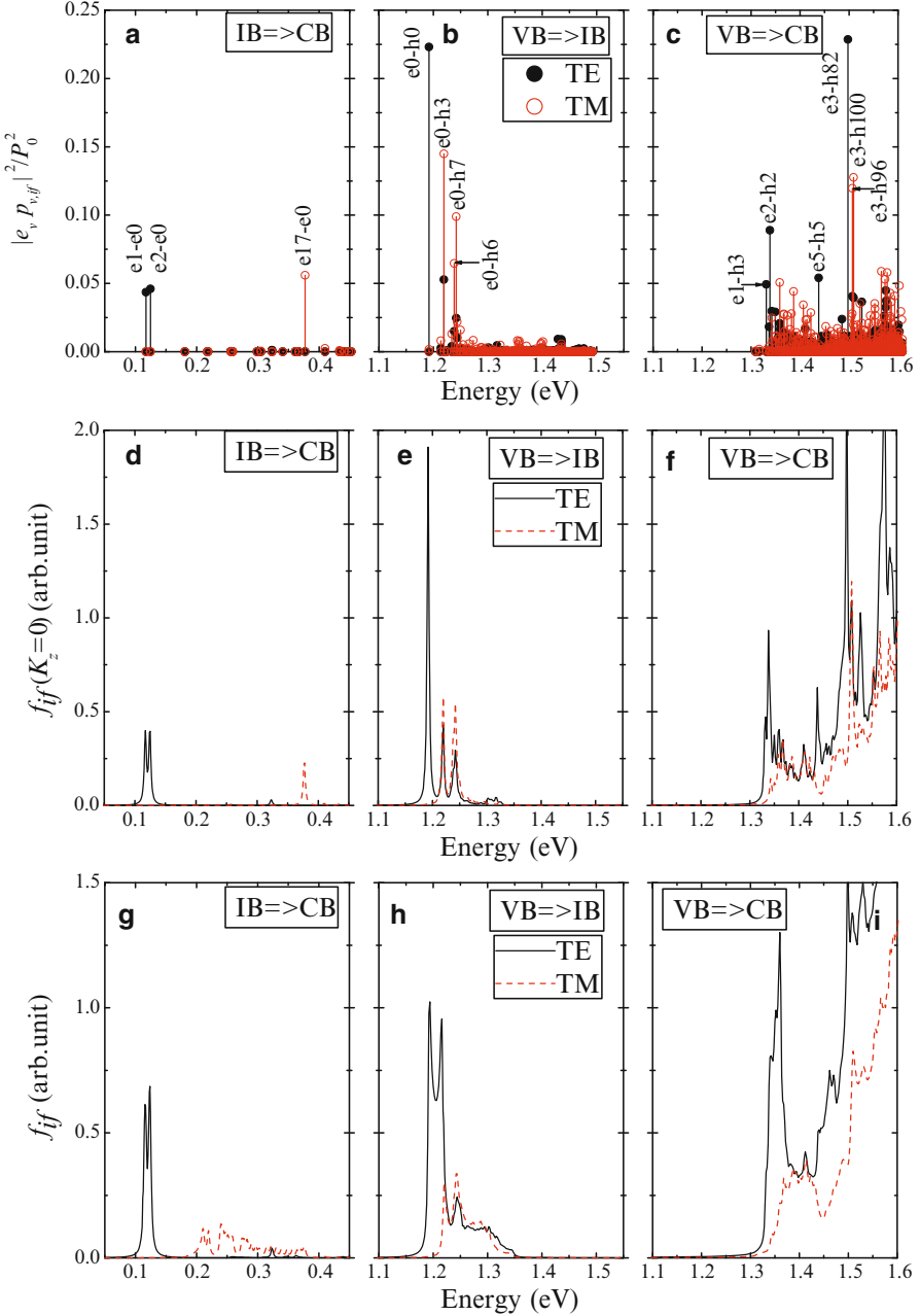
Fig. 5.9 Momentum matrix elements of the QD array with vertical periodicity d_z = 5 nm at K_z = 0 : (a) IB \rightarrow CB transitions, (b) VB \rightarrow IB transitions, (c) VB \rightarrow CB transitions; the transition strength for the same array at the band edge K_z = 0 , (d) IB \rightarrow CB transitions, (e) VB \rightarrow IB transitions, (f) VB \rightarrow CB transitions; and the transition strength for the same array summed over all K_z states, (g) IB \rightarrow CB transitions, (h) VB \rightarrow IB transitions and (i) VB \rightarrow CB transitions. Both the TE (solid symbol or solid line) and TM (open symbol or dashed line) polarizations are shown
