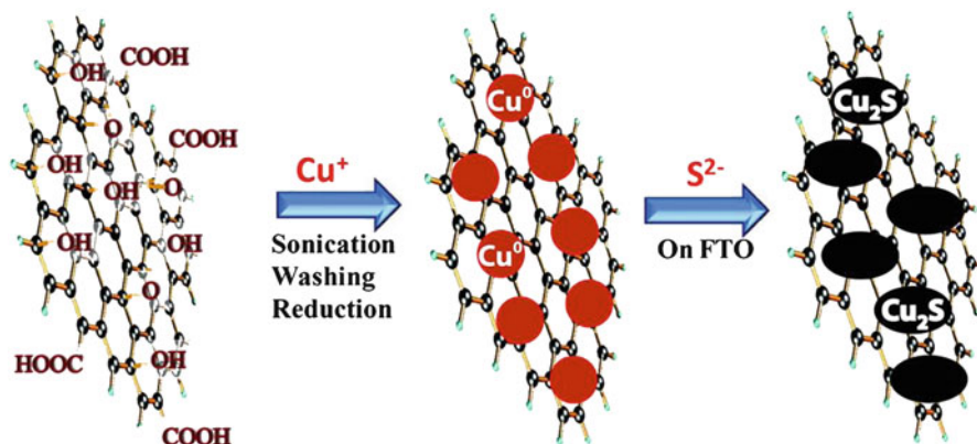
Fig. 11.4 Synthetic steps of Cu 2 S/RGO composite material. Reprinted with permission from [9]; Copyright © 2011 The American Chemical Society
