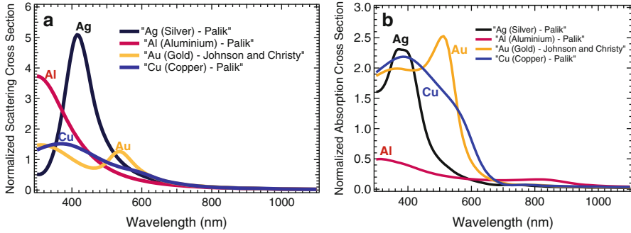
Fig. 14.9 The normalized scattering (a) and absorption (b) cross section for spherical particles (silver, aluminum, gold, and copper) of radius 50 nm in a vacuum environment ( n = 1 )
