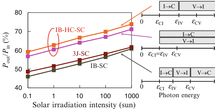
Fig. 8.28 (Left) Conversion efficiency of intermediate-band-assisted hot-carrier solar cells (IB-HC-SCs) using indirect-bandgap absorbers, depending on the solar irradiation intensity. \tau_{\text{th}} = 1 ns. The bandgap values and other parameters are optimized for each case. Results for IB-SCs with perfect photon selectivity and 3J-SCs are also shown for comparison. (Right) Absorption ranges for each interband transition. I→C: IB to CB (bandgap \epsilon_{CI} ), V→I: VB to IB (bandgap \epsilon_{IV} ), V→C: VB to CB (bandgap \epsilon_{CV} ). Reproduced with permission from [99]. © 2012, John Wiley & Sons, Ltd.
