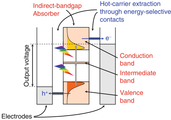
Fig. 8.27 Schematic energy diagram of an intermediate-band-assisted hot-carrier solar cell (IB-HC-SC) and operating principle. Reprinted with permission from [99]. © 2012, John Wiley & Sons, Ltd.
