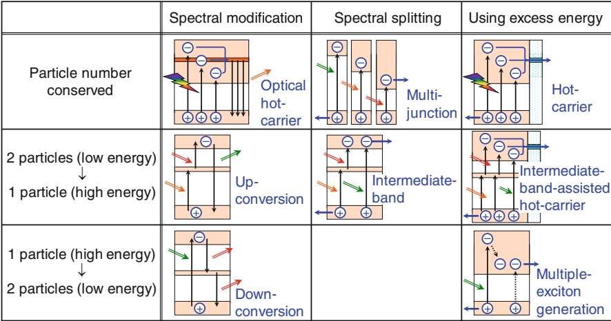
Fig. 8.1 Concepts of solar cells to exceed the Shockley–Queisser (SQ) limit
