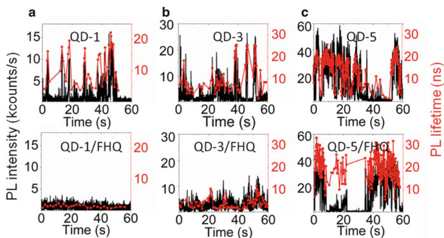
Fig. 4.8 Time trajectories of single molecule PL intensity (black) and PL lifetime (red) for isolated QDs (upper panel) and FHQ/QD-1 hybrids (lower panel): (a) QD-1 and FHQ/QD-1; (b) QD-3 and FHQ/QD-3; (c) QD-5 and FHQ/QD-5. Reproduced from [23]
