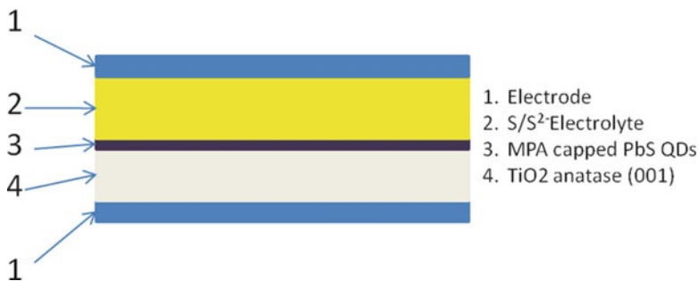
Fig. 9.5 Schematic of the device used to demonstrate a photocurrent enhanced by MEG [42] consisting of: (1) two electrodes; (2) an aqueous S/S^{2-} electrolyte; (3) MPA-capped PbS QD monolayer and (4) an atomically flat (0 0 1) anatase TiO_2 substrate (MPA mercaptopropionic acid)
