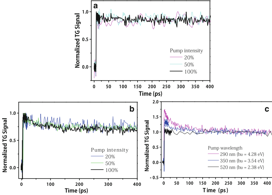
Fig. 12.7 (a) Normalized TG kinetics of the PbS QDs for the wavelength of 520 nm ( h\nu = 1.9E_g ), in which the pump light intensity decreased from 4.2 \mu\text{J/pulse} (100 %) to 0.84 \mu\text{J/pulse} (20 %); (b) normalized TG kinetics of the PbS QDs for the wavelength of 350 nm ( h\nu = 2.83E_g ), in which the pump light intensity decreased from 0.9 \mu\text{J/pulse} (100 %) to 0.18 \mu\text{J/pulse} (20 %); (c) a comparison of the TG kinetics of the PbS QDs normalized at 400 ps for three different wavelengths of 520 nm ( h\nu = 1.9E_g ), 350 nm ( h\nu = 2.83E_g ) and 290 nm ( h\nu = 3.42E_g )
