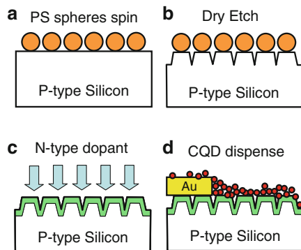
Fig. 3.5 The schematic fabrication flow for c-Si nanopillar arrays (NPA) solar cell with CdS quantum dots (QDs) layers: (a) spin-cast of nearly-close-packed polystyrene nanospheres monolayer, (b) resulting NPA after dry etching, (c) diffusion of an N-type layer. (d) \text{SiN}_x deposition and screen printing of the front and back electrodes, and then spin CdS QDs layers on the cell [18]
