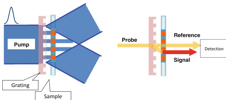
Fig. 12.3 Schematic illustration of the principles of generation and detection of a transient grating in a sample using the transient grating technique
