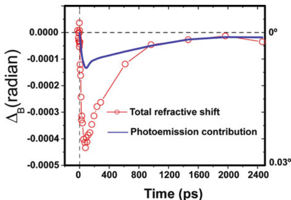
Fig. 13.9 Experiments to characterize surface photovoltage and photoelectron dynamics performed at F = 65 \text{ mJ/cm}^2 . Data (symbols, colored in red) show the refraction shift of a selected diffracted beam. An N -particle simulation to estimate the refraction contribution associated with photoemission is shown (solid line, colored in blue) for comparison [27]
