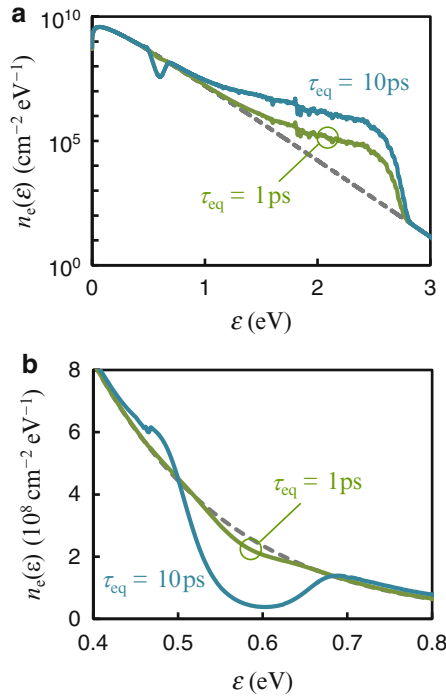
Fig. 8.20 Carrier energy distribution n_c(\epsilon) depending on the carrier equilibration time \tau_{eq} . \tau_{th} = 1 \text{ ns} , w_{esc} = 0.1 \text{ eV} . \epsilon_g , E_{esc} and other parameters are optimized for each case. (a), (b) 1 sun, \epsilon_g = 1.12 \text{ eV} , E_{esc} = 0.58 \text{ eV} above the CBM, T_{eq} = 1,590 \text{ K} . (c), (d) 1,000 sun, \epsilon_g = 0.93 \text{ eV} , E_{esc} = 0.61 \text{ eV} above the CBM, T_{eq} = 1,700 \text{ K} . Broken lines show the equilibrated distribution f(\epsilon; \mu_{eq}, T_{eq}) \rho_c(\epsilon)
