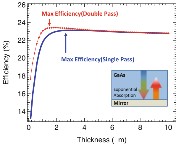
Fig. 14.3 Efficiency as a function of thickness for single and double pass absorption. The maximum efficiency is a trade-off between high absorption efficiency (thick device) and high carrier collection efficiency (thin device). The use of a mirror back reflector allows a device to be half as thick and still absorbs the same amount of light
