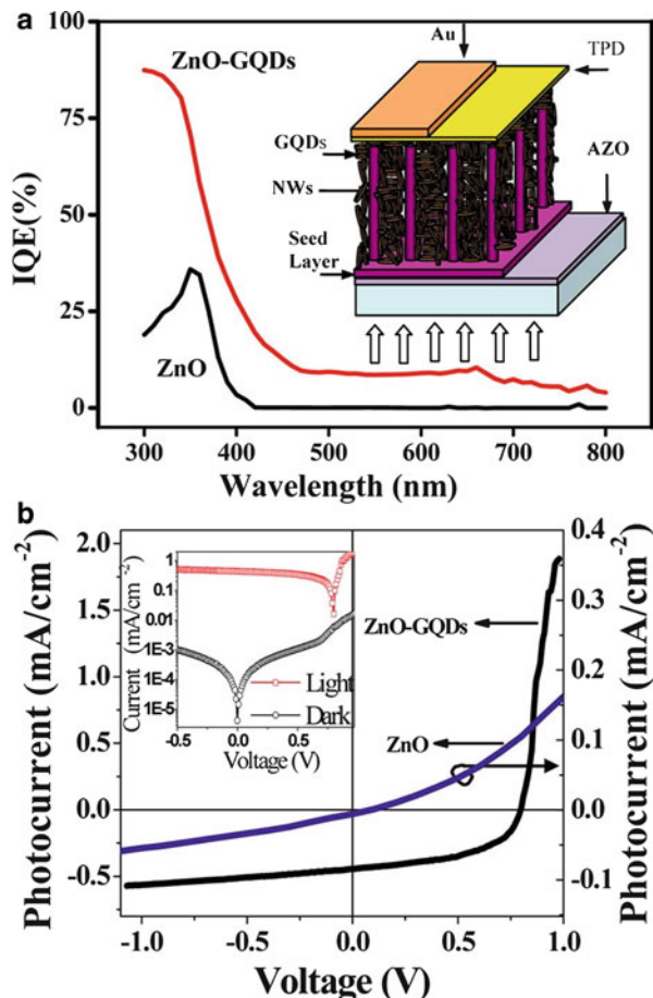
Fig. 10.10 (a) IQE of the samples. The inset shows the schematic model of the device. (b) Solar cell I - V characteristics under white light illumination. The inset shows the logarithmic plot of dark and photo current of the GQDs-ZnO cell (reprinted with permission from [25]. Copyright (2012) American Chemical Society)
