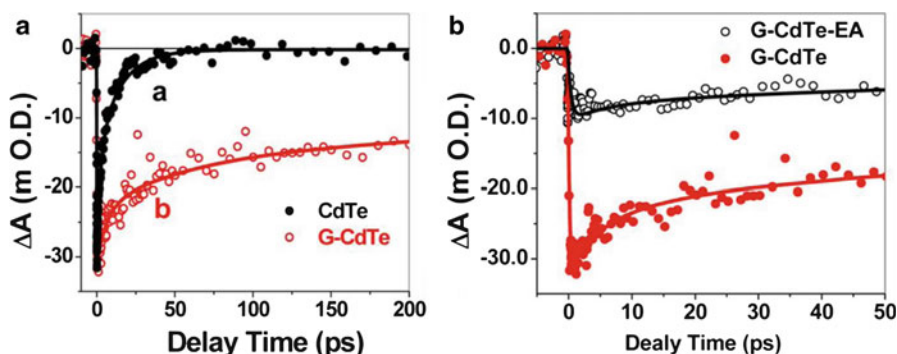
Fig. 11.2 (a) Bleach recovery kinetics at 460 nm for (a) CdTe and (b) CdTe/graphene pumping at 400 nm and (b) kinetics decay traces at 460 nm for CdTe/graphene (G-CdTe) and CdTe/graphene with electron quencher (G-CdTe-EA) pumping at 400 nm. Reprinted with permission from [34]; Copyright © 2012 The American Chemical Society
