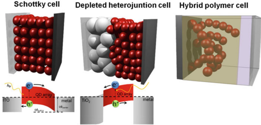
Fig. 1.1 Sketches illustrating the different types of solar cells based on colloidal QDs, apart from the QDSSC: Schottky cell, depleted heterojunction cell and hybrid bulk heterojunction cell. Energy-band diagrams for the first two devices are also included
