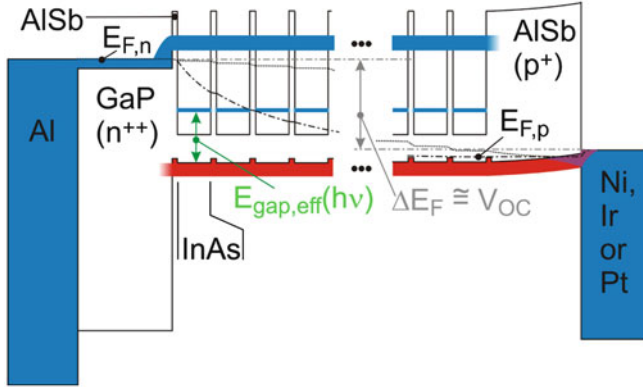
Fig. 8.25 Schematic energy diagram of a hot-carrier solar cell using an MQW absorber. Reprinted with permission from [93]. © 2012, The American Institute of Physics
