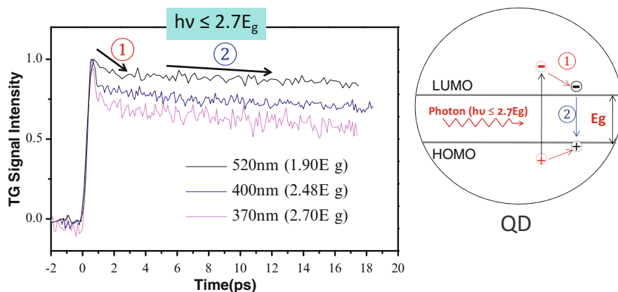
Fig. 12.9 Normalized TG kinetics for pump light wavelengths decreasing from 520 nm ( h\nu : 1.9E_g ) to 370 nm ( h\nu : 2.70E_g )
