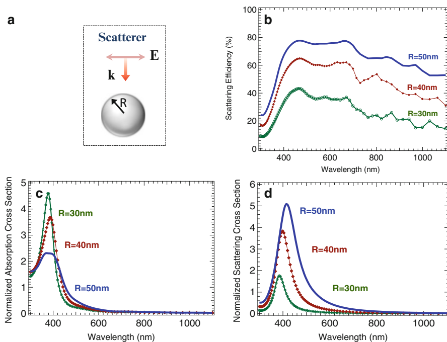
Fig. 14.13 (a) Schematic of the simulations for Ag spheres with radii of 30, 40, and 50 nm in vacuum ( n = 1 ). (b) Scattering efficiency. (c) Normalized absorption cross section. (d) Normalized scattering cross section
