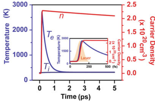
Fig. 13.6 Non-thermal Boltzmann transport coupled two-temperature model calculations of electronic/ionic temperature ( T_e , T_i ) and carrier density induced by 800 nm femtosecond laser in silicon. The laser fluence and pulse width are 65 \text{ mJ/cm}^2 and 45 fs, and the silicon sample thickness is 50 \mu\text{m} [33]. Inset: Closeup view of the first 500 fs [33]
