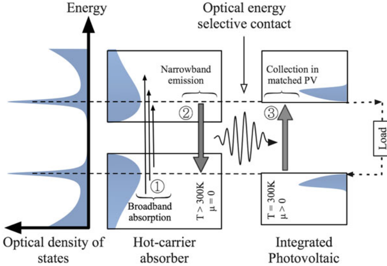
Fig. 8.26 Operating principle of an optical hot-carrier solar cell. Reprinted with permission from [96]. © 2011, The American Institute of Physics
