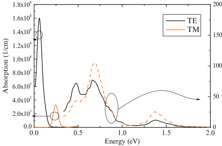
Fig. 5.8 Bound-to-bound spectra of 2D QD array with b = 10 nm and d_x = d_y = 1 nm, left axis, and bound-to-continuum right axis. All spectra are broadened with the line broadening of \Delta E = 25 meV
