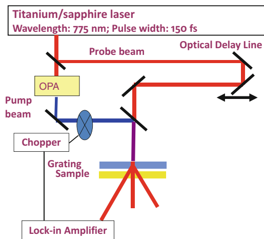
Fig. 12.4 Setup of the improved transient grating technique
