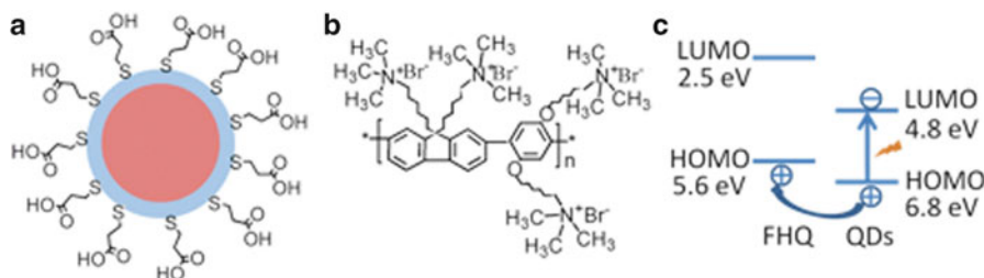
Fig. 4.1 (a) MPA-capped core/shell CdSe/ZnS quantum dots (QDs) and (b) cationic conjugated polymer FHQ. (c) Scheme for photoinduced hole transfer between QD and FHQ. Reproduced in part from [23]
