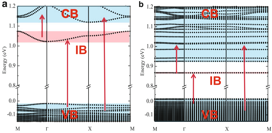
Fig. 5.6 Electronic structure of the laterally coupled 2D QD array throughout the first BZ: (a) array made of QDs with b = 10 nm and d_x = d_y = 1 nm and (b) array made of QD with b = 20 nm and d_x = d_y = 5 nm
