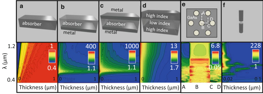
Fig. 14.23 Potential solar cell architectures. (a) Planar slab in air in which the LDOS is always below the bulk value. Structures with the potential to beat the ergodic limit. (b) Planar slab with an Ag back-reflector, (c) metal–absorber–metal planar structure, (d) high/low/high index structure with refractive, (e) a photonic crystal, and (f) a split dipole antenna with an absorber in the gap. The second row shows the LDOS enhancement (on a log scale) over the bulk material for each structure for various cell thicknesses and wavelengths. Values of LDOS enhancement >1 correspond to beating the traditional absorption limit. Adapted from [21]
