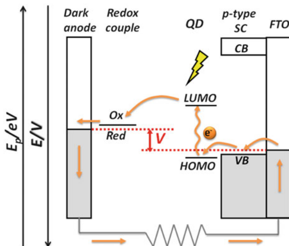
Fig. 1.7 Working scheme of a solar cell with a quantum dot-sensitized photocathode. SC denotes semiconductor
