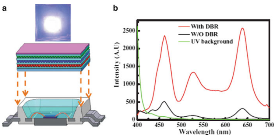
Fig. 3.16 (a) Top : the QDLED device in action; bottom : the device schematic diagram. (b) EL spectra with and without the DBR structure [30]
