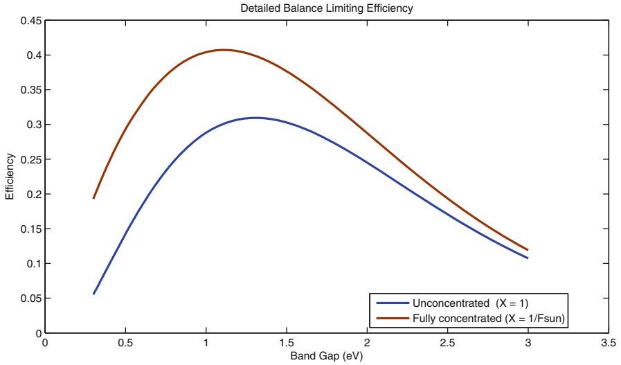
Fig. 6.1 Detailed balance limiting efficiency of a photovoltaic device as a function of the band gap for unconcentrated light X = 1 and fully concentrated light X = 1/F_{\text{sun}} . The efficiency was calculated assuming the sun is modeled as a blackbody with characteristic temperature 6,000 K. For fully concentrated light, the maximum efficiency of about 41% occurs approximately at a band gap of E_g = 1.1 eV, while unconcentrated light leads to a maximum efficiency of about 31% with a band gap of E_g = 1.31 eV
