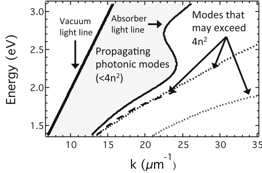
Fig. 14.21 Waveguide dispersion relations. Plasmonic, metal–insulator–metal, and high–low–high index dielectric slot waveguides have dispersion relations that lie to the right of the bulk absorber light line, which have large propagation constants, slow group velocities, and are well confined. Adapted from [19]
