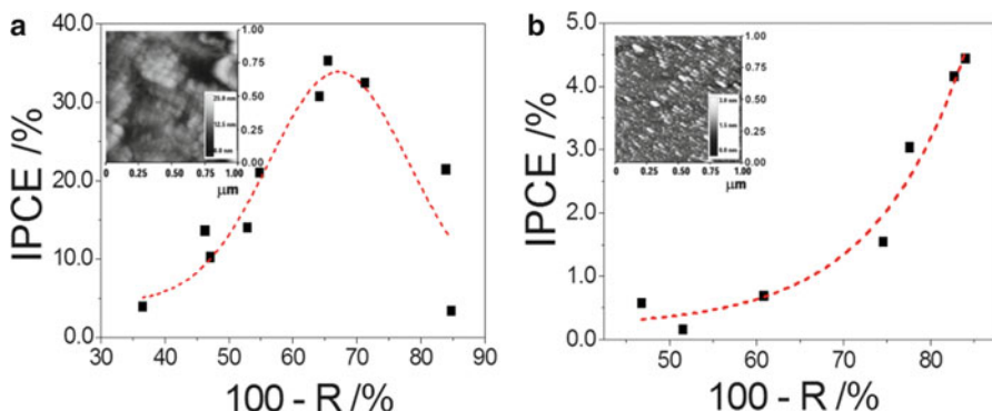
Fig. 1.11 IPCE at the excitonic peak vs 100-Reflectance % at the excitonic peak for direct (a) and MPA-mediated (b) adsorption. The inset shows the tapping-mode AFM images of an Nb-doped (1 1 0) rutile single crystal sensitized in the same way. The images clearly show the generation of aggregates for direct adsorption when a long adsorption time is employed. Adapted with permission from [66]
