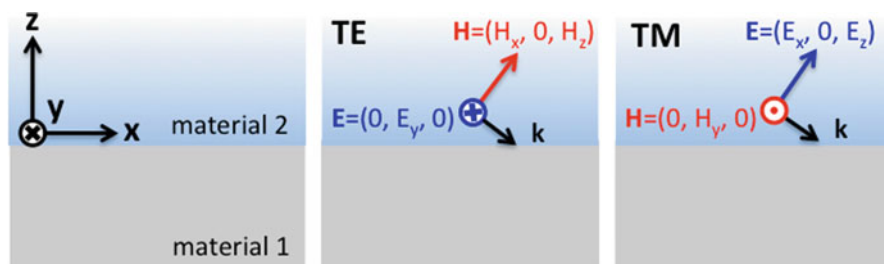
Fig. 14.15 TE and TM modes for a simple two-material waveguide. The interface corresponds to z = 0
