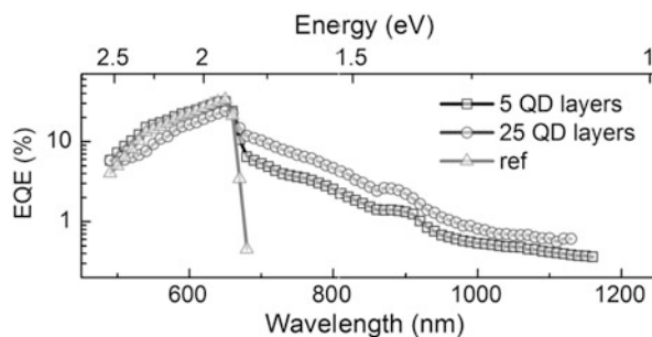
Fig. 7.10 Comparative EQE measurements of device SC-2 (5 QD layers), SC-3 (25 QD layers), and the reference sample REF (w/o QDs)
