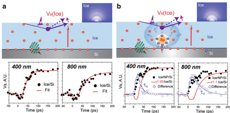
Fig. 13.15 (a) Controlled experimental measurements of ice surface photovoltage without the presence of nanoparticles. The rise of the surface voltage is generally delayed by the timescale of the energetic charge carriers migrating to the surface after being launched from the Si substrate. (b) Equivalent results obtained the surface with Au nanoparticles decoration. By comparing (a) and (b), we can deduce the fast components (blue circles) unique to nanoparticle (NP)-decorated surface [93]
