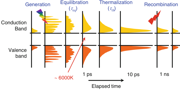
Fig. 8.2 Time evolution of carrier energy distribution after pulsed solar irradiation. \tau_{eq} : carrier equilibration time, \tau_{th} : carrier thermalization time
