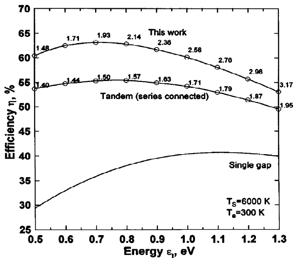
Fig. 7.2 Efficiency limit for an IBSC as a function of the low bandgap energy E_L . The efficiency for a single gap solar cell is also presented (reproduced from Luque et al. [10])
