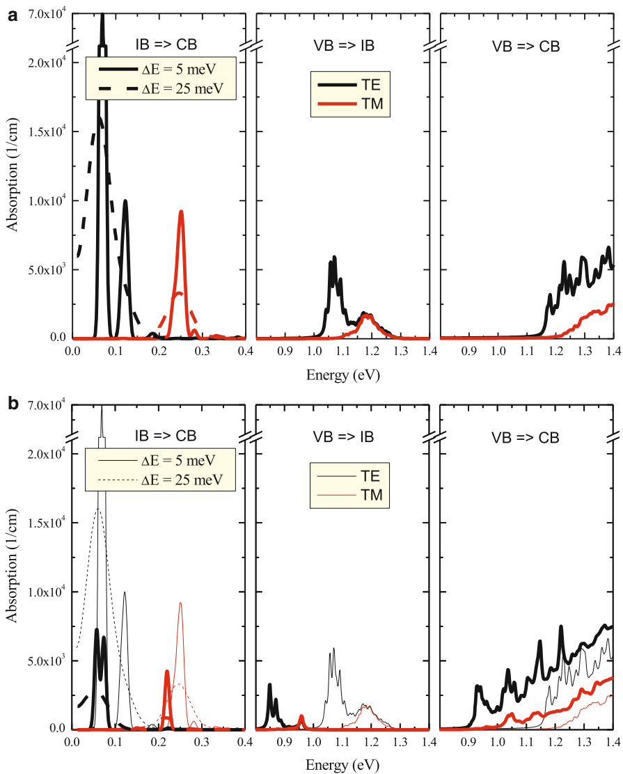
Fig. 5.7 Absorption coefficients of the laterally coupled 2D QD array: (a) the array made of QDs with b = 10 nm and d_x = d_y = 1 nm and (b) the array made of QD with b = 20 nm and d_x = d_y = 5 nm. Dotted lines in IB \rightarrow CB spectra present absorption coefficients calculated with line broadening of \Delta E = 25 meV
