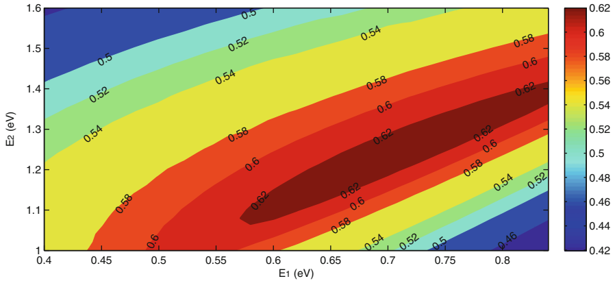
Fig. 6.5 Limiting efficiency of the IBSC with one intermediate band as a function of the two energy transitions E_1 and E_2 for fully concentrated light X = 1/F_{\text{sun}} . The color bar on the right-hand side of the contour plot summarizes what efficiencies the various colors represent
