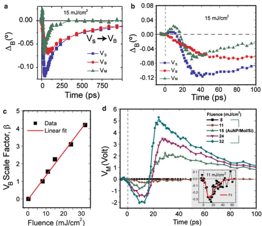
Fig. 13.12 Ultrafast transport at gold nanoparticle/SAM/silicon interface. (a) The overall refraction shift determined by SAM diffracted beam (labeled V_S ), the background (labeled V_B ) scaled to match the long time transient of V_S , and the molecular charge transport contribution, labeled V_M , obtained by subtracting \Delta_B(V_B) from \Delta_B(V_S) . The data are obtained at F = 15 \text{ mJ/cm}^2 . (b) The short time response of (a). (c) The scale factor \beta used in scaling V_B to match V_S in the long time for different fluences, showing a linear trend w.r.t fluence. (d) V_M determined for different fluences, compared to the transient voltage obtained for \text{SiO}_2/\text{Si} at F = 65 \text{ mJ/cm}^2 . Inset, the V_M obtained at F = 11 \text{ mJ/cm}^2 is fit to an RC model with nearly equal time constants of 8 \pm 1 \text{ ps} for charging/discharging [27]
