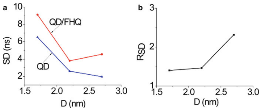
Fig. 4.10 (a) Standard deviation \sigma of PL lifetime vs ZnS shell thickness, t_s , for the distributions shown in Fig. 4.9a–c. (b) Ratio ( R_\sigma ) of standard deviations of PL lifetime for FHQ/QD hybrids and for QDs vs ZnS shell thickness, t_s . Reproduced in part from [23]
