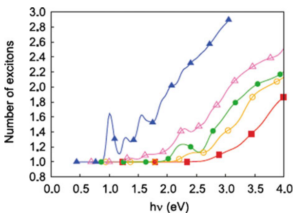
Fig. 9.10 Quantum yield (number of excitons created per absorbed photon) for different QDs sizes corresponding to E_g = 0.44 eV (filled triangles), E_g = 0.69 eV (open triangles), E_g = 0.86 eV (filled circles), E_g = 0.94 eV (open circles), and E_g = 1.24 eV (filled squares). Reprinted with permission from [57]. Copyright 2011 American Chemical Society
