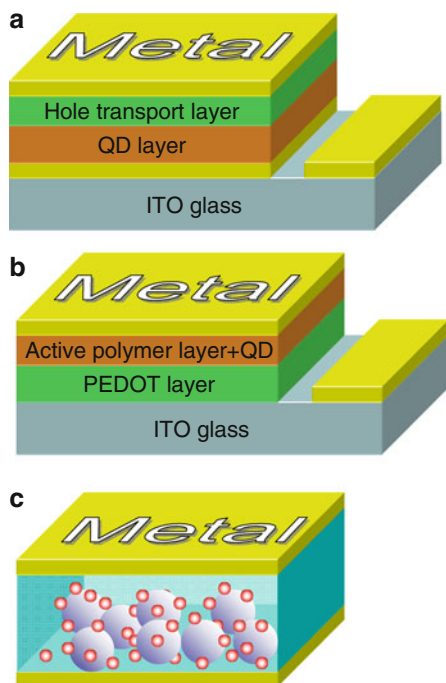
Fig. 3.1 Three types of pure colloidal quantum dot solar cells (a) metal–semiconductor junction, (b) polymer–semiconductor, and (c) semiconductor–semiconductor systems [26]
