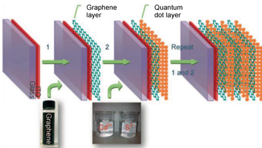
Fig. 11.5 Fabrication of the layered graphene/QDs on ITO glass. (1) Electrophoretic deposition of graphene; (2) sequential SILAR process to synthesize a layer of CdS QDs. The layered graphene/QDs device was obtained by repeating steps 1 and 2. Reprinted with permission from [36]; Copyright © John Wiley and Sons
