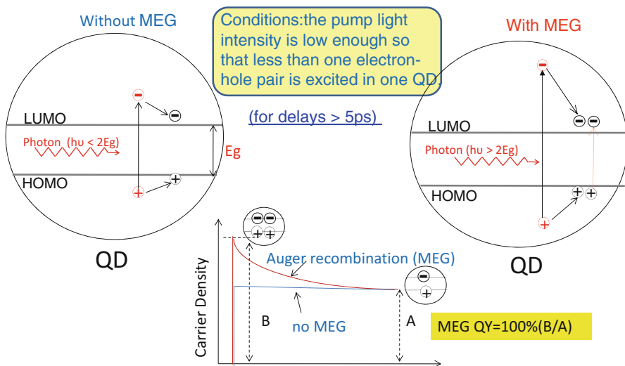
Fig. 12.2 Schematic illustration of MEG characterization using a transient absorption (TA) method
