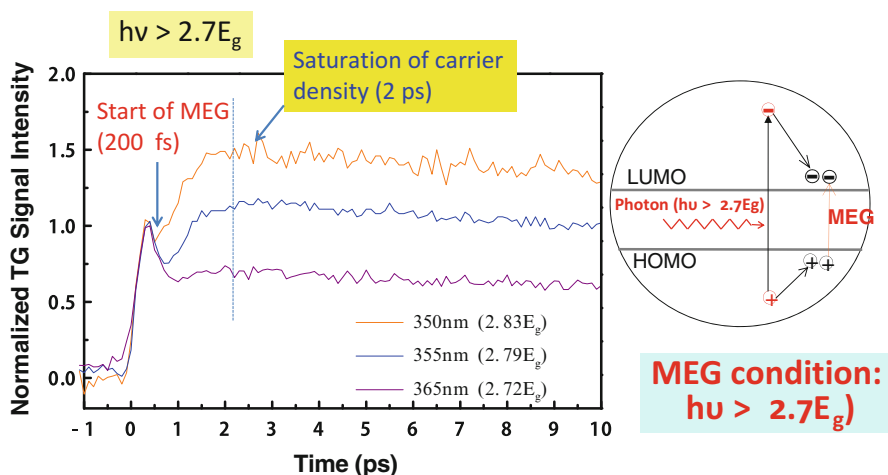
Fig. 12.11 Detailed initial TG kinetics of a part of Fig. 12.10
