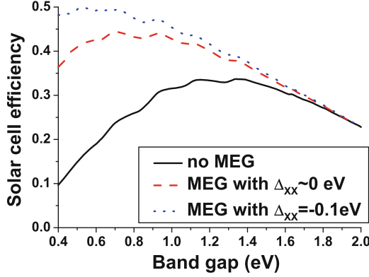
Fig. 9.2 Maximum theoretical solar cell efficiency for a range of band gaps, E_g , calculated using the Detailed Balance Model for a conventional solar cell ( solid line ), and cell in which MEG is efficient but for which the biexciton interaction energy, \Delta_{xx} , is negligible ( dashed line ), and a cell which combines efficient MEG and a large, attractive biexciton energy of \Delta_{xx} = -0.1 eV ( dotted line )
