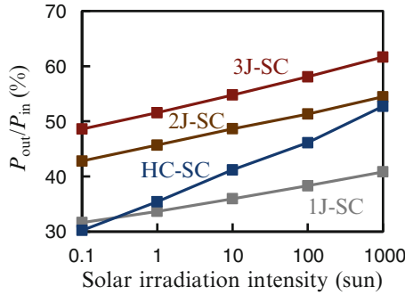
Fig. 8.15 Dependence of conversion efficiency P_{\text{out}}/P_{\text{in}} on the solar irradiation intensity. \tau_{\text{th}} = 1 ns. \epsilon_g , \Delta E and other parameters are optimized for each case. Results for 1J-, 2J- (double-junction), and 3J-SCs are also shown for comparison. Reproduced with permission from [22]. © 2011, Elsevier B.V.
