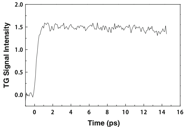
Fig. 12.12 TG kinetics of colloidal CdSe QDs with a bandgap of 2.18 eV (i.e., an optical absorption peak of 570 nm) obtained from Evident Technologies measured under the pump light wavelength of 420 nm
