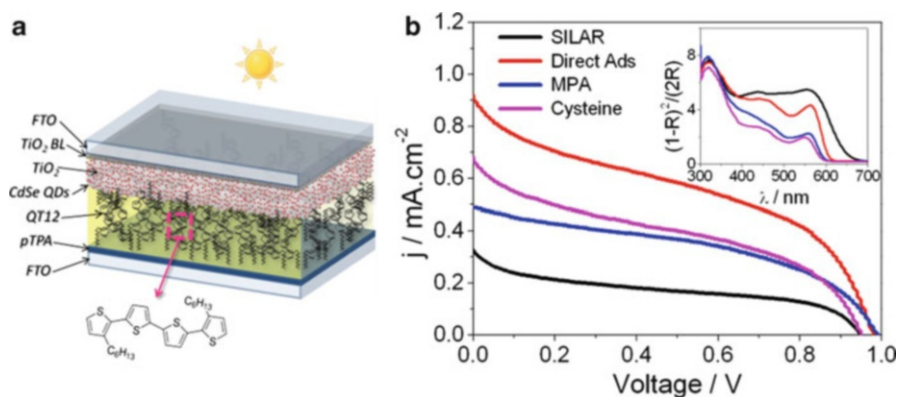
Fig. 1.6 (a) Schematic structure of the solid-state QDSSC tested by Barceló et al. (b) Current density–voltage curves of the cell with different modes of attachment. The inset presents the UV–vis diffuse reflectance spectra (transformed according to the Kubelka–Munk function) obtained for each photoanode. Adapted from [83]—reproduced by permission of the PCCP Owner Societies
