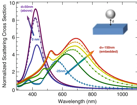
Fig. 14.14 Normalized scattering cross section of a spherical silver particle with radius of 50 nm as distance from the substrate is changed. d is the distance from the bottom of the sphere to the surface of the substrate (note that a negative d corresponds to particle partially/fully embedded within the substrate). Data is plotted as the sphere is moved in steps of 25 nm
