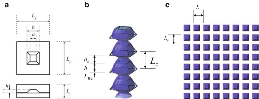
Fig. 5.2 Schematic of a single QD that is used to makes an array (a), QD truncation factor is defined as t = a/b , while all the other relevant parameters are defined in the main text. The vertically aligned 1D QD array (b) and 2D laterally aligned QD array (c)
