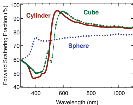
Fig. 14.12 Percentage of forward scattering as a function of wavelength corresponding to different particle shapes. There are three different shapes considered: sphere ( d = 100 nm: blue line), cylinder ( d = 100 nm, h = 100 nm: red line), and cube ( d = 100 nm: green line). In all cases, the Ag particles sit on an n = 2 dielectric substrate
