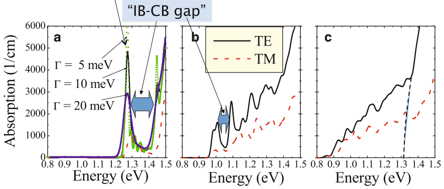
Fig. 5.4 Intraband transversal electric (TE) and transversal magnetic (TM) components of the absorption spectra of three representative QD arrays discussed in the main text, calculated with \Gamma=10 meV. TE spectra of structure (a) for \Gamma = 5, 10, 20 meV (dotted, solid, and dashed lines, respectively) demonstrate the robustness of the IB with respect to broadening. (a) QD size in array is b = 6 nm, (b) QD size in array is b = 12 nm and (c) QD size is b = 20 nm. In (c) dotted line is given for orientation and represents GaAs bulk-like absorption edge
