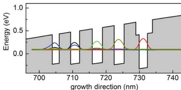
Fig. 7.16 Calculation of an idealized conduction band profile showing some delocalization of QD electron wavefunction within the QD stack
