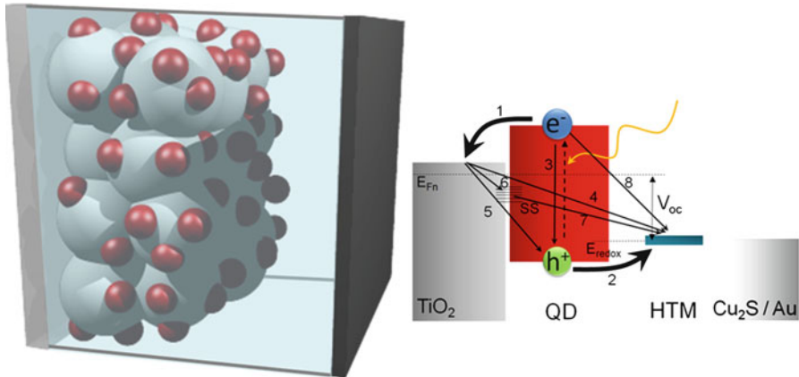
Fig. 1.2 Sketch depicting a QDSSC and the corresponding energy-band diagram illustrating the main processes: (1) electron injection; (2) hole transfer to the HTM; (3) QD band-to-band recombination; (4) recombination of \text{TiO}_2 CB electrons with the oxidized HTM; (5) back electron transfer; (6) electron trapping in interfacial states; (7) recombination of \text{TiO}_2 trapped electrons with the oxidized HTM; (8) recombination of QD CB electrons with the oxidized HTM
