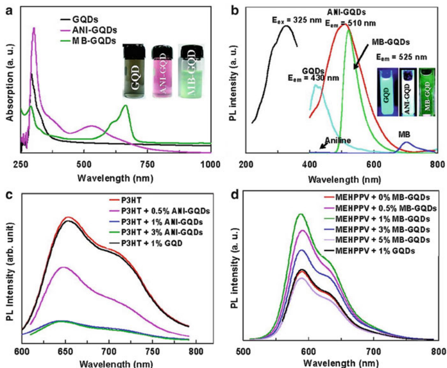
Fig. 10.6 (a) UV-vis absorption, (b) PL spectra of GQDs, ANI-GQDs, MB, Aniline, and MB-GQDs, (c) PL spectra of P3HT/ANI-GQDs, and (d) PL spectra of MEH-PPV/MB-GQDs (reprinted with permission from [21]. Copyright (2011) American Chemical Society)
