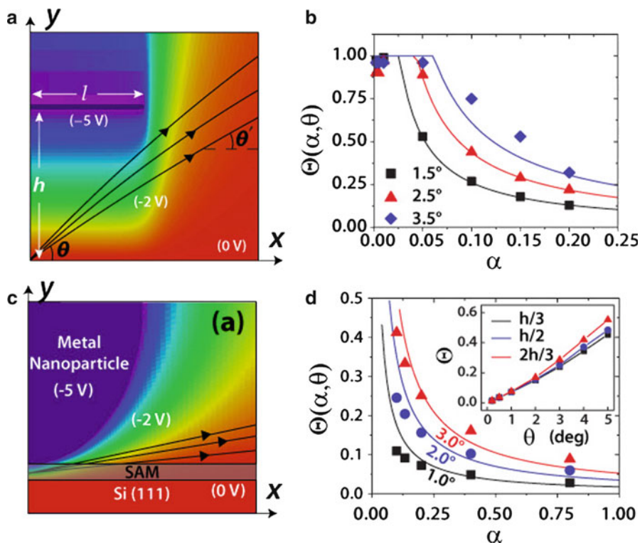
Fig. 13.22 (Color online) corrections for the boundary condition associated with finite-size geometries. (a) The calculated potential for a slab of length 2l , fixed at -5 V, a distance h from a grounded base plane. (b) The correction factor calculated for various aspect ratios, \alpha = 2h/l . Each curve represents a different launch angle, \theta_i . The solid lines are the predicted correction factors given by Eq. (13.28). (c) The calculated potential for the case of a 20 nm metallic nanoparticle, charged to -5 V, with a 1 nm thick dielectric layer ( \epsilon = 2.5 ) on the Si substrate. (d) The correction factor as a function of aspect ratio (SAM to nanoparticle) is calculated by performing ray-tracing in the field distribution described in (a). The solid symbols are the simulated data; the lines are from Eq. (13.28) using the definition of \alpha from the text. Inset: The correction factor as a function of launch angle \theta for three different launch positions along the SAM [27]
