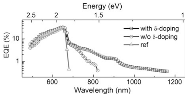
Fig. 7.9 Comparative EQE measurements of device SC-1 (w/o \delta -doping), SC-2 (w \delta -doping) and the reference sample REF (w/o QDs)
