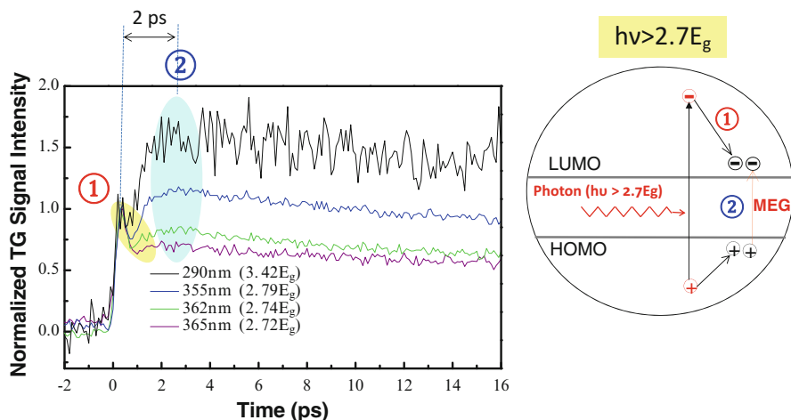
Fig. 12.10 Normalized TG kinetics for pump light wavelengths decreasing from 365 nm ( h\nu: 2.72E_g ) to 290 nm ( h\nu: 3.42E_g ), where the TG signals are normalized at the initial peaks
