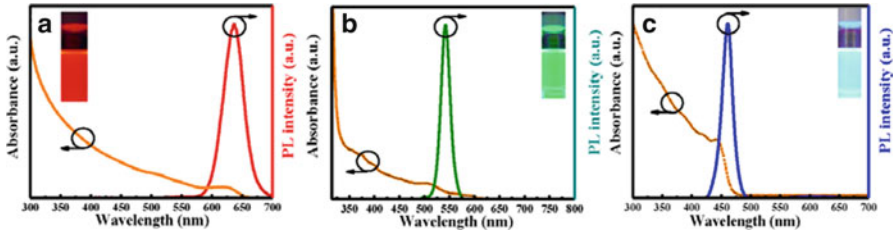
Fig. 3.3 Absorbance and photoluminescence intensity profiles for three different types of CQDs: (a) red, (b) green, and (c) blue [30]
