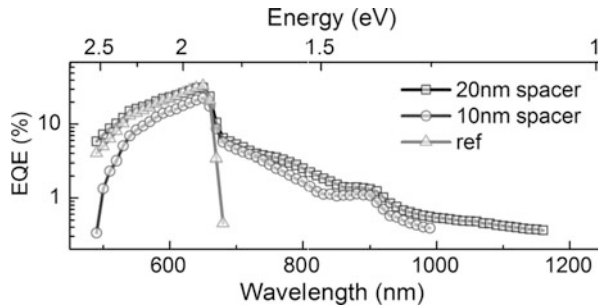
Fig. 7.12 Comparative EQE measurements of device SC-2 (20 nm spacer layers), SC-5 (10 nm spacer layers), and the reference sample REF (w/o QDs)
