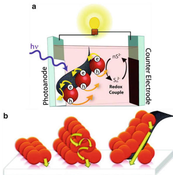
Fig. 11.7 (a) Scheme of the solar cells in which photocurrent generation occurs when CdSe QDs absorb light. (b) Three electron transfer routes from excited CdSe QDs to collecting electrode. Reprinted with permission from [39]; Copyright © 2012 The American Chemical Society
