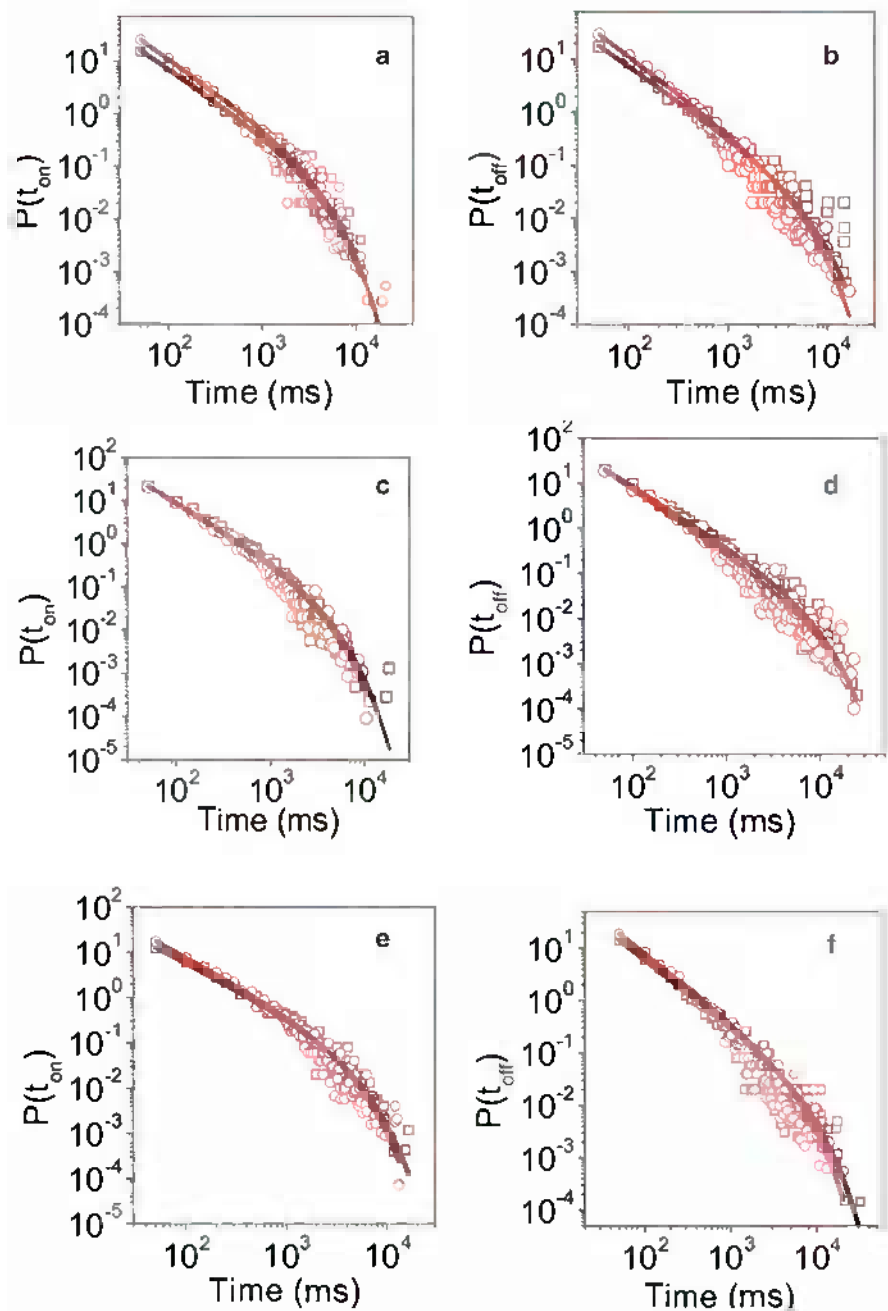
Fig. 4.11 Probability distributions P(t_{\text{on}}) , (a, c, e) and P(t_{\text{off}}) , (b, d, f) for QD-2 (a, b, black squares), FHQ/QD-2 hybrids (a, b, red dots), for QD-3 (c, d, black squares) and FHQ/QD-3 hybrids (c, d, red dots) and for QD-4 (e, f, black squares) and FHQ/QD-4 hybrids (e, f, red dots). Reproduced in part from [21]
