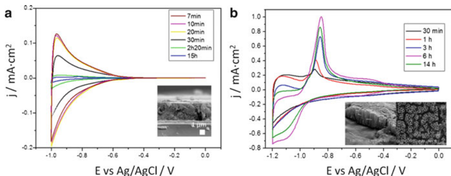
Fig. 1.10 Cyclic voltammograms for TiO 2 nanoparticulate (a) and TiO 2 nanotubes electrodes (b) after sensitization through direct adsorption of TOP-capped CdSe QDs for different adsorption times. Electrolyte: N 2 -purged 0.5 M Na 2 SO 3 . Scan rate 20 mV s -1
