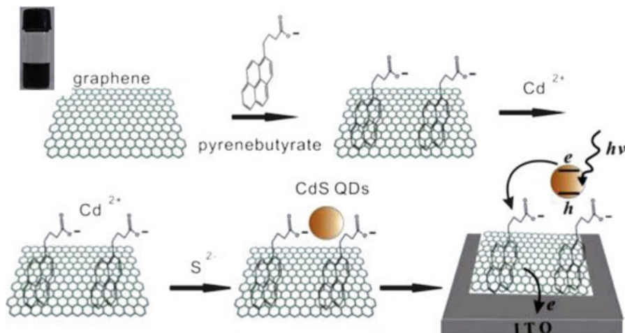
Fig. 11.3 Scheme of in situ growth of CdS QDs on graphene. Inset shows 0.5 mg mL -1 PB-graphene solution in methanol. Reprinted with permission from [40]; Copyright © 2010 Elsevier
