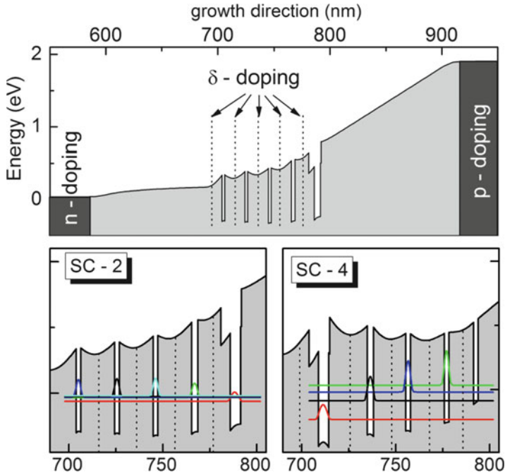
Fig. 7.15 Top : Simulated conduction band profile with n- and p-doped regions indicated with darker contrast. The QDs are located in the center of the intrinsic region. \delta -dopings are indicated as dotted lines. Bottom : Magnification of the QD region from device SC-2 (normal QD arrangement) and device SC-4 (inverted QD arrangement) and squared wave functions of the respective QDs. The QD eigenenergies in device SC-2 are nearly equi-energetic whereas the eigenenergies in SC-4 were strongly separated
