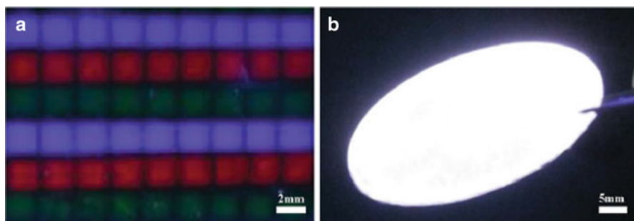
Fig. 3.15 Image of the (a) pixel pattern and (b) a 2-in. full wafer structure under UV excitation [30]
