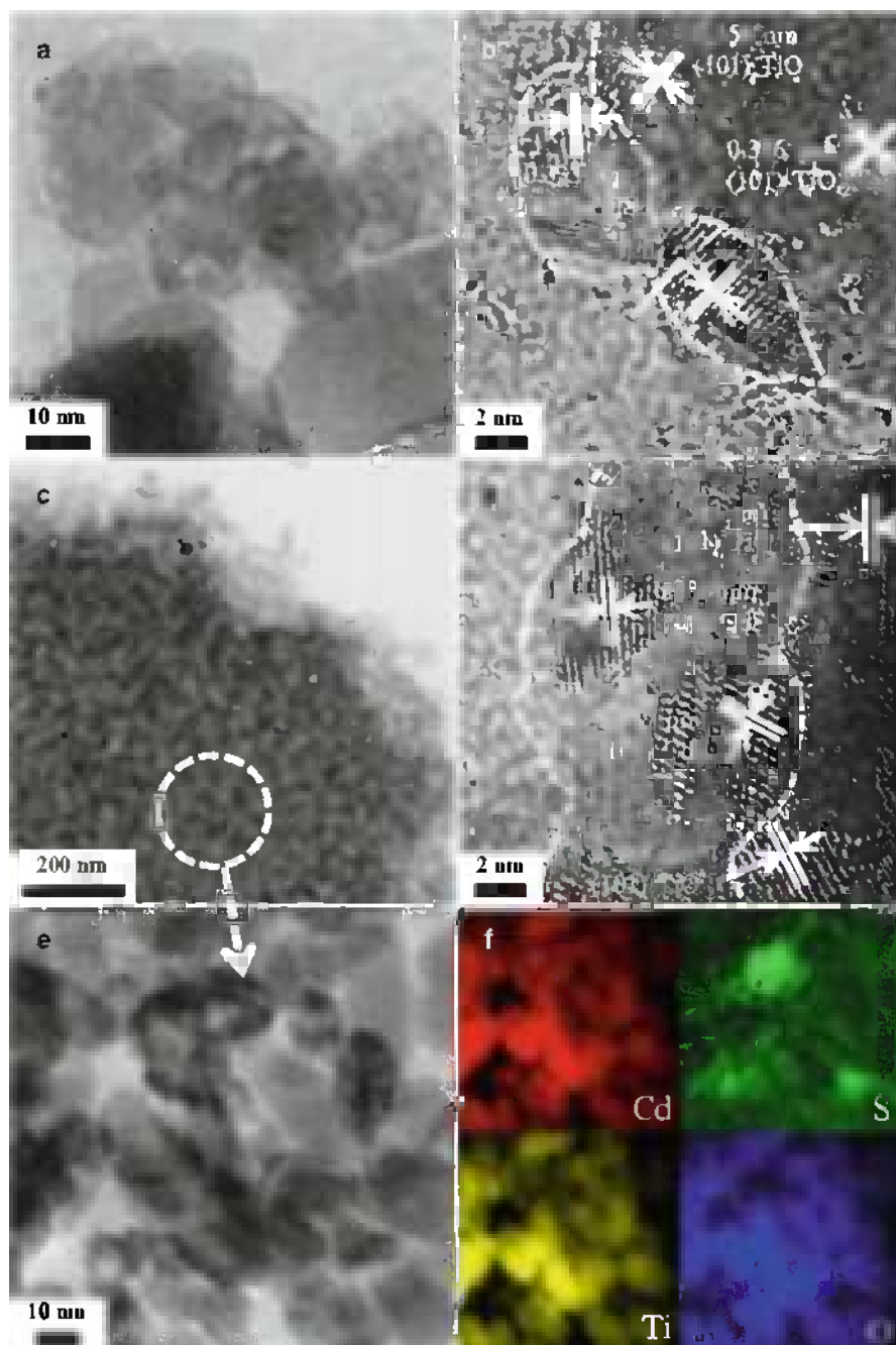
Fig. 2.12 STEM images of the CdS QD-sensitized \text{TiO}_2 particles. (a, b) T20 particles after SILAR process (c, d) A sliced MS \text{TiO}_2 particle after SILAR process (e, f) A high resolution TEM image of the sensitized MS \text{TiO}_2 particle, and corresponding EELS data
