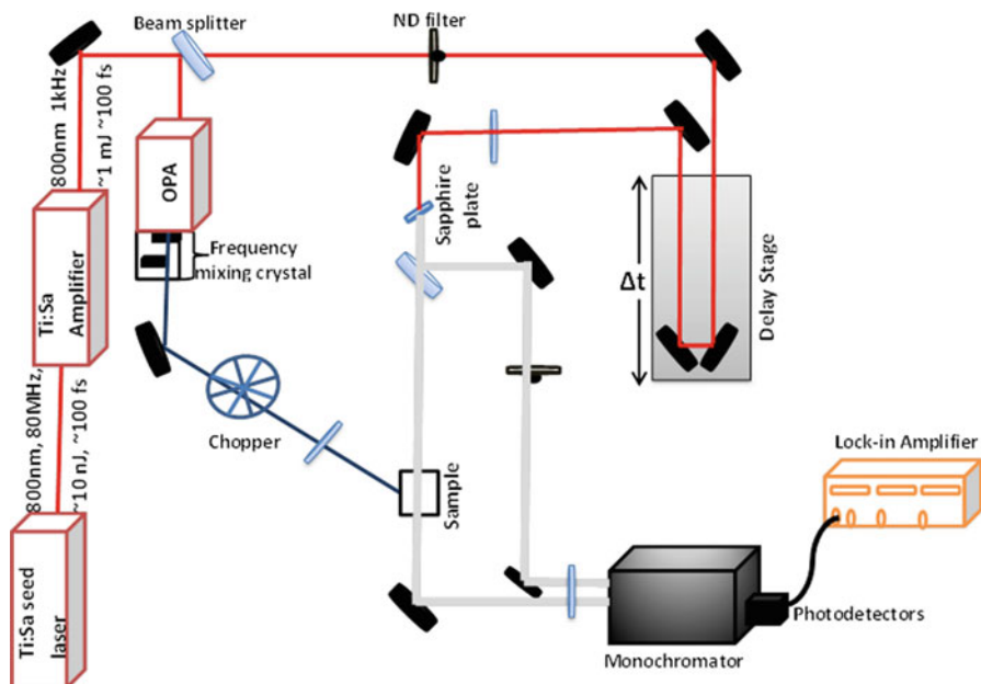
Fig. 9.3 Experimental set-up for a typical ultrafast transient absorption spectrometer
