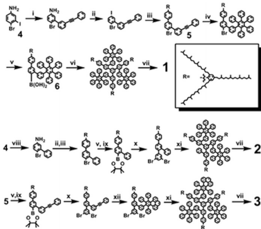
Fig. 11.9 Synthesis of GQDs via a wet chemistry approach. Reprinted with permission from [24]; Copyright © 2010 The American Chemical Society
