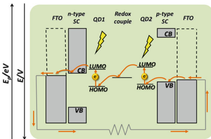
Fig. 1.8 Schematic representation of the working principle of a tandem QDSSC. SC denotes semiconductor
