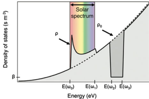
Fig. 14.24 Schematic of the spectral reweighting needed to achieve density of states enhancements over a particular bandwidth while simultaneously decreasing the density of states in another region where the density of states is unimportant for optical absorption. Adapted from [21]
