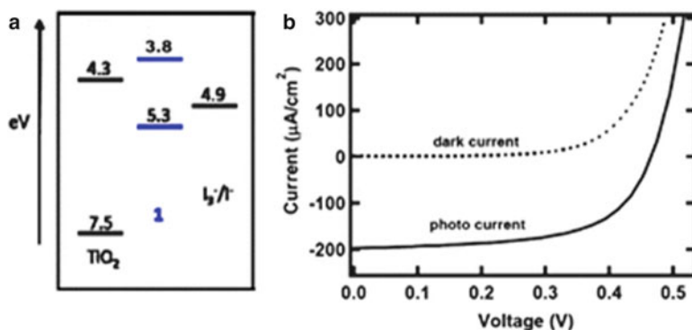
Fig. 11.12 (a) Calculated energy level alignment. (b) J - V characteristics of colloidal GQD-sensitized TiO 2 nanoparticle solar cells. Reprinted with permission from [80]; Copyright © The American Chemical Society
