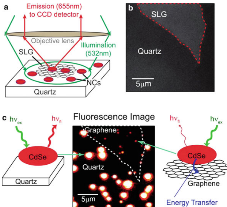
Fig. 11.1 Fluorescence images of CdSe/ZnS nanocrystals on single-layer graphene and on the quartz substrate. (a) Schematic diagram of the experimental setup; (b) optical reflectivity image in the emission range of our nanocrystals; (c) wide-field fluorescence image of individual CdSe/ZnS nanocrystals on quartz (left) and on single-layer graphene (right). Reprinted with permission from [32]; Copyright © 2010 The American Chemical Society
