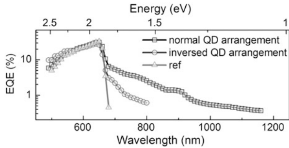
Fig. 7.11 Comparative EQE measurements of device SC-2 (normal QD arrangement), SC-4 (inverted QD arrangement) and the reference sample REF (w/o QDs)
