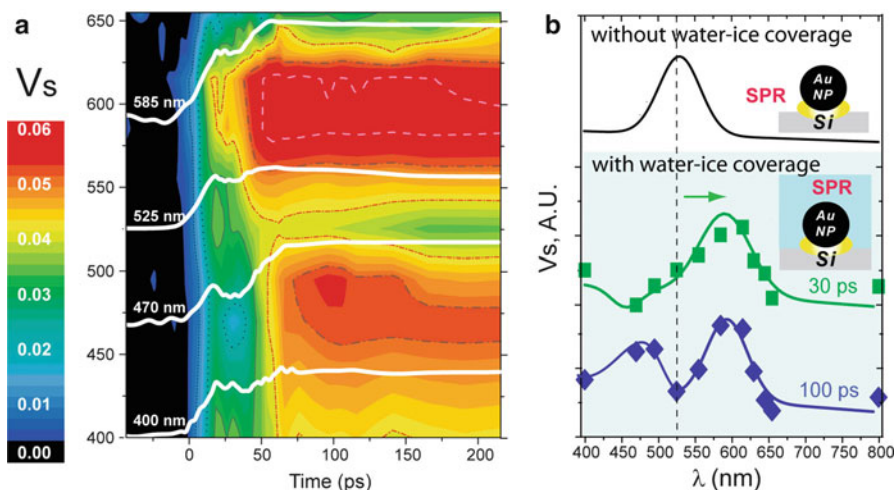
Fig. 13.14 (a) Surface photovoltage response map constructed using the diffractive voltammetry conducted on the surface of the water–ice slab dosed on the gold nanoparticle (NP)/SAM/silicon interface at excitation wavelength \lambda from 400 to 800 nm. Selected surface photovoltage curves V_s(t) at \lambda=400, 470, 525, and 585 nm show a composition of two dynamics with different timescales. (b) Comparisons between the surface voltage response spectra obtained from the interface without the coverage of water–ice ( black line ) and the ones with water–ice covers shows a red shift of the resonance peak ( green line ) at 30 ps, and bifurcation of peaks ( blue line ) at 100 ps [93]
