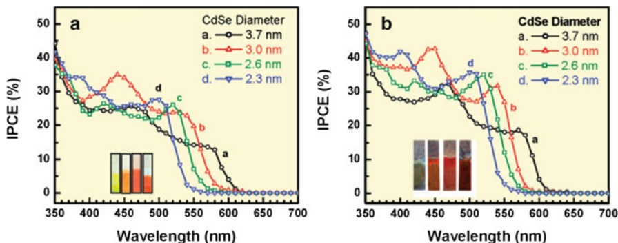
Fig. 1.4 IPCE spectra recorded for (a) OTE/TiO 2 (Nanoparticulate)/CdSe and (b) Ti/TiO 2 (Nanotubes)/CdSe electrodes, as a function of the CdSe QD diameter (a) 3.7, (b) 3.0, (c) 2.6, and (d) 2.3 nm. Reprinted with permission from [22]
