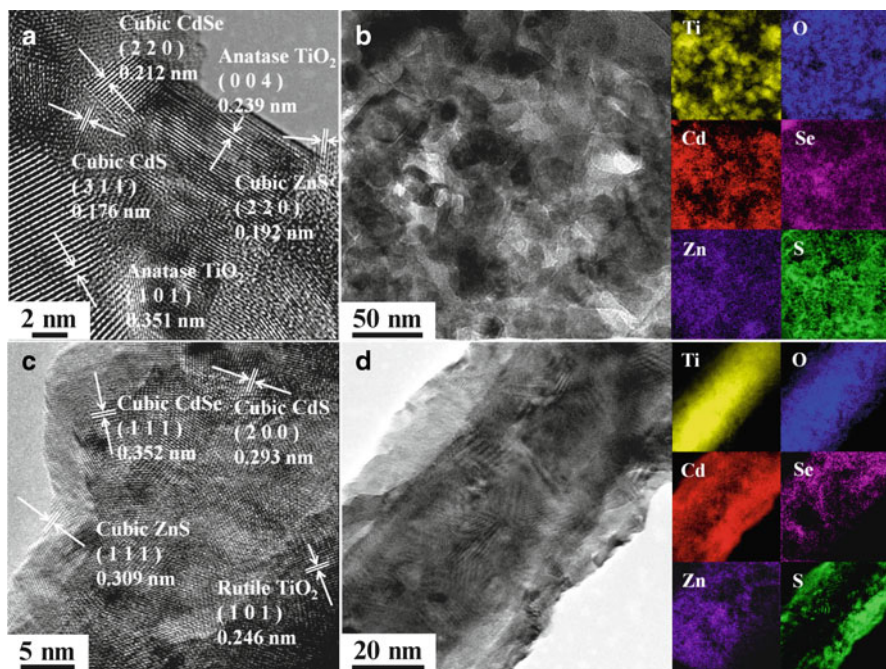
Fig. 2.22 STEM images of the CdS/CdSe/ZnS QD-sensitized \text{TiO}_2 nanocrystals. (a, b) The sensitized NP film and (c, d) SU film. Each inset compares EELS data of these two sensitized films
