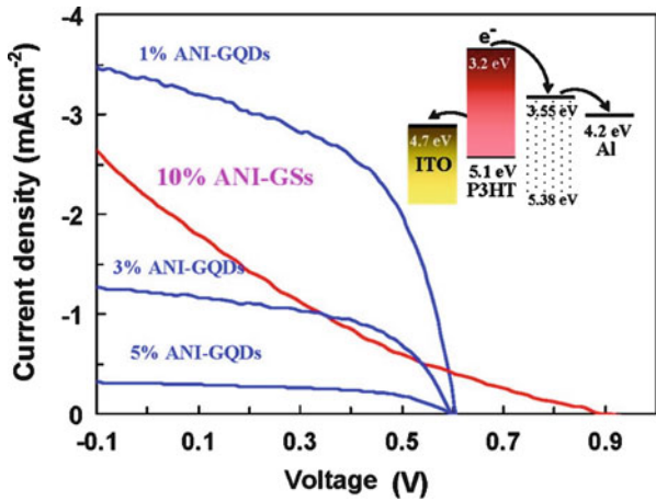
Fig. 10.7 J – V characteristics of the photovoltaic devices based on ANI-GQDs with different GQDs content and ANI-GS (under optimized condition) annealed at 160 °C for 10 min, in AM 1.5 G 100 mW illumination (reprinted with permission from [21]. Copyright (2011) American Chemical Society)
