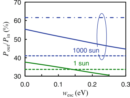
Fig. 8.18 Conversion efficiency P_{\text{out}}/P_{\text{in}} depending on the energy-selection with of the ESCs w_{\text{esc}} . \tau_{\text{eq}} (ps) = 10 w_{\text{esc}} (eV), \tau_{\text{th}} = 1 ns. \varepsilon_g , E_{\text{esc}} and other parameters are optimized for each case. Broken lines and a dashed-dotted line are the results for 1J- and 3J-SCs, respectively. Reprinted with permission from [43]. © 2010, The Japan Society of Applied Physics
