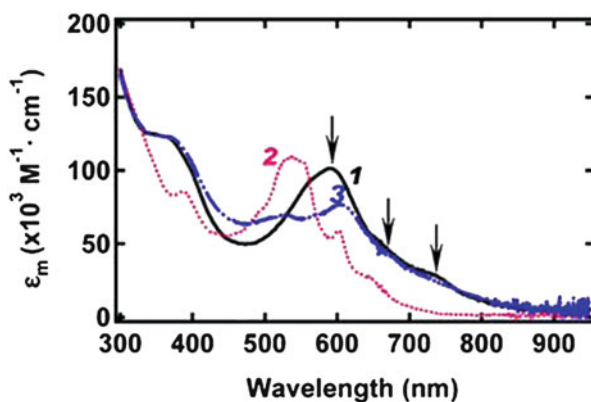
Fig. 11.10 UV-vis absorption of colloidal GQDs. \alpha , p , and \beta bands of GQDs with 168 conjugated carbon atoms are marked by arrows (i.e., 1 in Figs. 11.8a and 11.9), from right to left, respectively. Reprinted with permission from [24]; Copyright © 2010 The American Chemical Society
