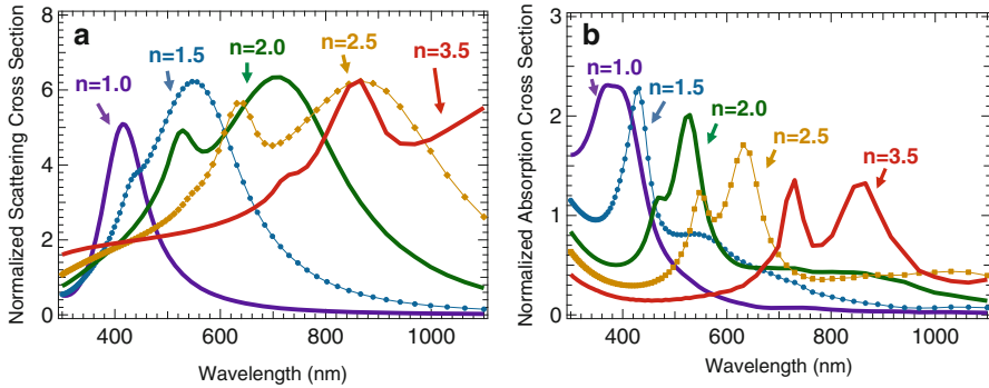
Fig. 14.10 Normalized scattering (a) and absorption (b) cross sections change with refractive index: n = 1 (air), n = 1.5 (e.g., \text{SiO}_2 ), n = 2 (e.g., \text{Si}_3\text{N}_4 ), n = 2.5 (e.g., \text{TiO}_2 ), and n = 3.5 (e.g., GaAs). The silver scattering particle has a radius of 50 nm
