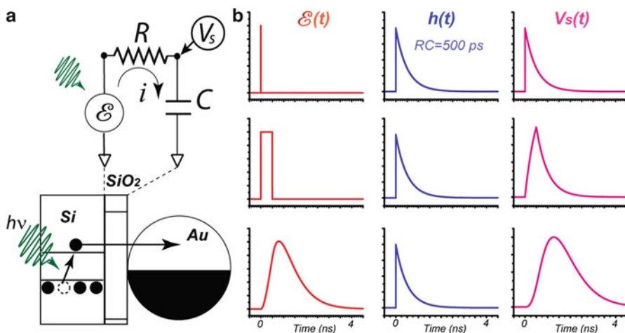
Fig. 13.16 (a) An effective circuit model depicting the transient surface voltage V_s(t) measurement via the refraction shift across the \text{SiO}_2 slab at \text{SiO}_2/\text{Si} interface. The electromotive potential \mathcal{E}(t) comes from the hot carriers generated at the Si substrate. (b) Examples showing the photovoltage V_s(t) measured at the interface as a function of \mathcal{E}(t) . The relationship can be seen as a convolution with kernel function h(t) characteristic of the RC circuit
