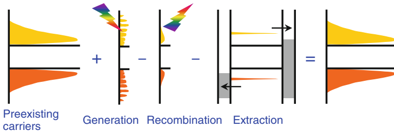
Fig. 8.4 Balance of particle and energy fluxes in a steady-state operation. Energy dissipation due to thermalization is excluded for simplification
