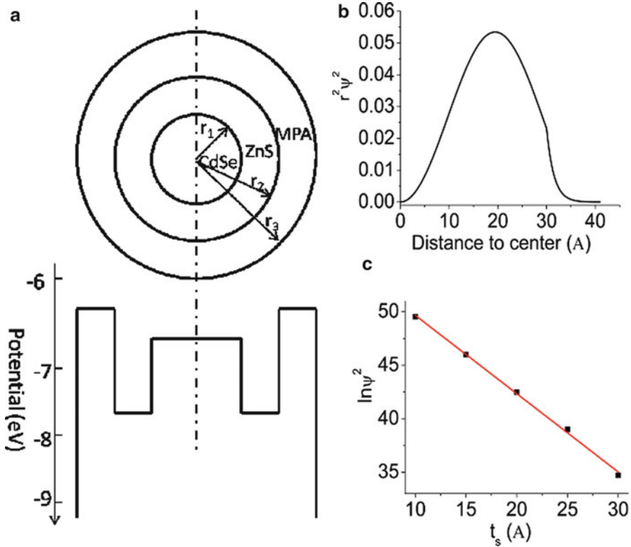
Fig. 4.7 (a) Schematic representation of the valence band alignment at the core/shell/ligand (CdSe/ZnS/MPA) quantum dot structure; (b) radial probability function of 1S hole wave function in CdSe/ZnS QD with shell thickness of 12 Å; (c) hole wave function density at ZnS surface vs ZnS shell thickness
