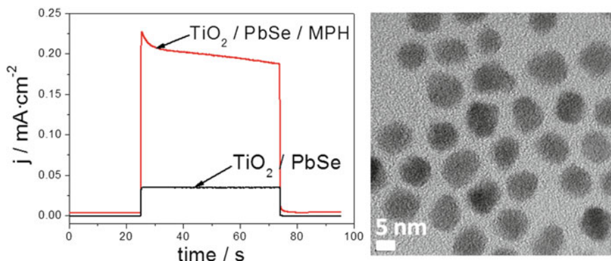
Fig. 1.13 Photocurrent transients recorded for PbSe-sensitized electrodes before and after modification with p-mercaptophenol (MPH). Measurements were done in a three-electrode cell using an Ag/AgCl/KCl (sat.) reference electrode and a Pt wire as a counter-electrode. An N 2 -purged aqueous 0.5 M Na 2 SO 3 was employed as electrolyte. Illumination was allowed only in the 380–1,100 nm range, with an irradiance of 50 mW cm -2 . A TEM image of the PbSe QDs is also included
