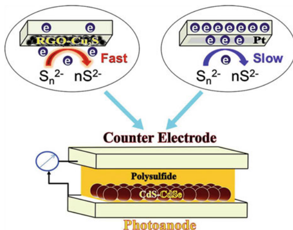
Fig. 11.6 Scheme of a QDSSC with the comparison of the kinetics of redox reaction at two different counter electrodes. Reprinted with permission from [9]; Copyright © 2011 The American Chemical Society
