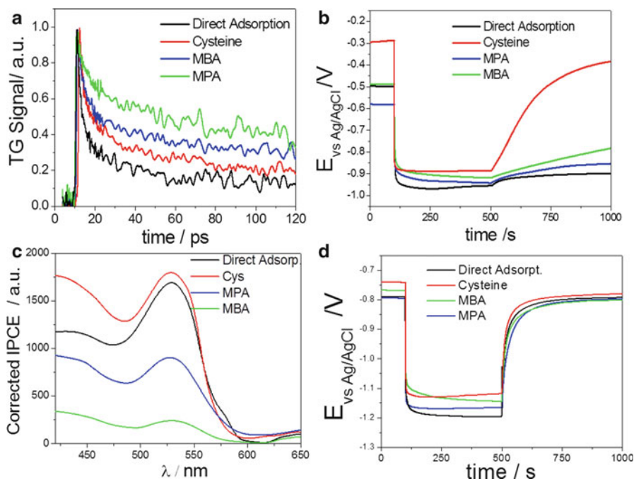
Fig. 1.12 (a) Transient grating responses for CdSe-sensitized TiO 2 electrodes using direct adsorption and cysteine, mercaptopropionic acid (MPA) and mercaptobenzoic acid (MBA) as linkers. All the curves are normalized to the maximum value. In this case a faster decay corresponds to a faster electron injection. (c) Corrected IPCE spectra, considering the light absorption, for TiO 2 /CdSe QDs in N 2 -purged aqueous 0.5 M Na 2 SO 3 . (b and d) Photopotential measurements obtained for transient illumination of electrodes sensitized with colloidal QDs in the absence (b, N 2 -purged aqueous 0.5 M Na 2 SO 3 ) and in the presence of an electron scavenger (c, 0.1 M S + 1 M Na 2 S + 1 M NaOH). In this case, a larger photopotential value corresponds to a larger electron accumulation, while a faster decay corresponds to a faster electron recombination rate. Adapted with permission from [44]
