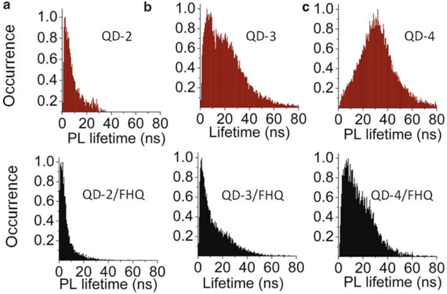
Fig. 4.9 Distributions of PL lifetimes for isolated QDs on surface (red, upper panels) and isolated FHQ/QD hybrids (black, lower panels) on glass surface: (a) QD-2 and FHQ/QD-2; (b) QD3 and FHQ/QD-3; (c) QD4 and FHQ/QD-4. Reproduced in part from [23]
