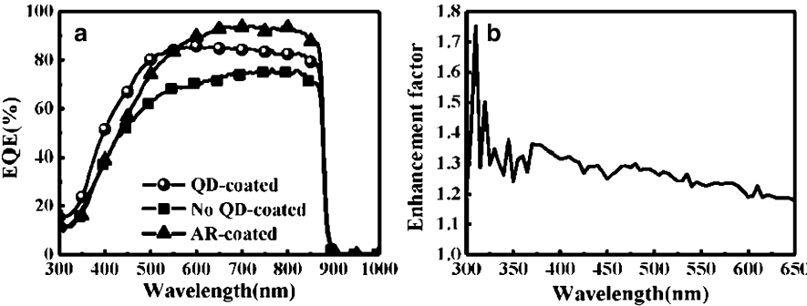
Fig. 3.11 (a) Measurement of external quantum efficiency of GaAs + CQD, GaAs only (No CQD), and GaAs + AR coating solar cells. (b) Enhancement of EQE between GaAs + CQD and GaAs only device. Peak at \sim 310 nm indicates photon down-conversion [49]
