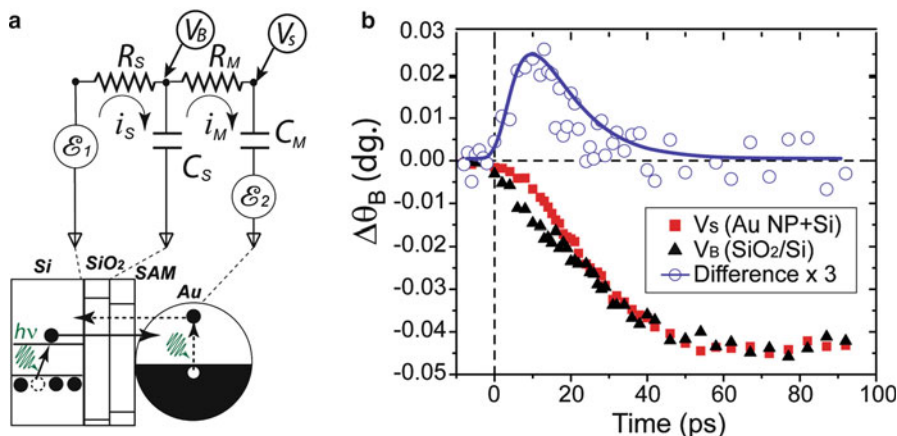
Fig. 13.11 (a) An effective circuit model depicting the transient surface voltage V_s(t) measurement via the refraction shift of the diffracted beams through SAM. The R_s , C_s , R_m , C_m are the effective resistance and capacitance of the substrate (S) and the SAM (M). The electromotive potential that can drive the photocurrent through the \text{SiO}_2 layer ( i_s ) and further through SAM ( i_m ) is mainly from the hot carriers generated from the Si ( \mathcal{E}_1(t) ); whereas the short-lived photoexcited hot carriers generated within the Au nanoparticle (NP) can also drive the charge transfer in the opposite direction ( \mathcal{E}_2(t) ). (b) The overall refraction shift determined by SAM diffracted beam (labeled V_s ), the background (labeled V_B ) obtained from \text{SiO}_2/\text{Si} interface, and the molecular charge transport contribution, obtained by subtracting V_B from V_s
