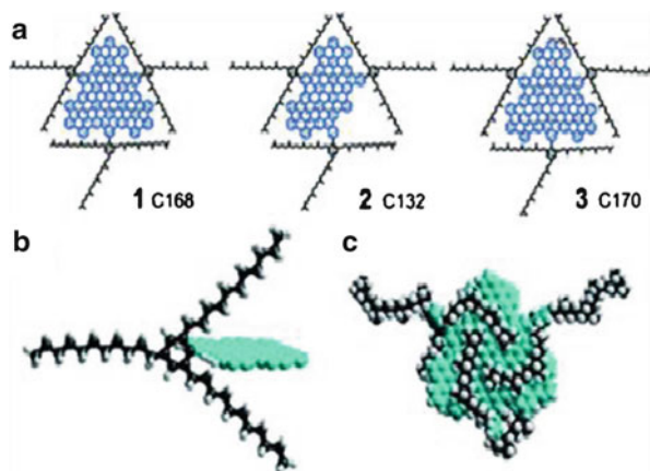
Fig. 11.8 (a) Schemes of GQDs with tunable size. (b, c) Strategies to make GQDs soluble. Reprinted with permission from [24, 80]; Copyright © 2010 The American Chemical Society
