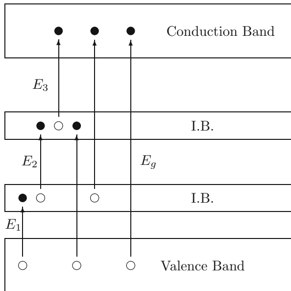
Fig. 6.2 This 4-Band diagram depicts two intermediate bands and shows the possible electronic transitions (reverse transitions are not shown but do occur). There is a total of six upward transitions, with E_1 , E_2 , and E_3 making up the three independent ones. The large energy gap, E_g , is the normal gap between the conduction and valence bands. For the purposes of this chapter, we make the assumption that E_1 \leq E_2 \leq E_3
