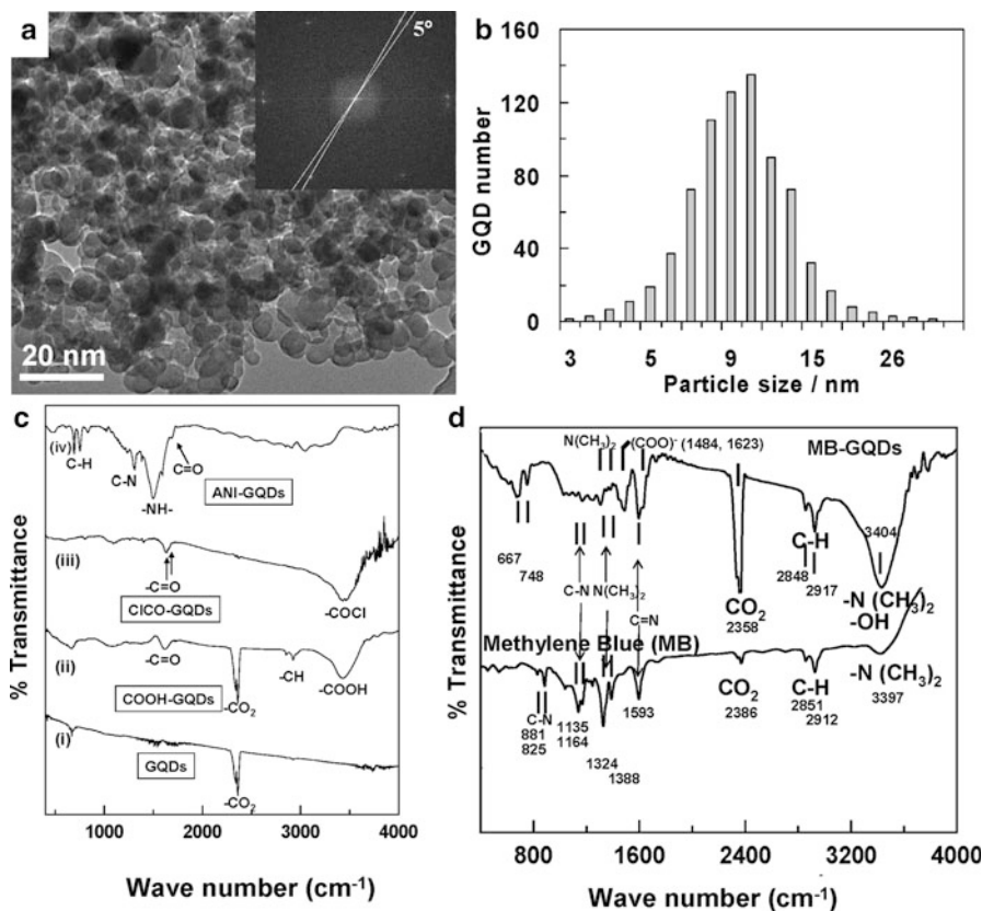
Fig. 10.5 (a) TEM image, (b) diameter distribution, and (c, d) FTIR spectra of the GQDs (reprinted with permission from [21]. Copyright (2011) American Chemical Society)
