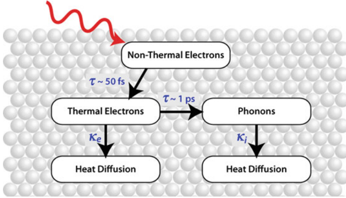
Fig. 13.19 The energy coupling scheme assumed by the TTM. First, the laser pulse is absorbed by the free electrons in the metal, which evolve into a Fermi–Dirac distribution in the first \approx 50 fs. The thermal electrons dump energy into the lattice, causing them to equilibrate after \approx 1 ps (depending on the metal). Both electrons and lattice undergo thermal losses from heat diffusion, the rates of which are largely governed by the thermal conductivity, \kappa (and strictly speaking the heat capacity and sound speed too) [33]
