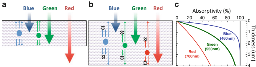
Fig. 14.2 Schematic of absorption depth and carrier collection for different wavelengths of incident light and film thicknesses. (a) A thin slab efficiently collects generated carriers; however, long wavelength photons are not absorbed resulting in reduced current. (b) A thick device absorbs nearly all of the light; however, the long path for collection increases the likelihood of carrier recombination without collection. (c) Absorption profile for different wavelengths of light
