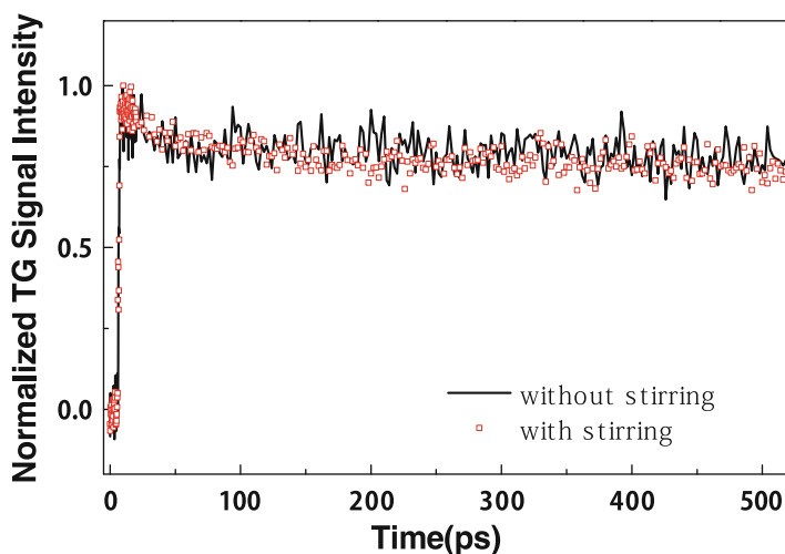
Fig. 12.8 Normalized TG kinetics of the PbS QDs for the wavelength of 360 nm ( h\nu : 2.83E_g ) measured with stirring and without stirring the PbS QD solution
