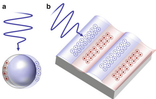
Fig. 14.7 Excitation of surface plasmons. (a) The incident light is coupled to the free electrons in a metal nanoparticle resulting in excitation of a localized surface plasmon resonance. (b) When light is incident on a planar structure, the coupling results in a propagating surface wave called a surface plasmon polariton. The circles with “-” and “+” represent separated charges
