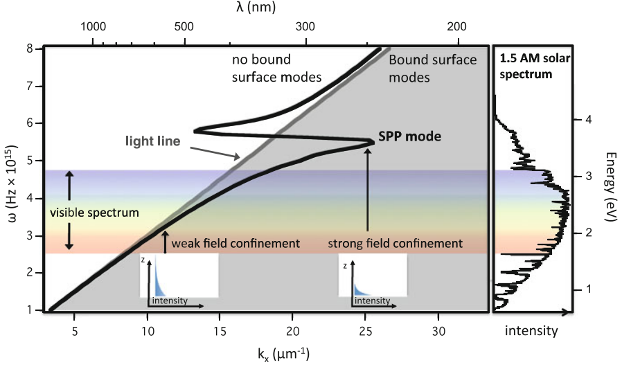
Fig. 14.17 Dispersion relation for the surface plasmon polariton mode at the silver/air interface. A significant fraction of the solar spectrum overlaps with the surface plasmon mode. Figure adapted from [9]
