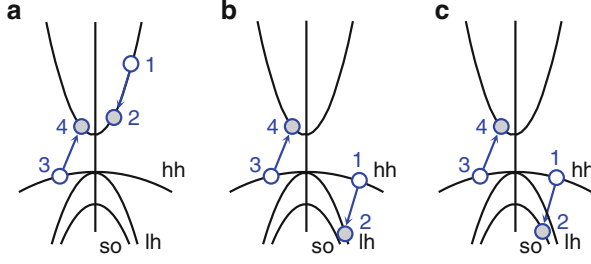
Fig. 8.16 Three major processes of impact ionization in the absorber: (a) CCCH, (b) CHHL, (c) CHHS. Note that all the circles represent electrons (not holes) in the valence bands and conduction bands. Reprinted with permission from [23]. © 2009, Elsevier B.V.
