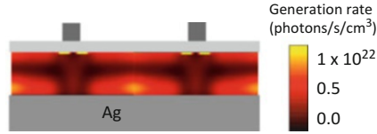
Fig. 14.18 Spatial variation of the generation rate of carriers within a semiconductor. Regions with high field intensities lead to large generation rates
