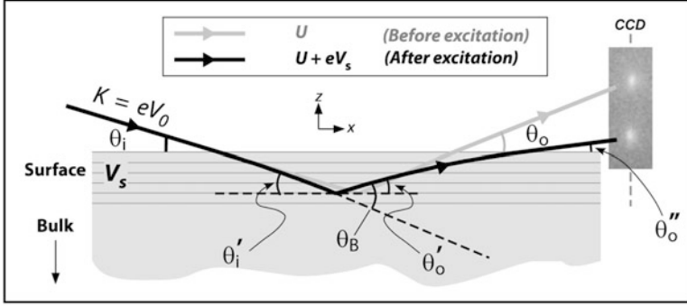
Fig. 13.3 The idealized slab model for considering the transient surface voltage. The top trajectory is the electron scattering from the crystal planes with the presence of a surface field. The electron beam, incident at \theta_i , is Bragg scattered at \theta_B , exiting the surface at \theta_o . Introducing an attractive surface potential V_s will cause the electron beam to be “refracted” deeper into the crystal ( \theta'_i ) and the same for the Bragg diffracted beam that would ultimately exit the crystal at \theta''_o with a net shift \Delta_B relative to \theta_o . Note here the shift is highly exaggerated for getting the point through [33]
