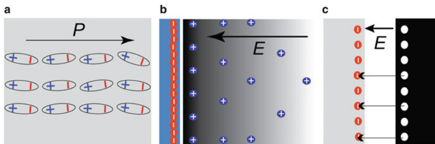
Fig. 13.1 Charge redistribution at nanomaterials' interfaces subject to photoexcitation. (a) Dielectric realignment; (b) carrier diffusion; (c) interfacial charge transfer
