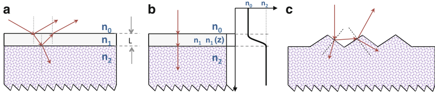
Fig. 14.4 Typical antireflection techniques for macroscopic solar cells: (a) destructive interference of reflected plane waves, (b) graded-index structures (where n_2 > n_1 > n_0 ), (c) pyramidal surface texturing
