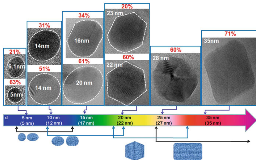
Fig. 10.1 HRTEM images of GQDs for their major shapes and corresponding populations ( p ) with increasing average size of GQDs. Here, the dotted line indicates the region of a GQD and p is defined as the ratio of number of GQDs with a major shape at each average size. Average sizes ( d_a ) of GQDs estimated from the HRTEM images at each d are indicated in the parentheses at the bottom of this figure. The connected arrows indicate the range of the average size in which GQDs with particular major shapes are found (reprinted with permission from [23]. Copyright (2012) American Chemical Society)
