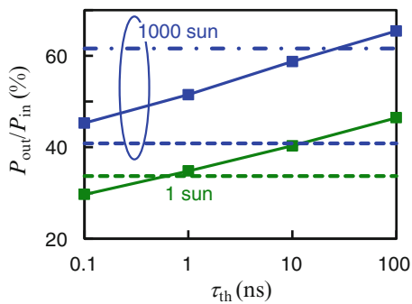
Fig. 8.21 Conversion efficiency P_{\text{out}}/P_{\text{in}} depending on the carrier thermalization time \tau_{\text{th}} . \tau_{\text{eq}} = \tau_{\text{th}}/1,000 , w_{\text{esc}} = 0.1 eV. \varepsilon_{\text{g}} , E_{\text{esc}} and other parameters are optimized for each case. Broken lines and a dashed-dotted line are the results for 1J- and 3J-SCs, respectively
