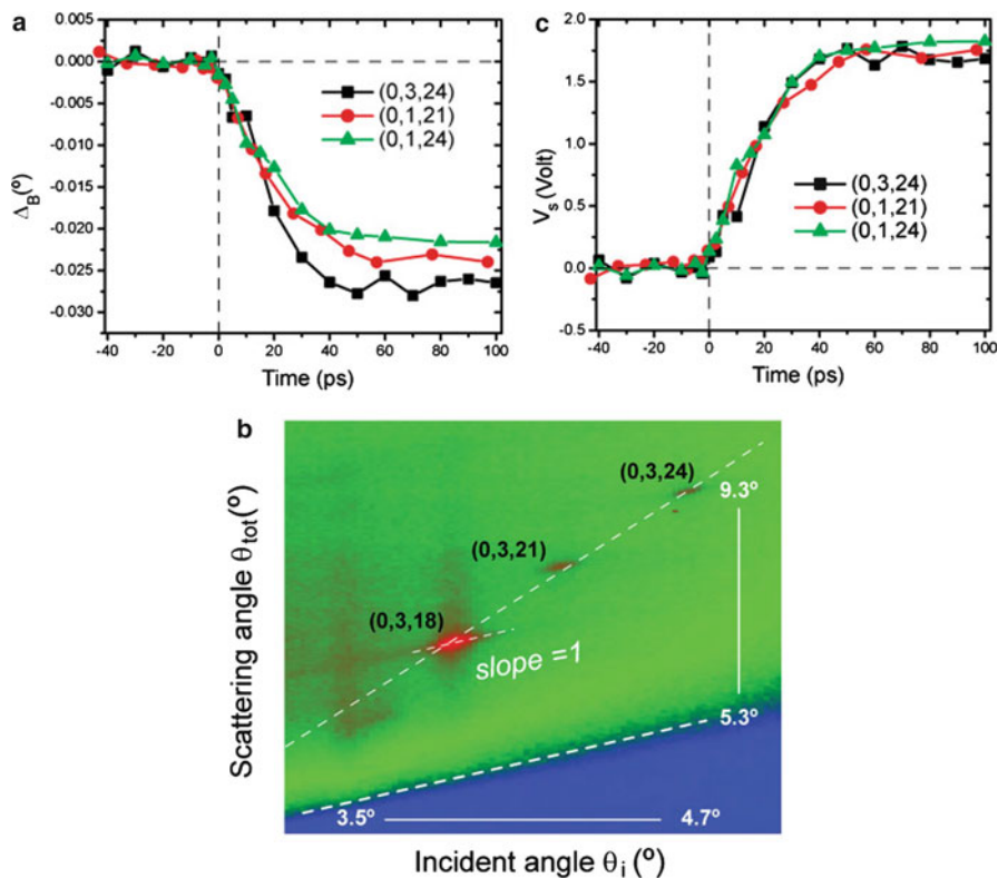
Fig. 13.7 Transient voltammetry from three diffracted beams from Si/SiO 2 interface. (a) The angular shift of (0,3,24), (0,1,21), and (0,1,24) beams excited at F = 65 \text{ mJ/cm}^2 . (b) The rocking map characterization of (0,3)-relrod, showing a surface diffraction condition a = 1 . (c) The photovoltage deduced from (0,3,24), (0,1,21), and (0,1,24) beams based on Eq. (13.8) using a = 1 [27]
