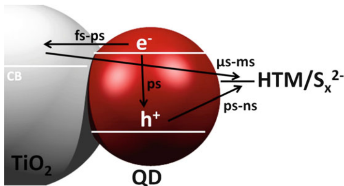
Fig. 1.9 Representation of a QD adsorbed on \text{TiO}_2 and the approximate time scales for electron and hole transfer processes
