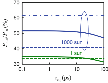
Fig. 8.19 Conversion efficiency P_{\text{out}}/P_{\text{in}} depending on the carrier equilibration time \tau_{\text{eq}} . \tau_{\text{th}} = 1 ns, w_{\text{esc}} = 0.1 eV. \varepsilon_g , E_{\text{esc}} and other parameters are optimized for each case. Broken lines and a dashed-dotted line are the results for 1J- and 3J-SCs, respectively. Reprinted with permission from [43]. © 2010, The Japan Society of Applied Physics
