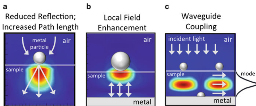
Fig. 14.6 Plasmonic nanoparticles can improve photovoltaics by (a) reducing reflection and increasing path length, (b) creating high local fields, or (c) coupling incident light into waveguide modes of the structure. Background shows the relative E-field intensity for the different situations
