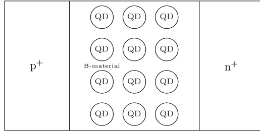
Fig. 6.7 A schematic of the proposed QD-IBSC with the barrier material surrounding the QDs. The QD material is arranged periodically within the barrier material and sandwiched in between the normal p–n junction. Reprinted with permission from [20]. Copyright 2010, American Institute of Physics
