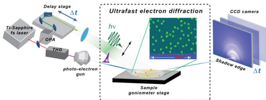
Fig. 13.2 The setup of ultrafast electron diffraction experiment used to measurement the surface voltages of nanoparticles and interfaces
