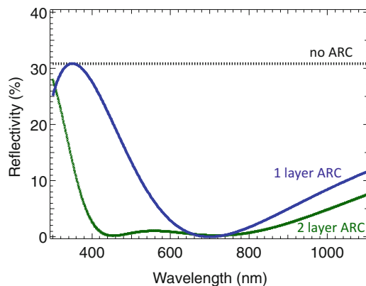
Fig. 14.5 Reflectivity as a function of wavelength from a surface with n_2 = 3.5 using no ARC, a single-layer ARC, and a double-layer ARC optimized for \lambda = 700 nm
