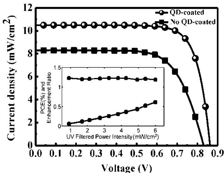
Fig. 3.12 IV measurement with UV light. The inset is the filtered UV PCE of the CQD/GaAs cell (bottom line with a slope) and the efficiency enhancement ( \eta_{\text{CQD}}/\eta_{\text{no CQD}} , top line) [49]
