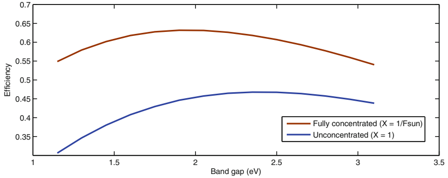
Fig. 6.3 Limiting efficiency of the IBSC with one intermediate band as a function of the largest band gap E_g for unconcentrated light X = 1 and fully concentrated light X = 1/F_{\text{sun}} . The efficiency was calculated assuming the sun is modeled as a blackbody with characteristic temperature 6,000 K. For fully concentrated light, the maximum efficiency of about 63.2 % occurs approximately at a band gap of E_g = 1.93 eV, while unconcentrated light leads to a maximum efficiency of about 46.8 % with a band gap of E_g = 2.40 eV
