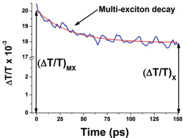
Fig. 9.4 A typical transmittance transient obtained from an ultrafast transient absorption experiment showing the decay of multi-excitons to single excitons in QDs. The MEG quantum yield can be determined from the ratio of the fractional transmittance change before [(\Delta T/T)_{MX}] and after [(\Delta T/T)_X] the decay
