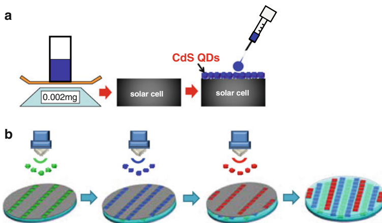
Fig. 3.4 Two different methods for CQD dispense on the device: (a) manual dispense by pipette (b) pulsed spray method
