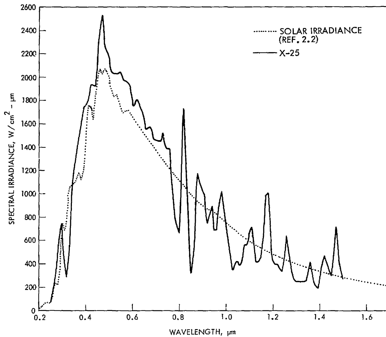
Figure 2.1 Spectral Output, Spectrolab X-25 Spectrosun 2.3
