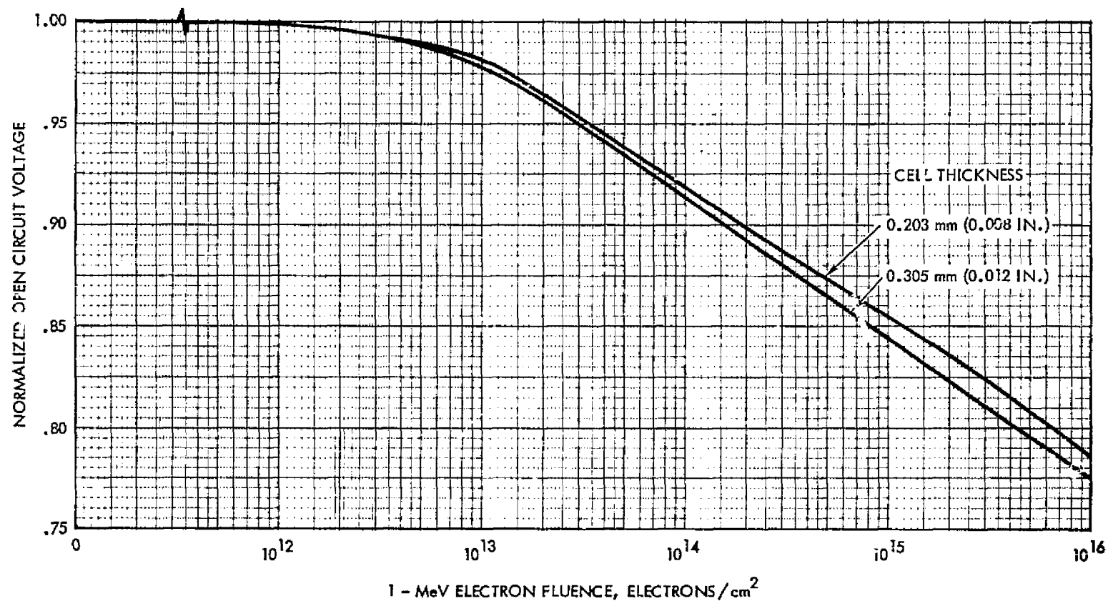
Figure-3.87 Normalized Open Circuit Voltage vs 1 MeV Electron Fluence for 20 Ohm-cm n/p Back Surface Field Silicon Cells. At 135.3 mW/cm 2 AMO Illumination, 30°C
