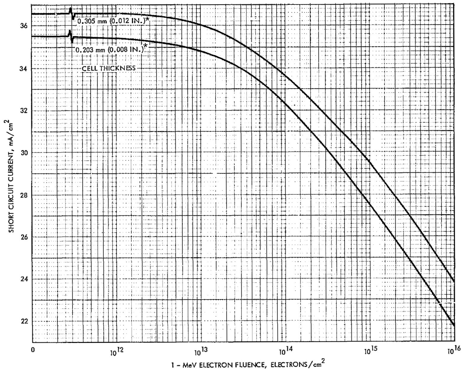
Figure 3.41 Short Circuit Current vs 1 MeV Electron Fluence for 2 Ohm-cm n/p Shallow Junction Silicon Cells. At 135.3 mW/cm 2 AMO Illumination, 30°C
