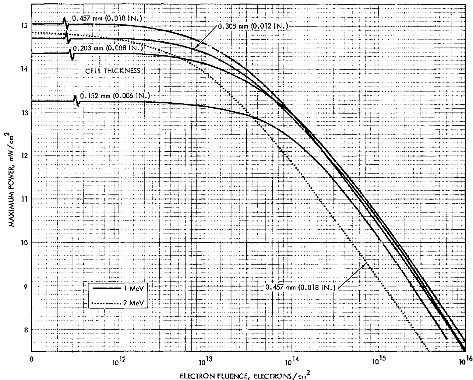
Figure 3.23 Maximum Power vs 1 MeV Electron Fluence for 2 Ohm-cm n/p Conventional Silicon Cells. At 135.3 \text{ mW}/\text{cm}^2 AMO Illumination, 30^\circ\text{C}
