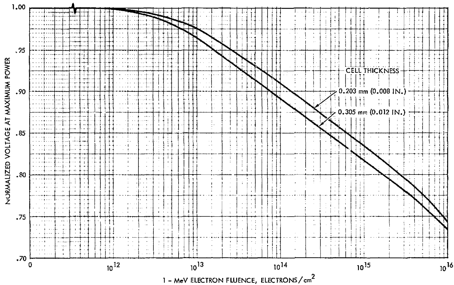
Figure 3.79 Normalized Voltage at Maximum Power vs 1 MeV Electron Fluence for 10 Ohm-cm n/p Back Surface Field Silicon Cells. At 135.3 mW/cm 2 AM0 Illumination, 30°C
