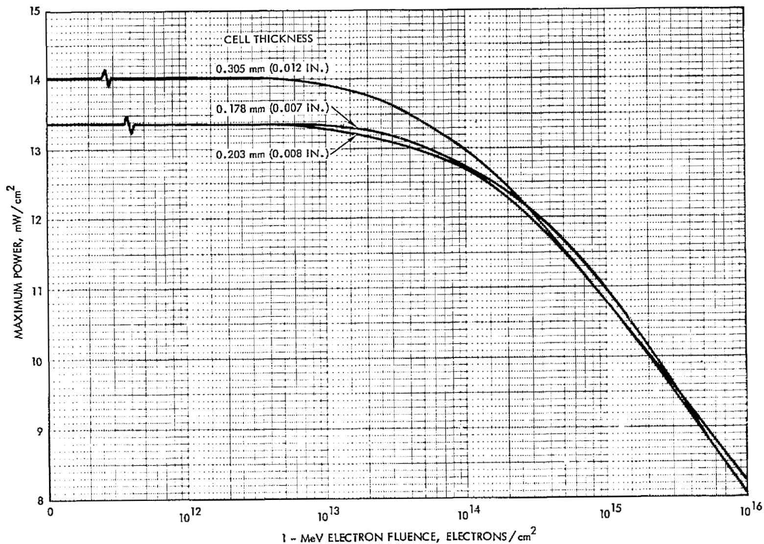
Figure 3.33 Maximum Power vs 1 MeV Electron Fluence for 10 Ohm-cm n/p Conventional Silicon Cells. At 135.3 \text{ mW}/\text{cm}^2 AMO Illumination, 30^\circ\text{C}
