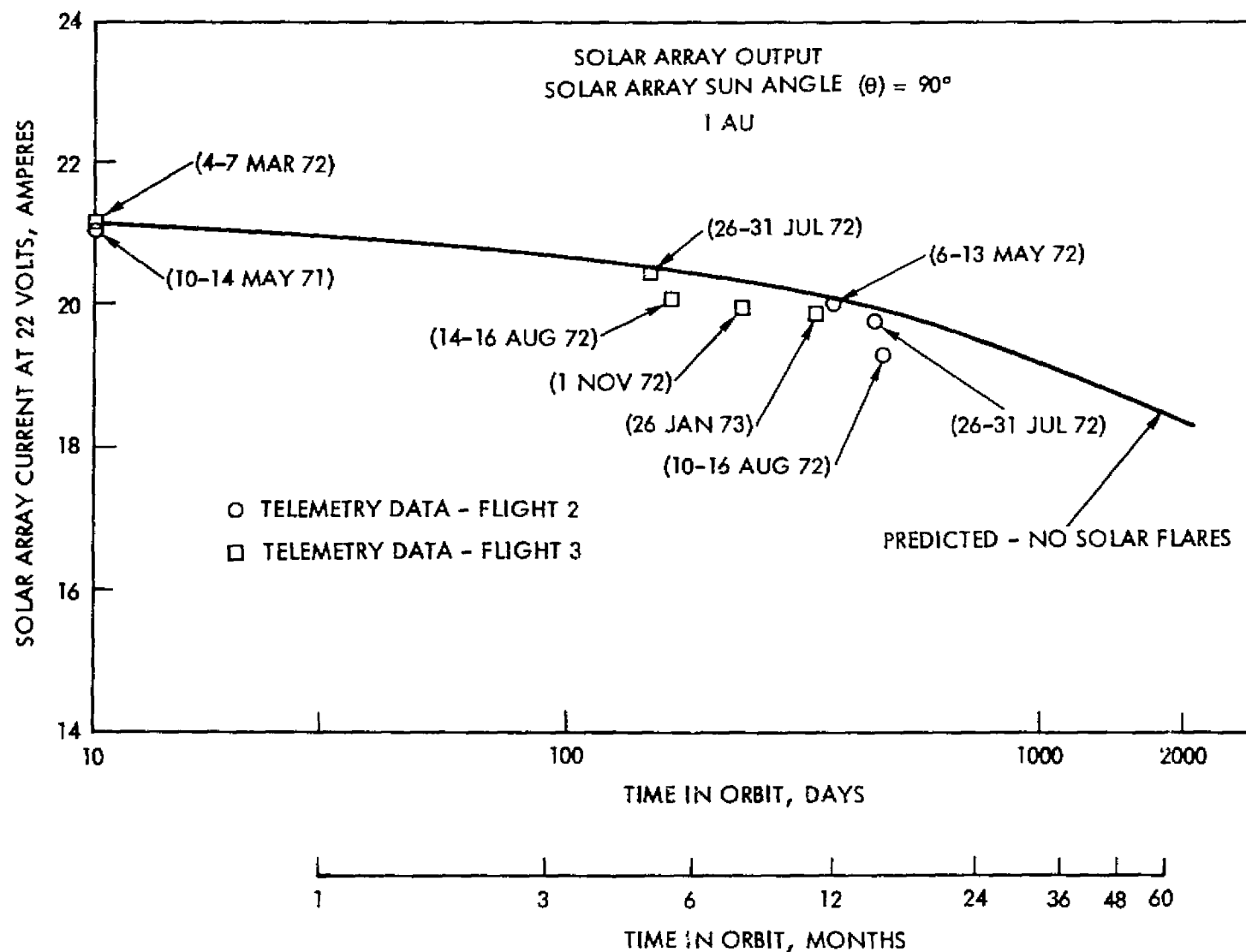
Figure 7.1 Performance of Two Satellite Solar Arrays in Synchronous Orbit During the August 1972 Solar Flares
