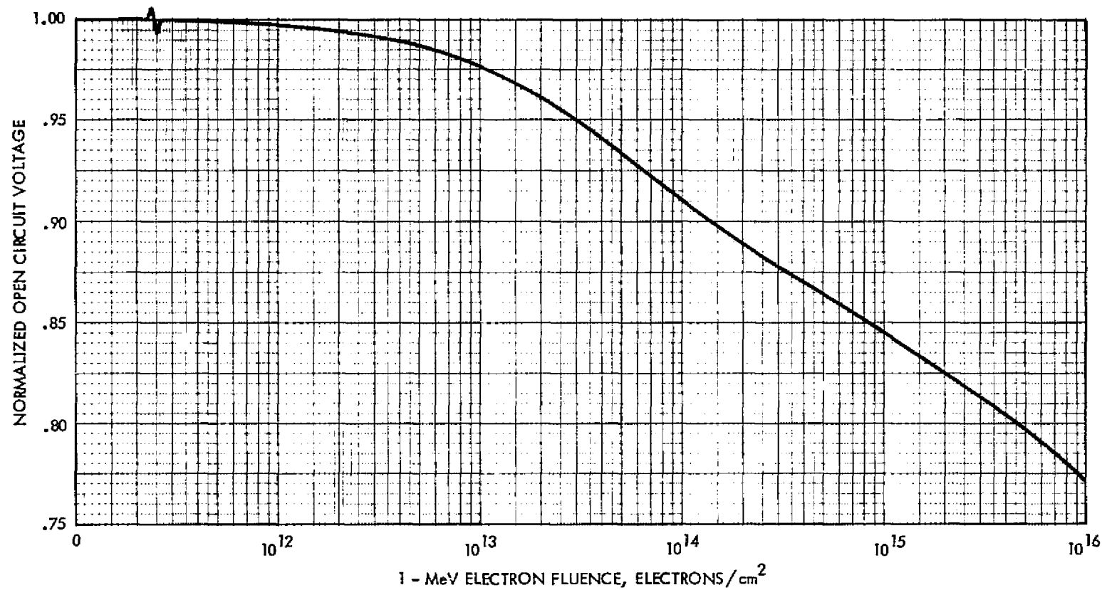
Figure 3.117 Normalized Open Circuit Voltage vs 1 MeV Electron Fluence for 10 Ohm-cm n/p Textured with Back Surface Field Silicon Cells. At 135.3 mW/cm 2 AMO Illumination, 30°C
