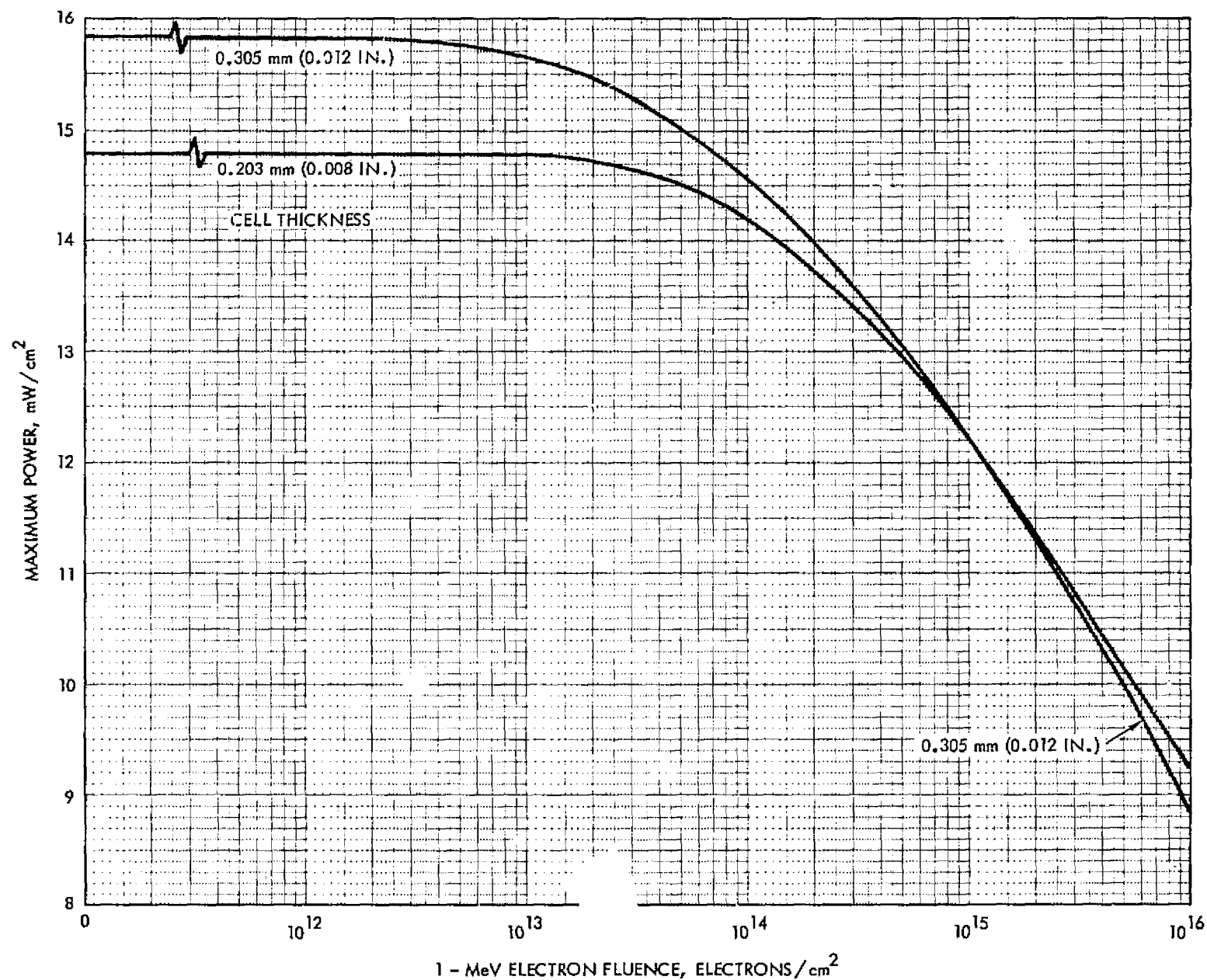
Figure 3.53 Maximum Power vs 1 MeV Electron Fluence for 10 Ohm-cm n/p Shallow Junction Silicon Cells. At 135.3 \text{ mW}/\text{cm}^2 AMO Illumination, 30^\circ\text{C}
