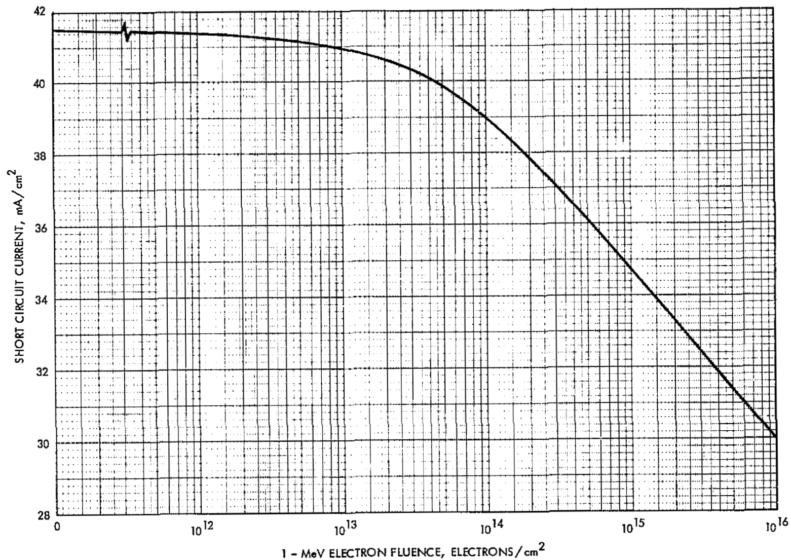
Figure 3.111 Short Circuit Current vs 1 MeV Electron Fluence for 10 Ohm-cm n/p Textured with Back Surface Field Silicon Cells. At 135.3 mW/cm² AMO Illumination, 30°C
