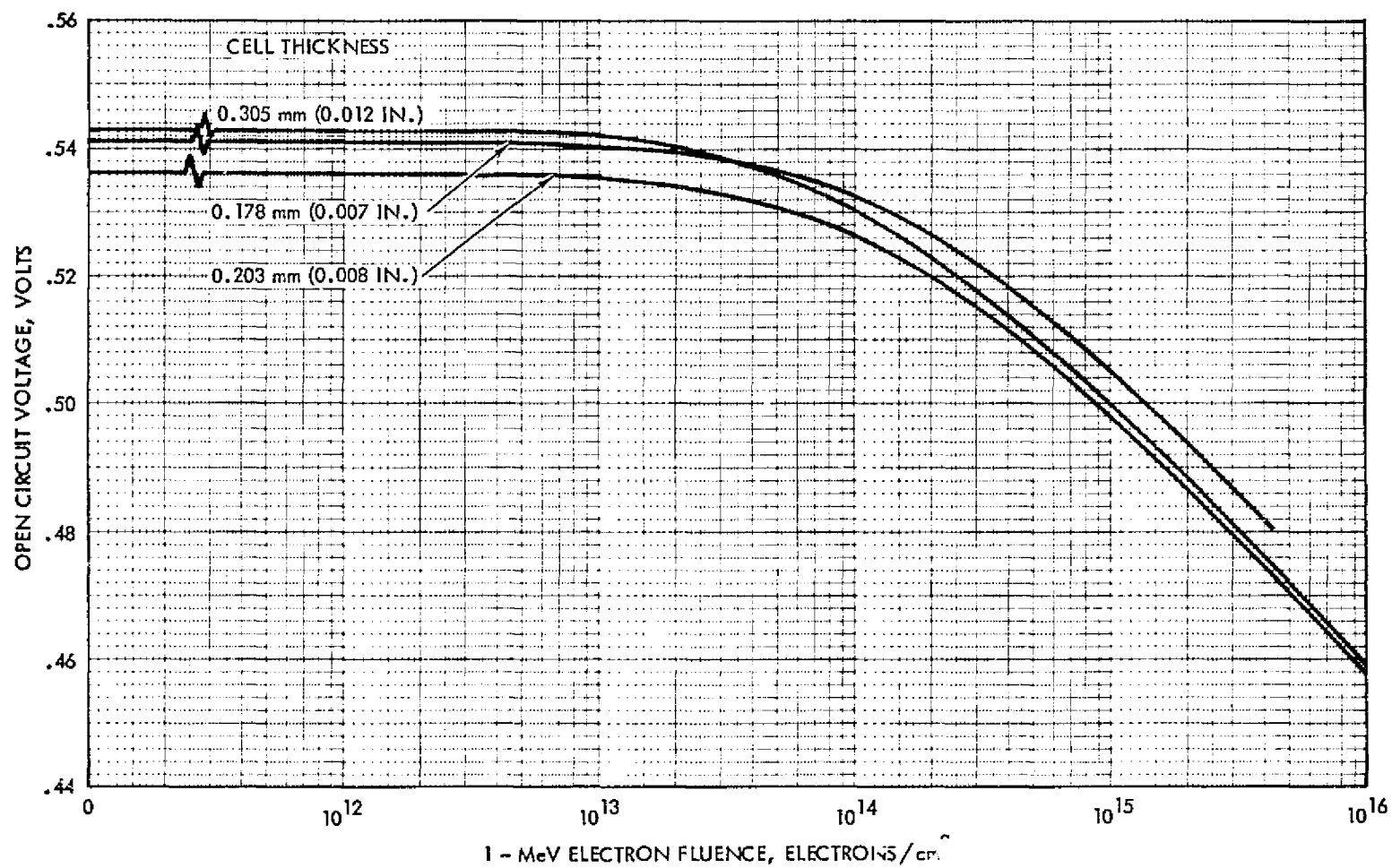
Figure 3.32 Open Circuit Voltage vs 1 MeV Electron Fluence for 10 Ohm-cm n/p Conventional Silicon Cells. At 135.3mw/cm AMO Illumination, 30° C
