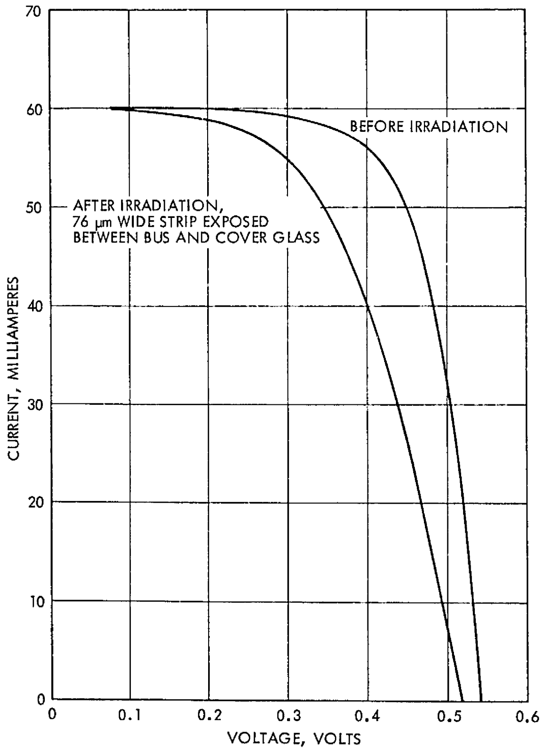
Figure 3.13 Low Energy Proton Junction Damage, 0.250 MeV Protons, 3 \times 10^{13} \text{p/cm}^2 , Partially Shielded N-P Solar Cell
