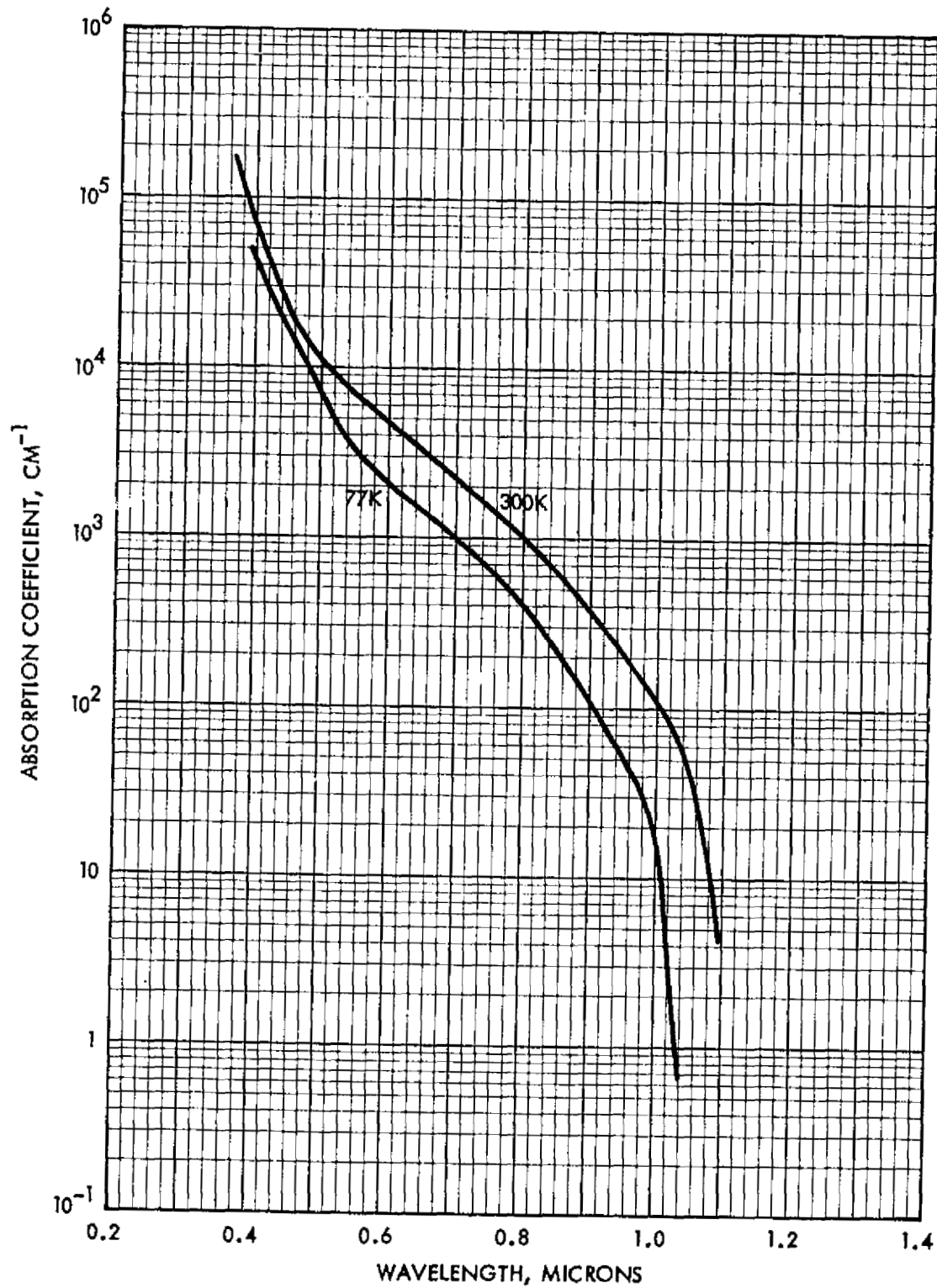
Figure B-3 Absorption Coefficient of Single Crystal Silicon at 77 K and 300 K
