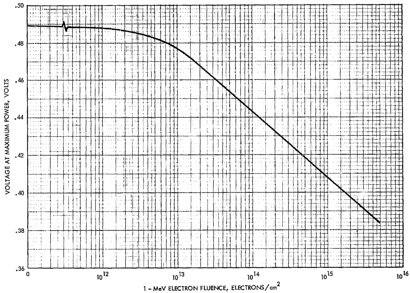
Figure 3.114 Voltage at Maximum Power vs 1 MeV Electron Fluence for 10 Ohm-cm n/p Textured with Back Surface Field Silicon Cells. At 135.3 mW/cm² AMO Illumination, 30°C
