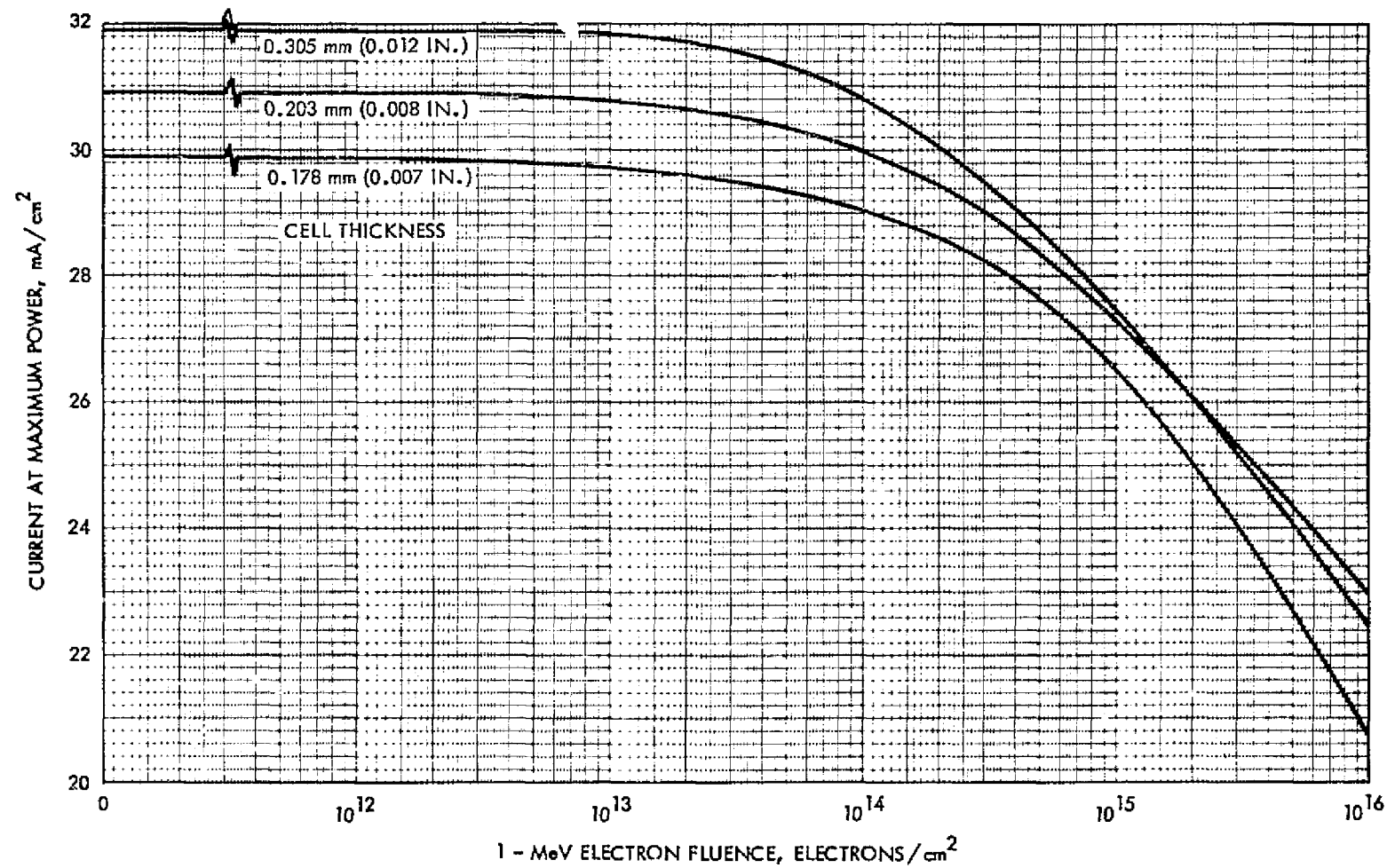
Figure 3.35 Current at Maximum Power vs 1 MeV Electron Fluence for 10 Ohm-cm n/p Conventional Silicon Cells. At 135.3 \text{ mW}/\text{cm}^2 AMO Illumination, 30^\circ\text{C}
