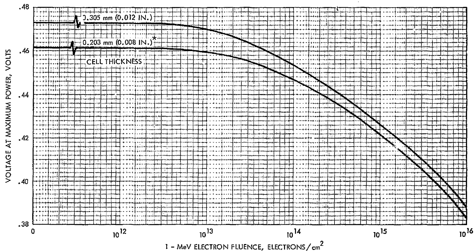
Figure 3.94 Voltage at Maximum Power vs 1 MeV Electron Fluence for 2 Ohm-cm n/p Textured Silicon Cells. At 135.3 mW/cm 2 AMO Illumination, 30°C
