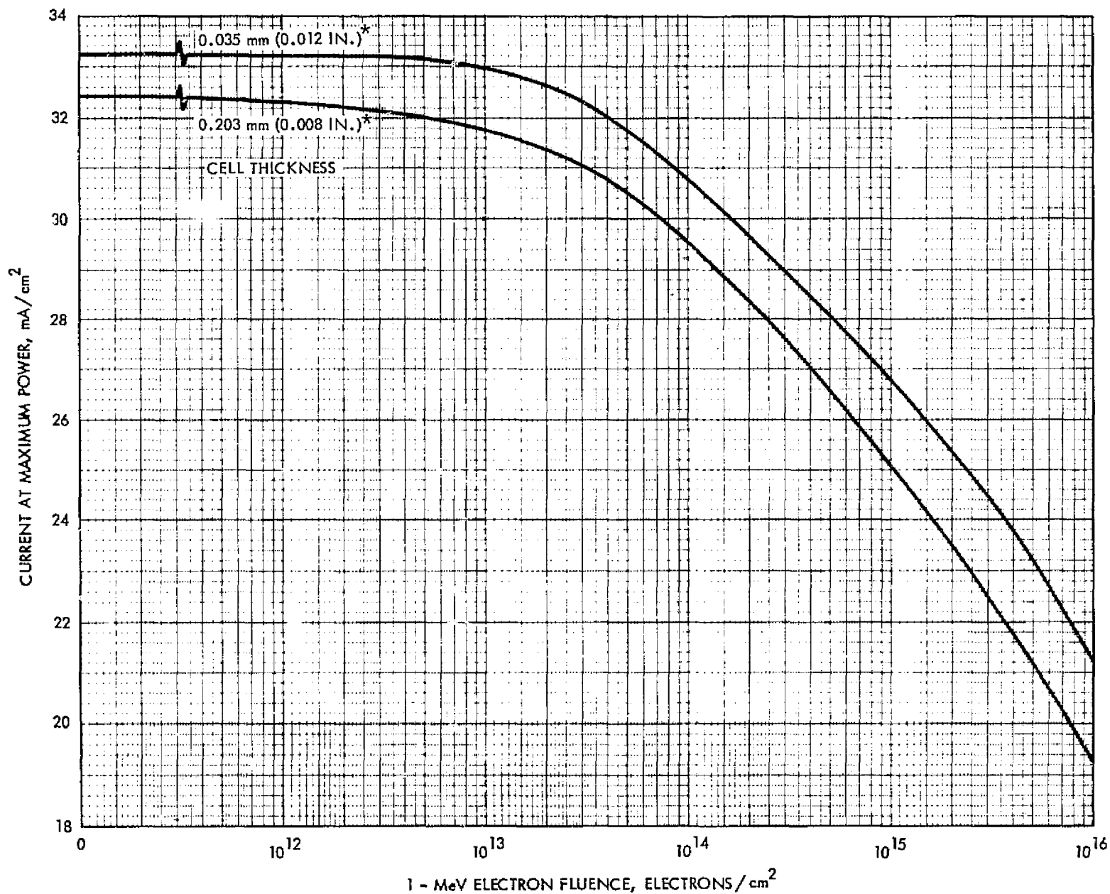
Figure 3.45 Current at Maximum Power vs 1 MeV Electron Fluence for 2 Ohm-cm n/p Shallow Junction Silicon Cells. At 135.3 mW/cm² AMO Illumination, 30°C
