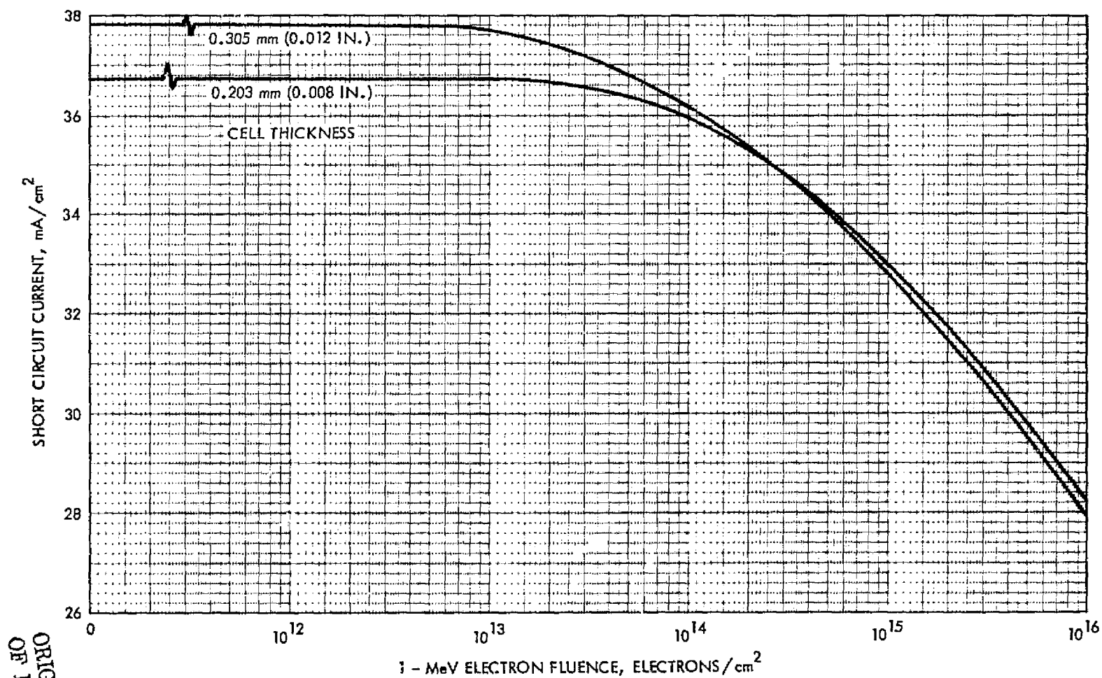
Figure 3.51 Short Circuit Current vs 1 MeV Electron Fluence for 10 Ohm-cm n/p Shallow Junction Silicon Cells. At 135.3 mW/cm² AND Illumination, 30°C
