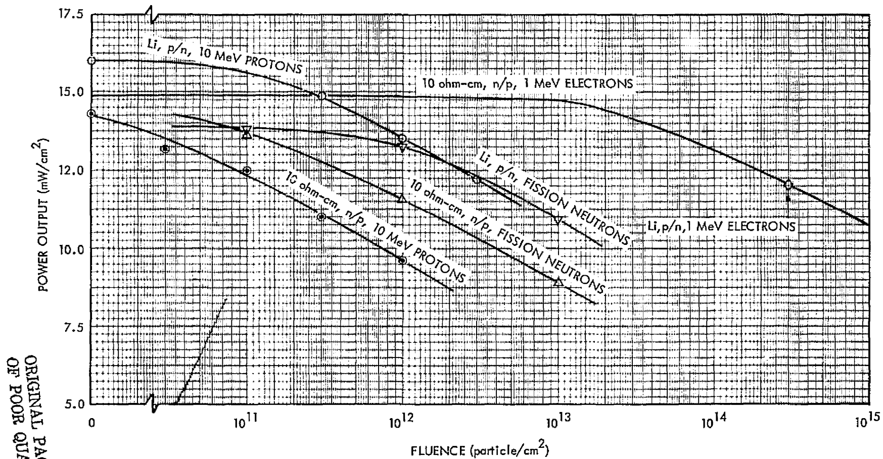
Figure 3.19 Recovered Power Output of Irradiated Conventional and Lithium Doped Solar Cells 3.90,3.93,3.53
