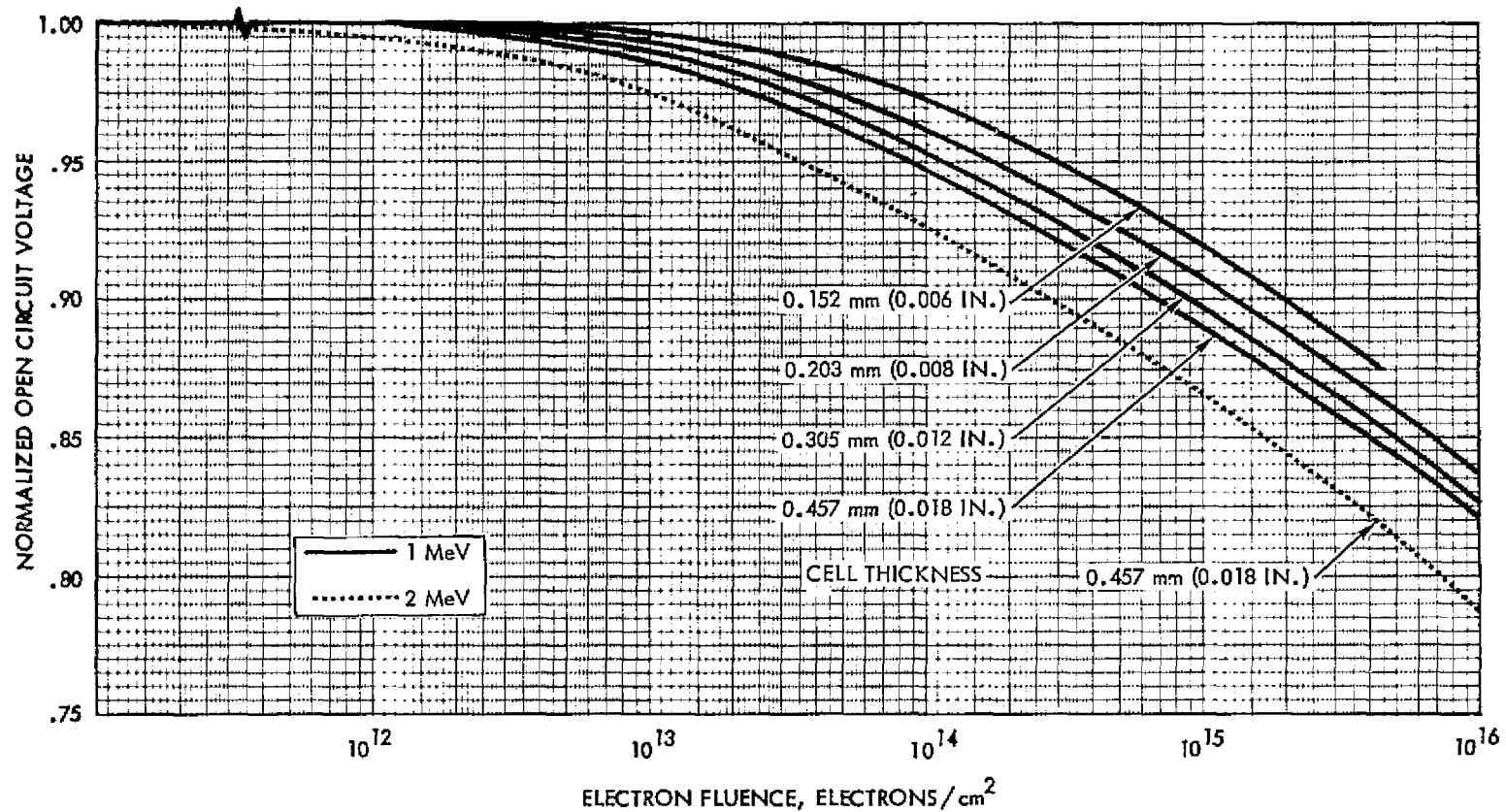
Figure 3.27 Normalized Open Circuit Voltage vs 1 MeV Electron Fluence for 2 Ohm-cm n/p Conventional Silicon Cells. At 135.3 mW/cm 2 AMO Illumination, 30°C
