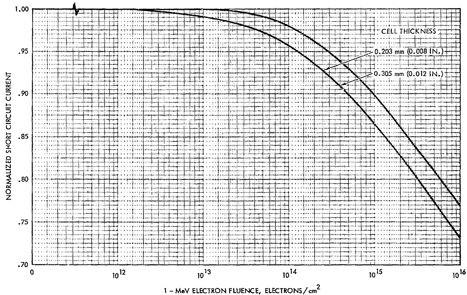
Figure 3.56 Normalized Short Circuit Current vs 1 MeV Electron Fluence for 10 Ohm-cm n/p Shallow Junction Silicon Cells. At 135.3 \text{ mW}/\text{cm}^2 AMO Illumination, 30^\circ\text{C}
