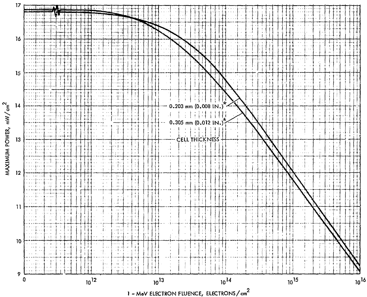
Figure 3.73 Maximum Power vs 1 MeV Electron Fluence for 10 Ohm-cm n/p Back Surface Field Silicon Cells. At 135.3 \text{ mW}/\text{cm}^2 AMO Illumination, 30^\circ\text{C}
