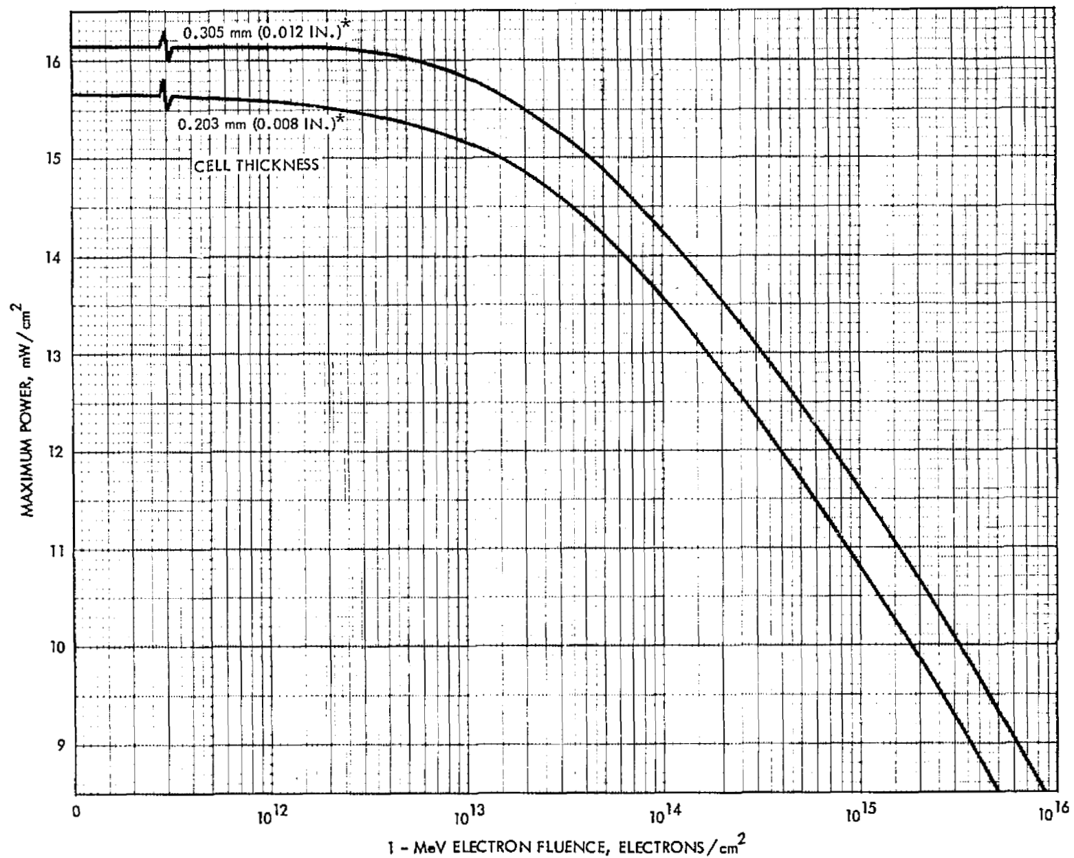
Figure 3.43 Maximum Power vs 1 MeV Electron Fluence for 2 Ohm-cm n/p Shallow Junction Silicon Cells. At 135.3 \text{ mW}/\text{cm}^2 AMO Illumination, 30^\circ\text{C}
