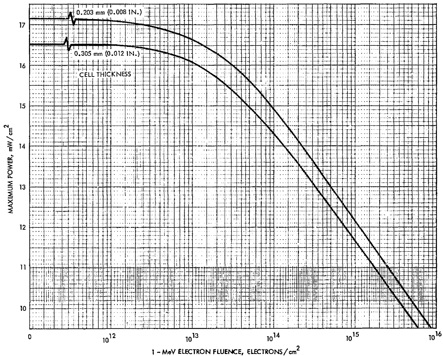
Figure 3.83 Maximum Power vs 1 MeV Electron Fluence for 20 Ohm-cm n/p Back Surface Field Silicon Cells. At 135.3 \text{ mW}/\text{cm}^2 AMO Illumination, 30^\circ\text{C}
