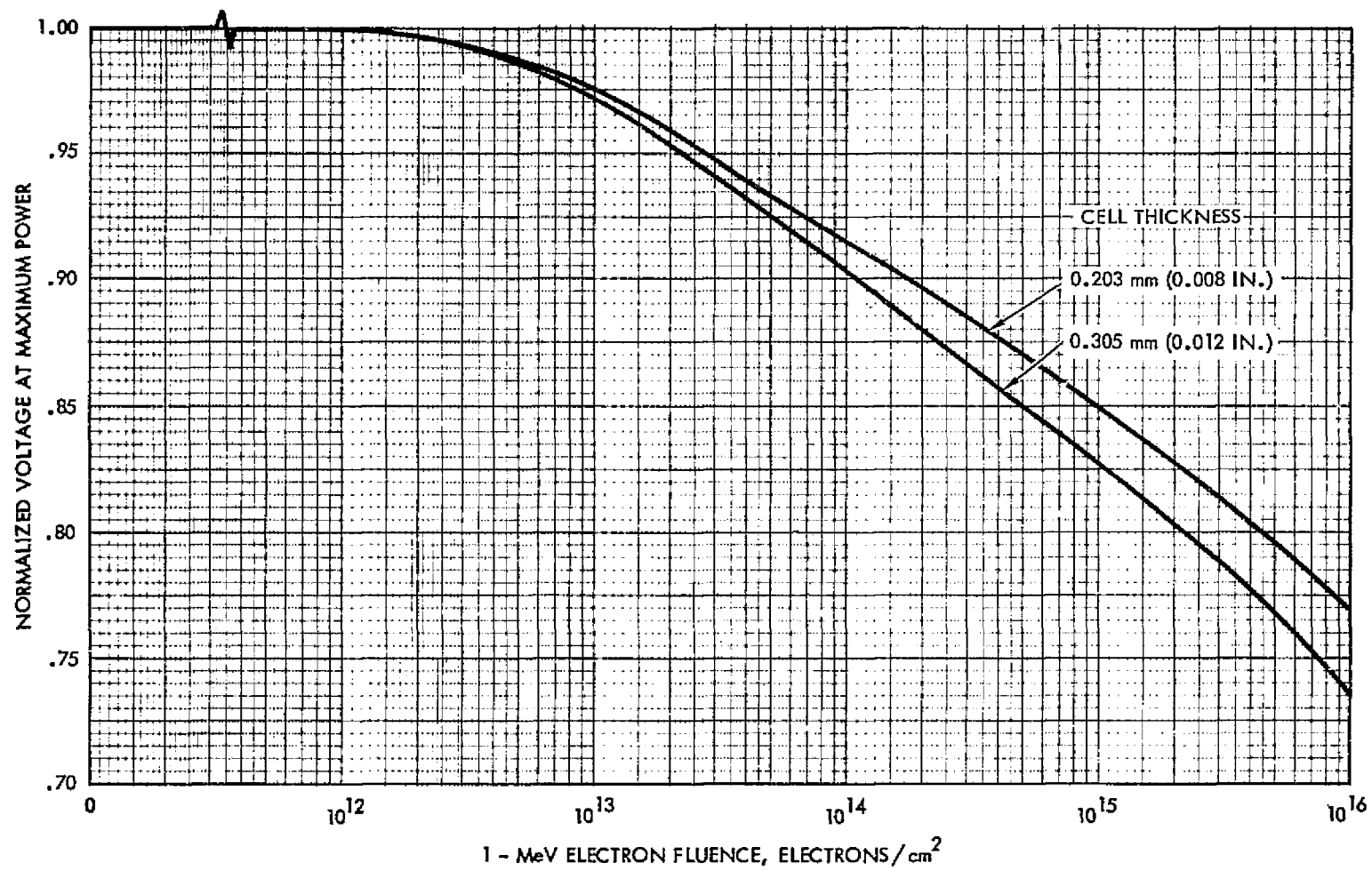
Figure 3.89 Normalized Voltage at Maximum Power vs 1 MeV Electron Fluence for 20 Ohm-cm n/p Back Surface Field Silicon Cells. At 135.3 \text{ mW/cm}^2 AMO Illumination, 30^\circ\text{C}
