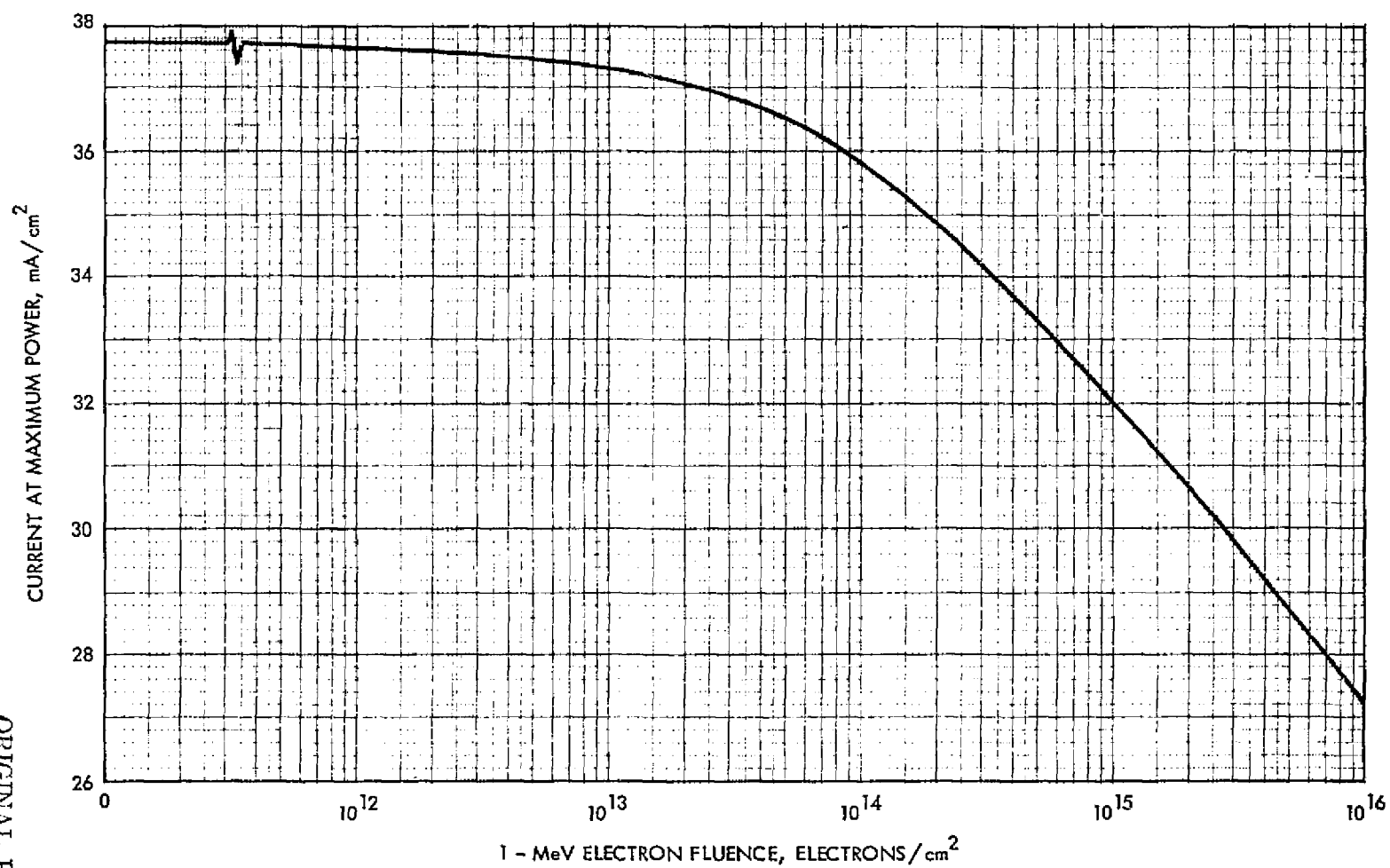
Figure 3.115 Current at Maximum Power vs 1 MeV Electron Fluence for 10 Ohm-cm n/p Textured with Back Surface Field Silicon Cells. At 135.3 mW/cm² AMO Illumination, 30°C
