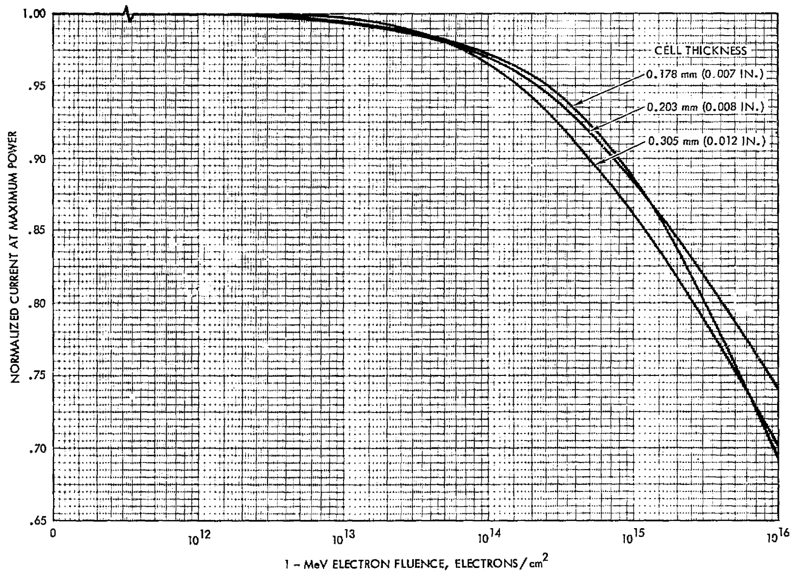
Figure 3.40 Normalized Current at Maximum Power vs 1 MeV Electron Fluence for 10 Ohm-cm n/p Conventional Silicon Cells.
