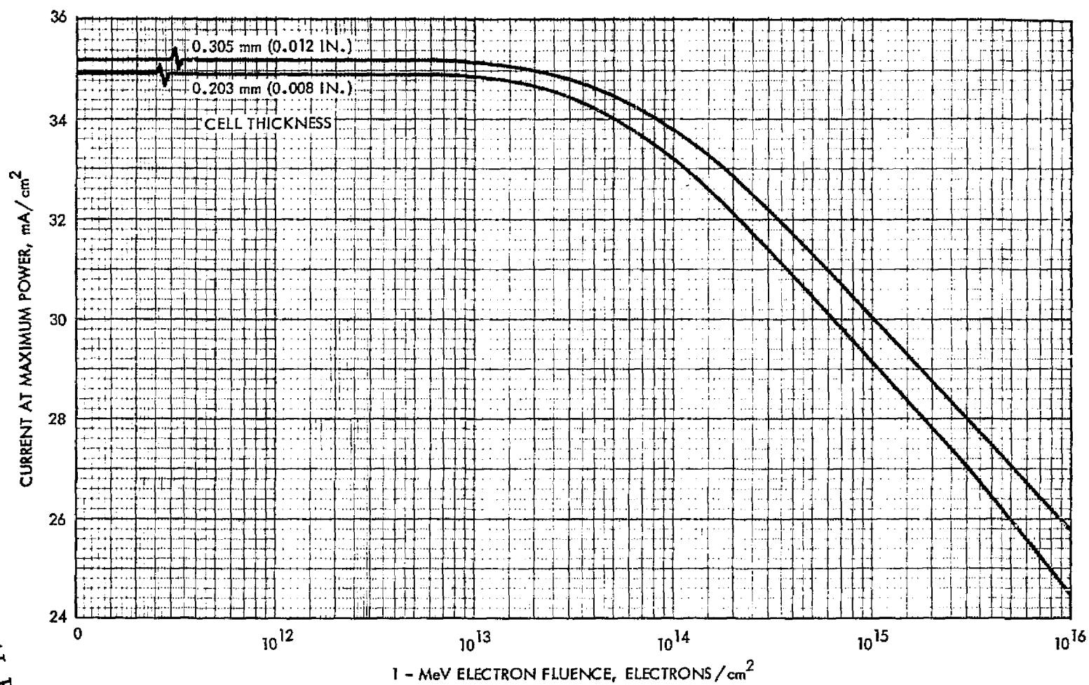
Figure 3.85 Current at Maximum Power vs 1 MeV Electron Fluence for 20 Ohm-cm n/p Back Surface Field Silicon Cells. At 135.3 mW/cm 2 AMO Illumination, 30°C
