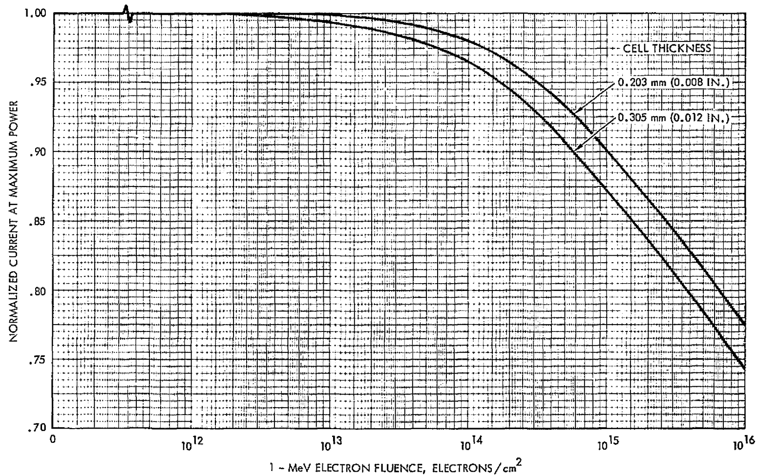
Figure 3.110 Normalized Current at Maximum Power vs 1 MeV Electron Fluence for 10 Ohm-cm n/p Textured Silicon Cells. At 135.3 mW/cm 2 AMO Illumination, 30°C
