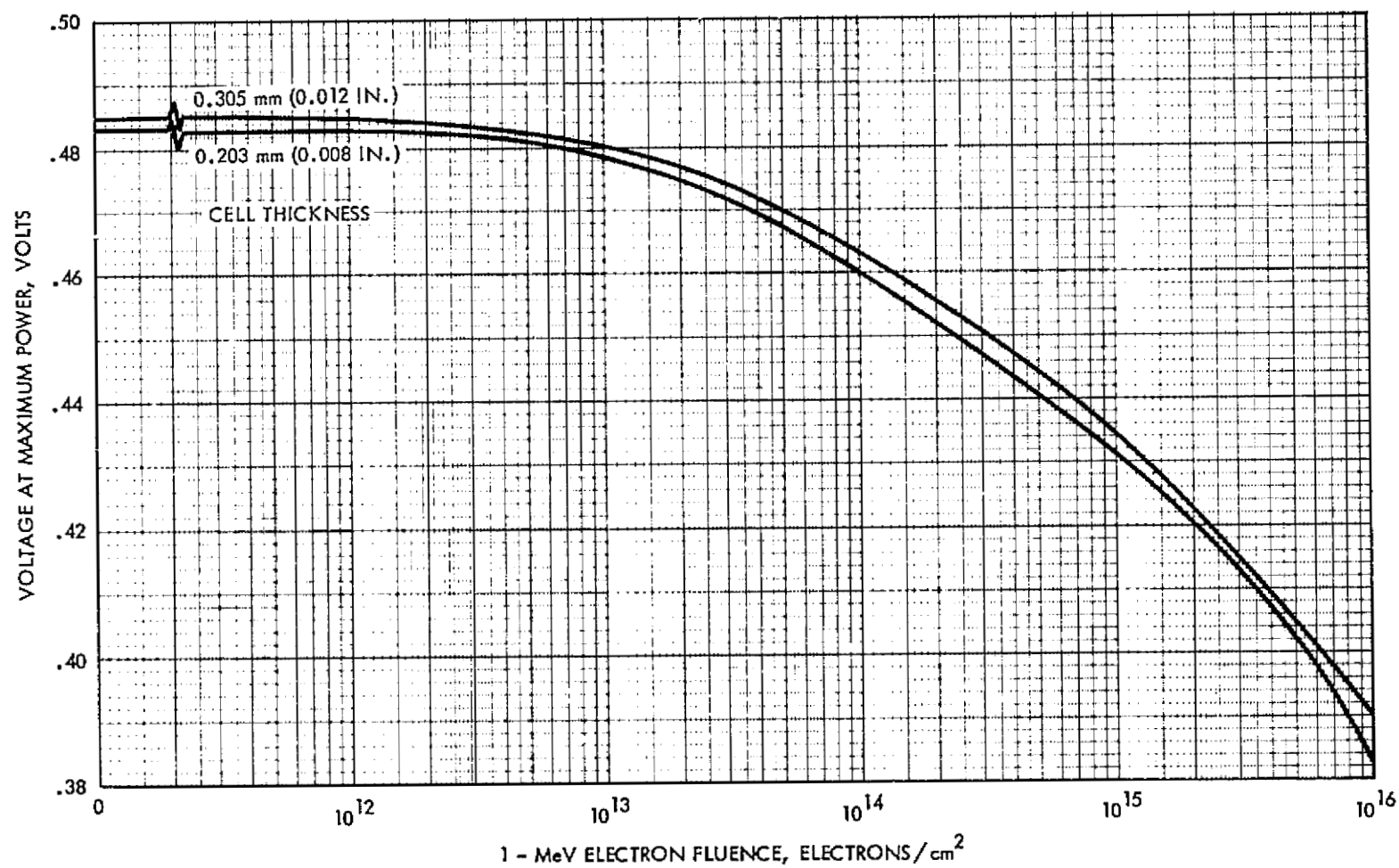
Figure 3.44 Voltage at Maximum Power vs 1 MeV Electron Fluence for 2 Ohm-cm n/p Shallow Junction Silicon Cells. At 135.3 \text{ mW/cm}^2 AMO Illumination, 30^\circ\text{C}
