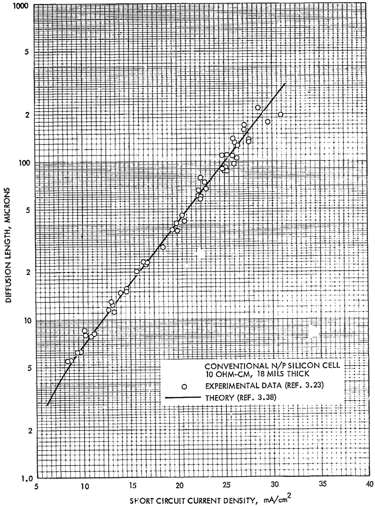
Figure 3.9 Minority Carrier Diffusion Length vs Short Circuit Density of Conventional N/P Silicon Cells.
