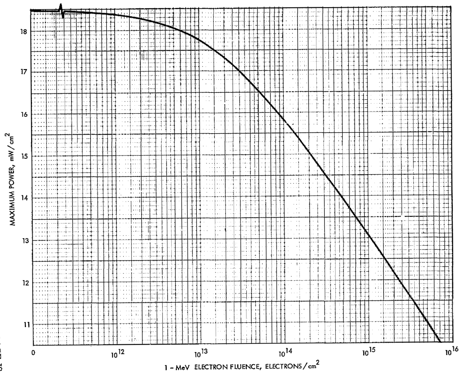
Figure 3.113 Maximum Power vs 1 MeV Electron Fluence for 10 Ohm-cm n/p Textured with Back Surface Field Silicon Cells. At 135.3 mW/cm² AMO Illumination, 30°C
