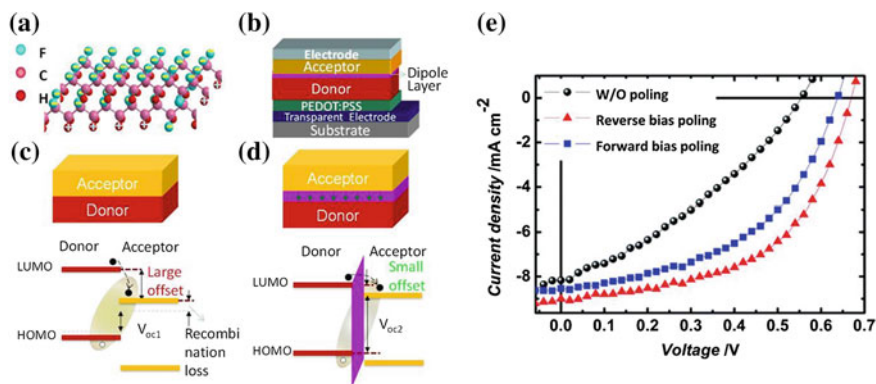
Fig. 7.16 a The molecular structure of a ferroelectric P(VDF-TrFE) dipole layer, b the device structure with a dipole layer inserted between the acceptor and the donor layers, the working principle to tune relative energy levels is shown in c bulk heterostructure without and d with a dipole layer inserted between the acceptor and the donor layers. e Tunable J - V curves with reverse bias poling and forward bias poling. Reprinted with permission from Yang et al. [51]. © (2012) WILEY-VCH Verlag GmbH & Co. KGaA, Weinheim
