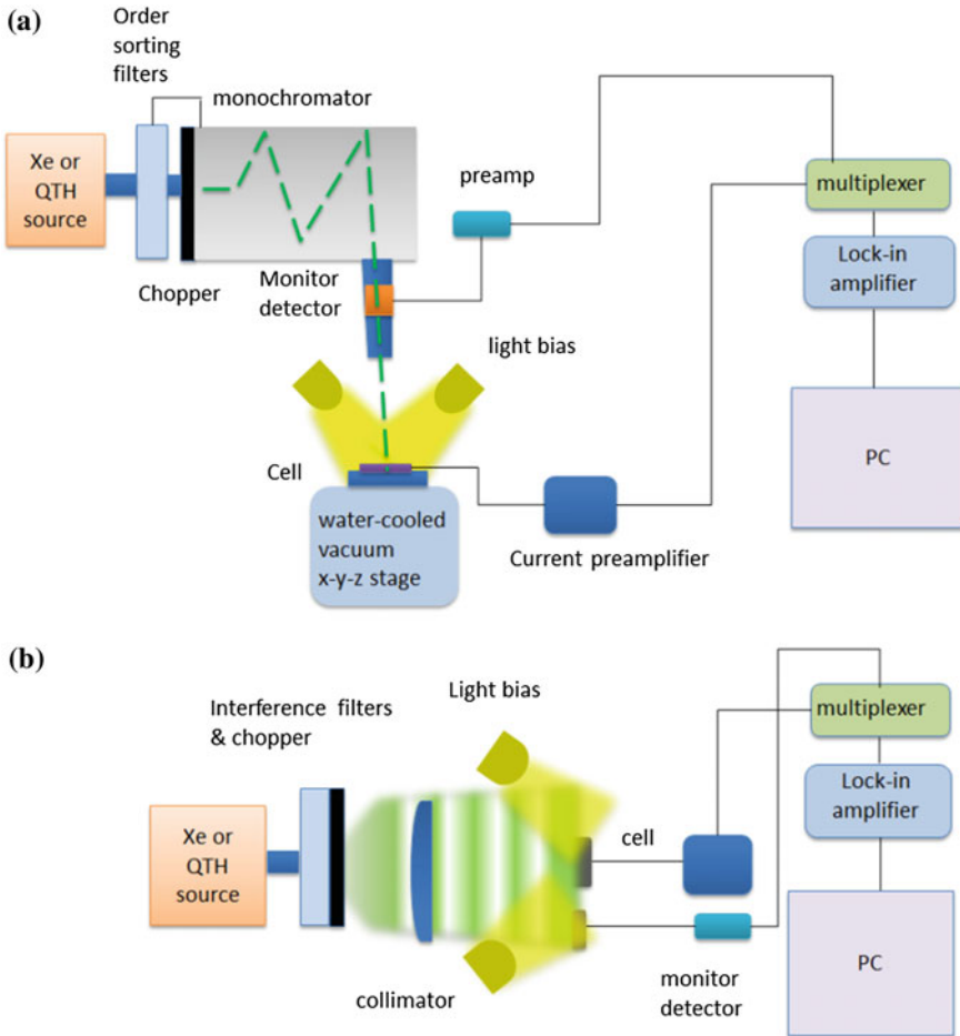
Fig. 8.4 a Schematics of a monochromator-based SR measurement system where the probe beam underfills the cell. b An example of an SR measurement system where the beam overfills the cell
