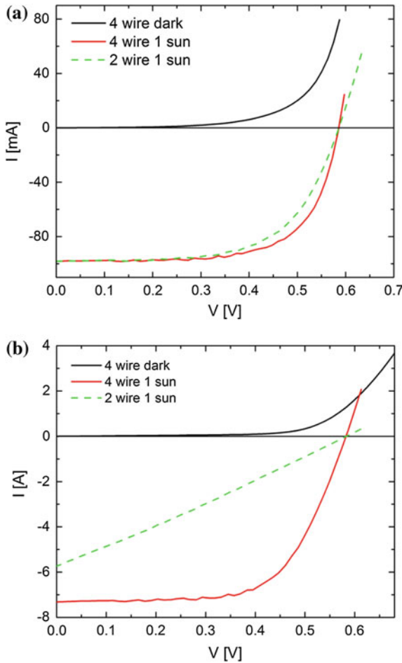
Fig. 8.8 a Comparison between 2 wire and 4 wire I - V measurements on a small 4 cm 2 solar cell. b Same comparison on a larger cell with an area of 219 cm 2 . The I - V curves measured in the dark are also plotted for both solar cells
