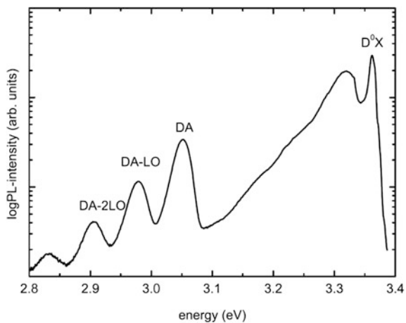
Fig. 4.1 PL spectra of CVD grown ZnO on GaN templates with in situ Li doping ( T = 4.2 \text{ K} , He–Cd laser excitation). The positions of the zero phonon line of the donor–acceptor pair band and its phonon replica are indicated [28]
