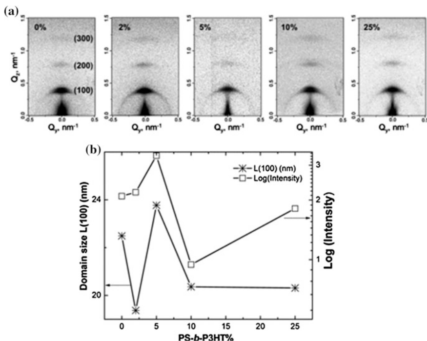
Fig. 7.9 a 2D GIXS patterns of the P3HT:PC 61 BM blend films with adding 0 wt%, 2 wt%, 5 wt%, 10 wt%, and 25 wt% of PS- b -P3HT compatibilizers. Q_z and Q_y are the perpendicular and parallel wave vectors transfer with respect to substrate surface. b The domain size and normalized peak intensity of (100) extracted from 1D GIXS measurement. Reprinted with permission from Sun et al. [17]. © (2011) WILEY-VCH Verlag GmbH & Co. KGaA, Weinheim
