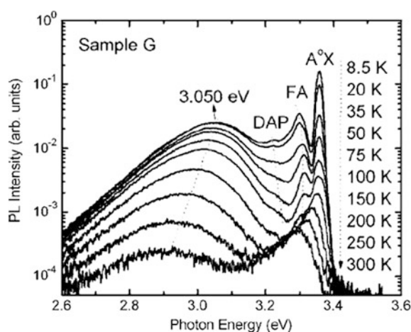
Fig. 4.15 PL spectra measured at several temperatures over the range from 8.5 to 300 K for an Sb-doped p-type ZnO [96]
