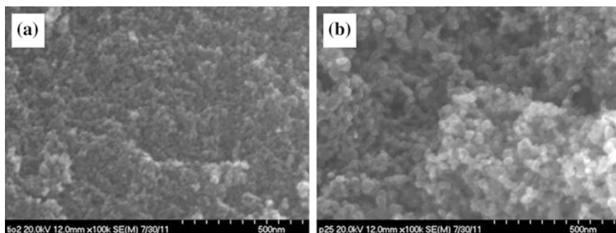
Fig. 5.1 The surface features of the a IH- \text{TiO}_2 and b commercially procured P25 (Degussa ® corporation) are observed in these representative images obtained using the scanning electron microscope
