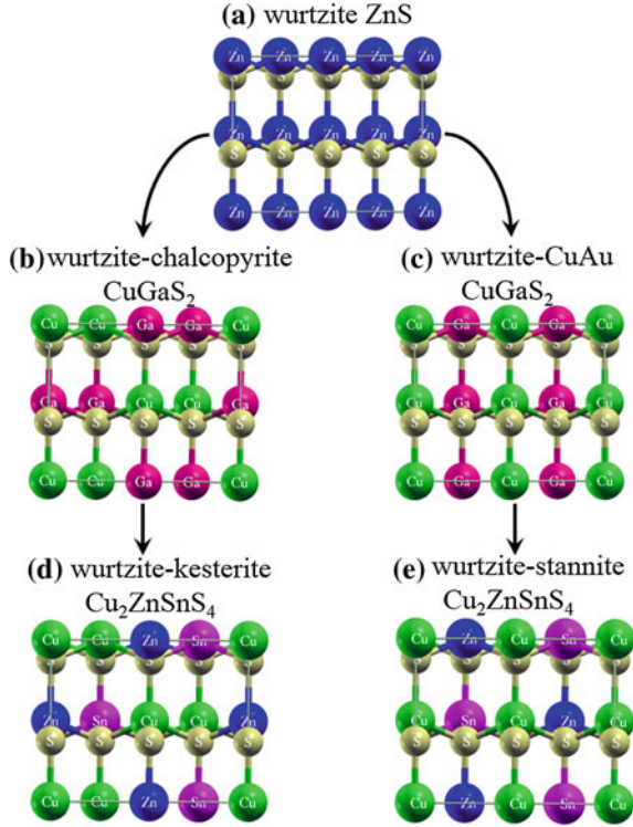
Fig. 3.4 The crystal structure mutation from wurtzite \text{ZnS} to chalcopyrite \text{CuGaS}_2 and \text{CuAu CuGaS}_2 , then to wurtzite-kesterite \text{Cu}_2\text{ZnSnS}_4 and stannite \text{Cu}_2\text{ZnSnS}_4
