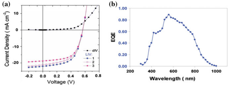
Fig. 2.27 a I - V characteristics of electrodeposited CZTS solar cell under dark (black) and 1 sun (lines 1, 2, and 3) illumination for a champion CZTS cell, showing efficiencies of 7.3, 6.74, and 6.86 %, respectively. b The quantum efficiency (QE) curve. LIV and dIV mean light and dark current-voltage curve, respectively [138]
