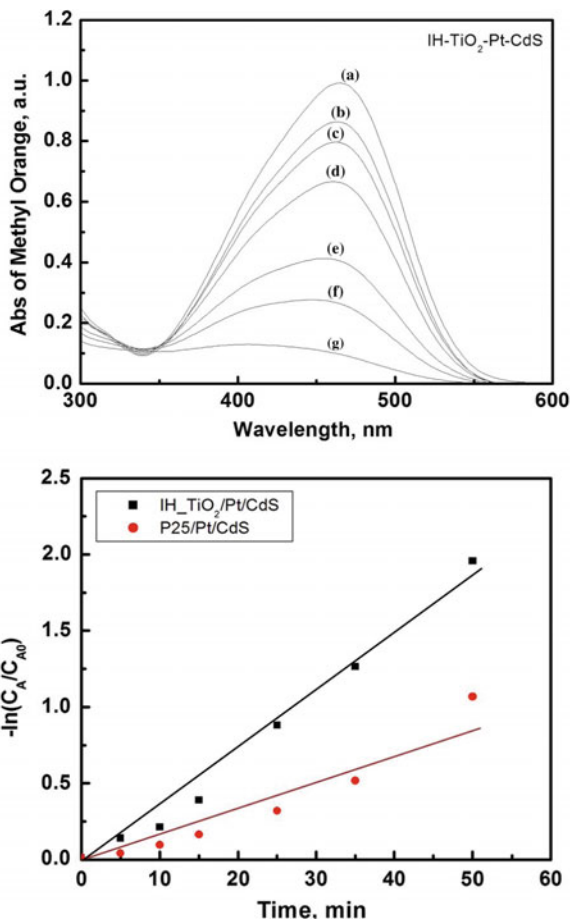
Fig. 5.13 a The absorbance spectra of the MO solution was monitored at the end of a 0, b 5, c 10, d 15, e 25, f 35, and g 50 min to determine the fractional conversion of the methyl orange dye during the simultaneous production of hydrogen. b A pseudo-first-order linearized kinetic model was applied to the absorbance data to determine the rate constant. The linear fit indicates that the photodegradation follows the first-order kinetics
