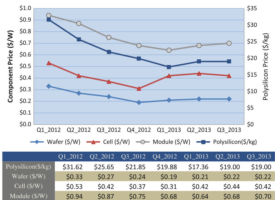
Fig. 9.11 US polysilicon, wafer, cell, and module prices. Source US solar market insight: year in review 2012; solar market insight 2013 Q3
