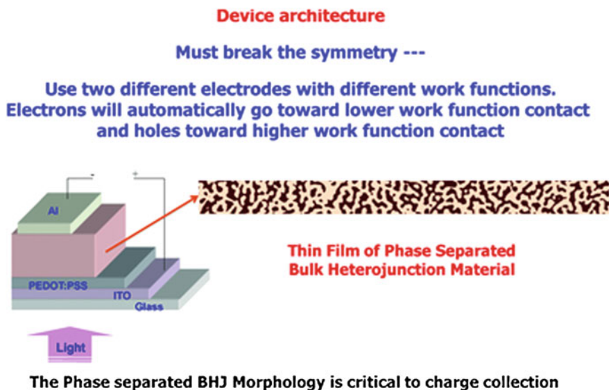
Fig. 6.3 The BHJ concept [18]
