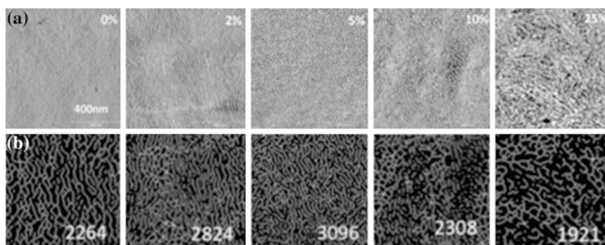
Fig. 7.8 a AFM phase images of P3HT:PC 61 BM blend films with 0 wt%, 2 wt%, 5 wt%, 10 wt%, 25 wt% PS-b-P3HT compatibilizers. b The features in the mid-frequency range after Fourier transform for corresponding AFM phase images. 5 wt% of PS-b-P3HT compatibilizers showed the best ordering of P3HT polymer and penetrating network. Reproduced with permission from Sun et al. [17]. © (2011) WILEY-VCH Verlag GmbH & Co. KGaA, Weinheim
