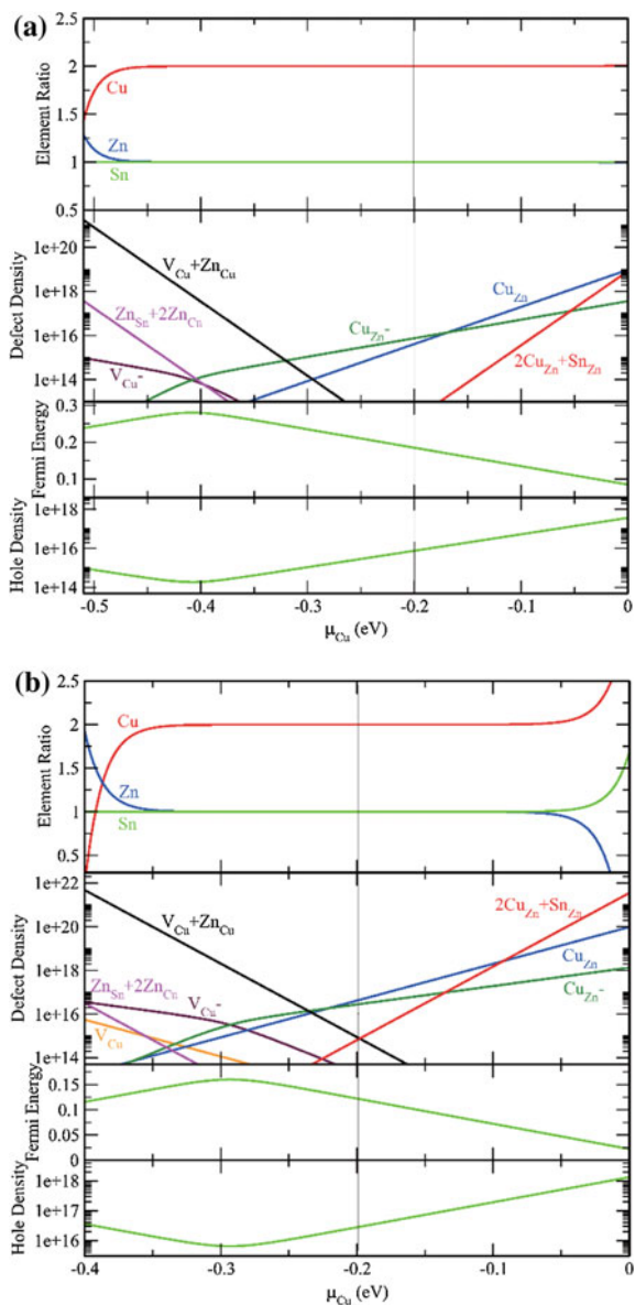
Fig. 3.15 Calculated element ratio, defect density ( \text{cm}^{-3} ), Fermi energy (in eV relative to VBM), and hole density ( \text{cm}^{-3} ) at room temperature as functions of the Cu chemical potential for a \text{Cu}_2\text{ZnSnS}_4 and b \text{Cu}_2\text{ZnSnSe}_4 . Adapted from Ref. [79]
