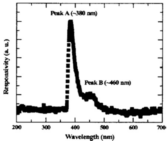
Fig. 4.13 Spectral response for a ZnO photodiode [82]
