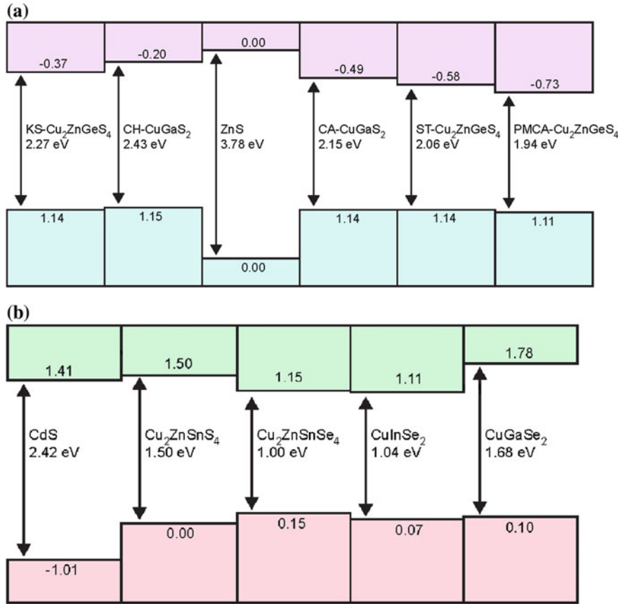
Fig. 3.8 The calculated band alignment for different binary, ternary, and quaternary chalcogenide semiconductors (calculations were performed using the GGA functional, with the spin-orbital interaction considered). Adapted from Ref. [61, 83]
