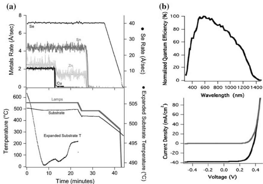
Fig. 2.15 a Deposition rate of source materials ( top ) and substrate temperature profile ( bottom ); b external quantum efficiency ( top ) and the illuminated J - V characteristic of the CZTSe device with 9.15 % efficiency ( bottom ) [14]
