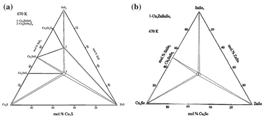
Fig. 2.4 Phase diagrams of a \text{Cu}_2\text{S}\text{--}\text{ZnS}\text{--}\text{SnS}_2 [44] and b \text{Cu}_2\text{Se}\text{--}\text{ZnSe}\text{--}\text{SnSe}_2 pseudo-ternary systems at 670 K [45]
