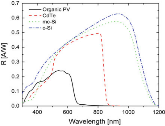
Fig. 8.5 Power-mode spectral response curves of a few different types of solar cells
