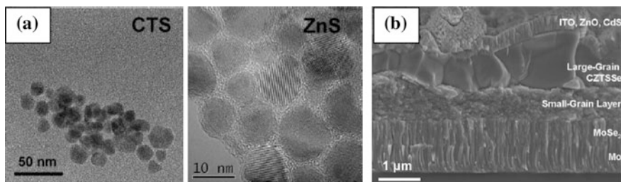
Fig. 2.21 a TEM images of the as-synthesized copper-tin-sulfide and ZnS nanocrystals and b cross-sectional SEM image of the completed device structure [126]
