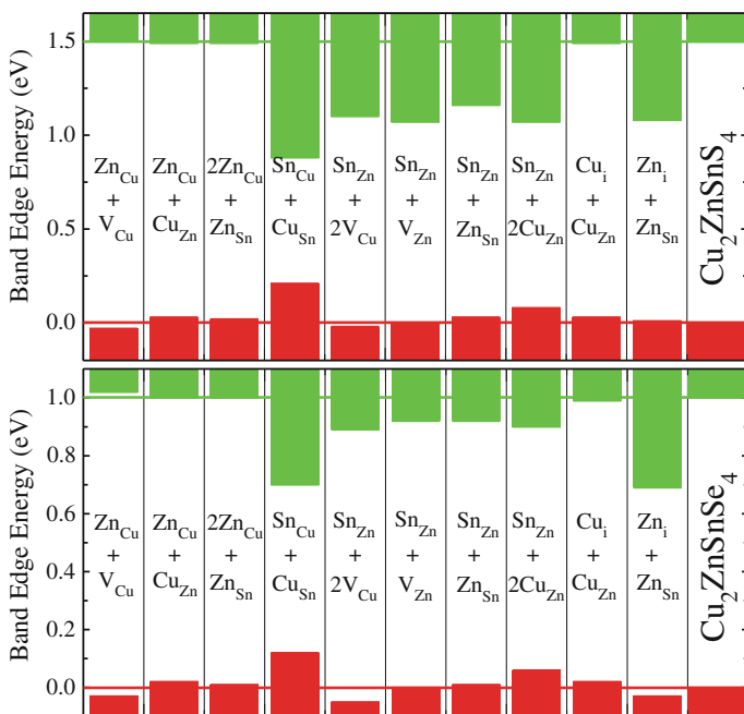
Fig. 3.14 The valence and conduction band shifts caused by different defect clusters in \text{Cu}_2\text{ZnSnS}_4 (top panel) and \text{Cu}_2\text{ZnSnSe}_4 (bottom panel). Adapted from Ref. [79]
