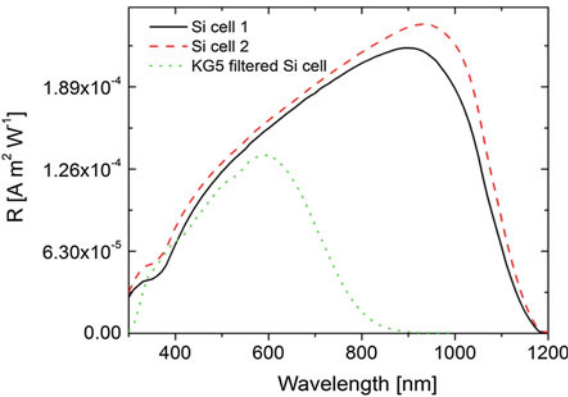
Fig. 8.6 Irradiance-mode spectral response curves of a few solar cells
