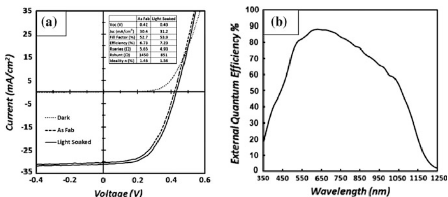
Fig. 2.20 a J - V characteristics of the best CZTSSe solar cell without and with 15-min light soaking and b external quantum efficiency of the corresponding device [18]
