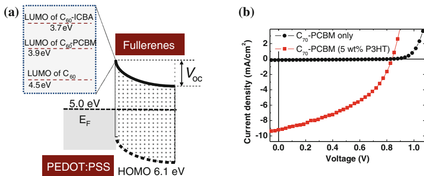
Fig. 7.15 a Schematic energy diagram showing the variation of V_{OC} following the LUMO of fullerene levels. b Device performance comparison between devices based on pristine PC_{71}BM and devices based on PC_{71}BM with adding 5 wt% P3HT. Reprinted with permission from Yang et al. [92]. © (2012) WILEY-VCH Verlag GmbH & Co. KGaA, Weinheim
