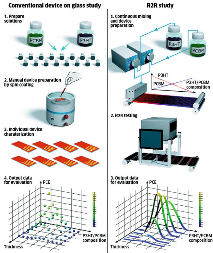
Fig. 6.16 Comparison of conventional small-scale OPV device optimization versus R2R optimization [143]
