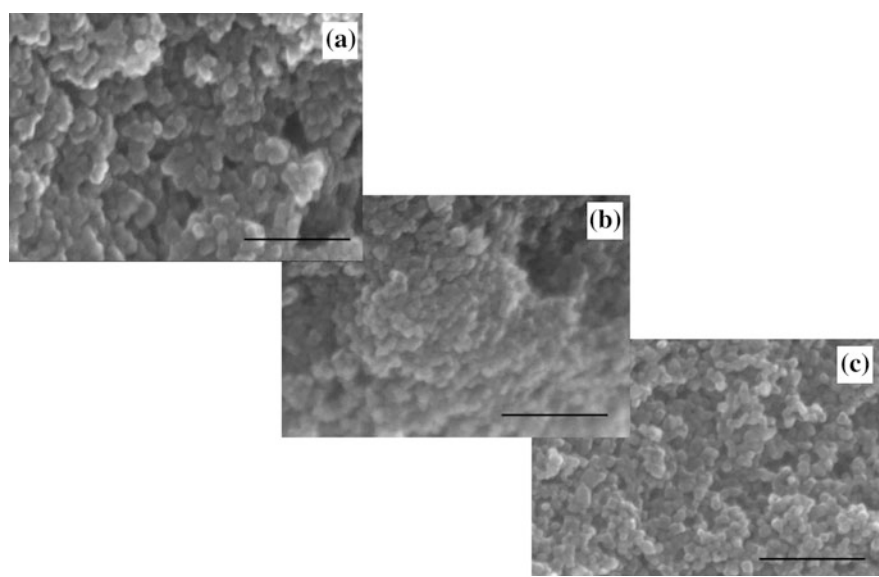
Fig. 5.2 The surface features of the IH-TiO 2 with different metal deposits are shown in these images obtained using the scanning electron microscope. This includes IH-TiO 2 with a Pt, b Au, and c Ag. All the samples have been shown with a scale of 200 nm
