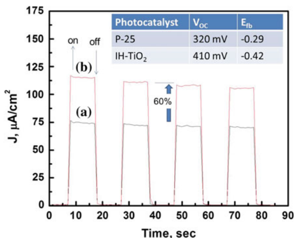
Fig. 5.8 The photocurrent measurements of the a commercial (Degussa® P25) and the b IH-TiO 2 are shown. The inset shows the stabilized values of the chronopotentiometry ( V_{OC}/i ) and the values of the flat-band potential ( E_{fb} ) for both TiO 2
