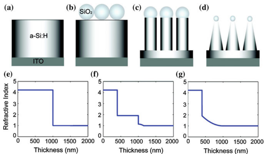
Fig. 1.6 a–d Schematic illustration of 1-μm-thick a-Si:H on ITO-coated glass substrate, a monolayer of silica nanoparticles on top of a-Si:H thin film, NW arrays, and NC arrays. The effective refractive index profiles of the interfaces between air and e a-Si:H thin film, f 600 nm a-Si:H NW arrays, and g 600 nm a-Si:H NC arrays. Adapted with permission from Ref. [27]. Copyright © 2009, American Chemical Society
