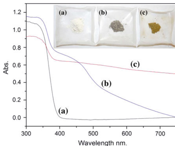
Fig. 5.5 UV-visible diffuse reflectance spectra of a IH-TiO 2 , b Pt deposits on IH-TiO 2 , and c CdS deposits on IH-TiO 2 -Pt. The inset shows the photographs of the different samples in the same order
