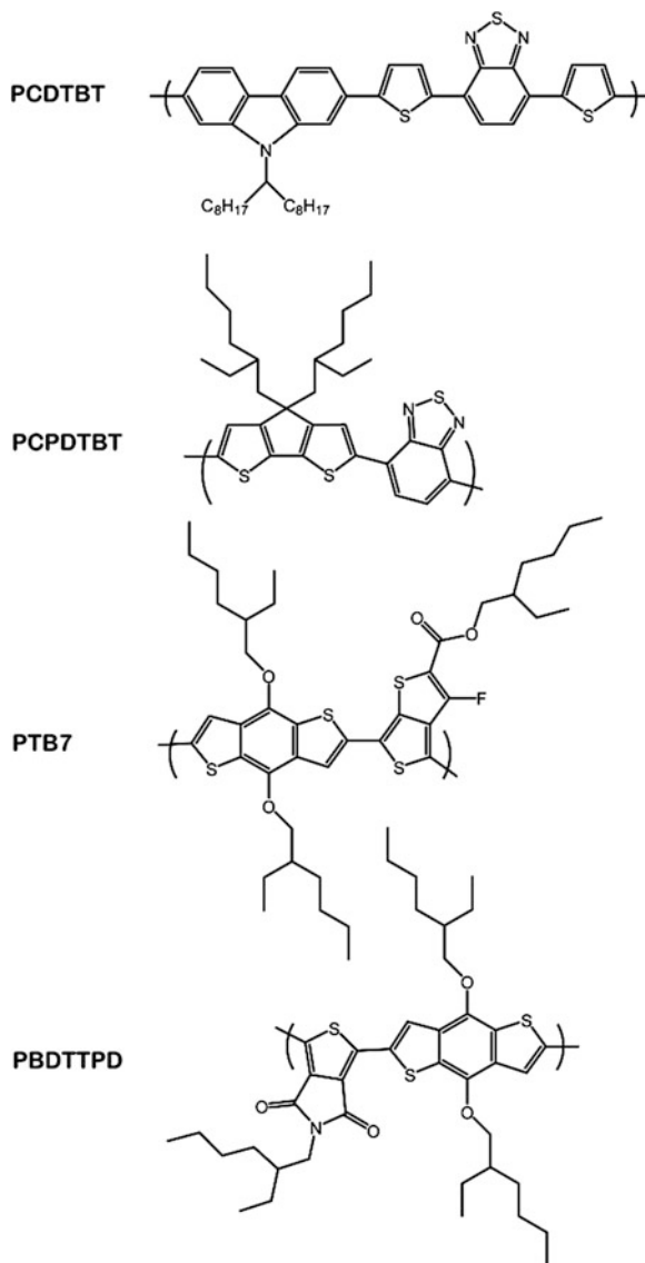
Fig. 6.6 Some commonly used donor polymers
