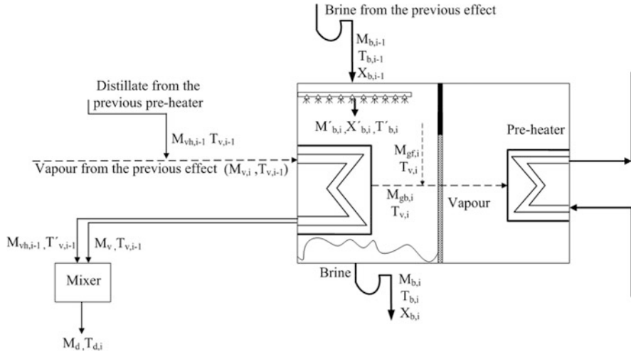
Fig. 3.6 Flow diagram of the subgroup G2-1
