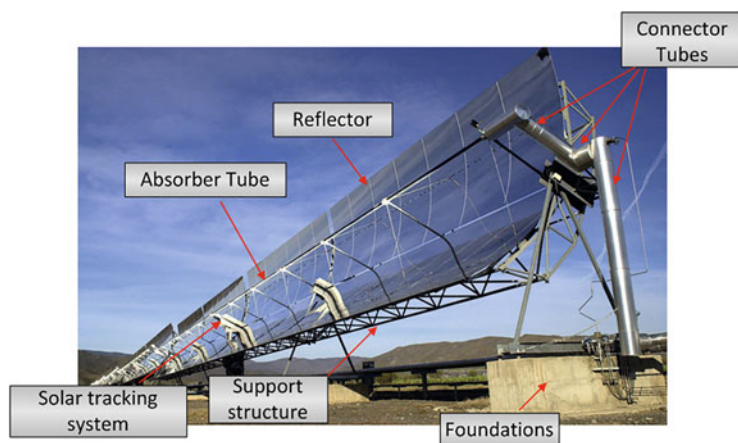
Fig. 4.4 Parabolic-trough collector components
