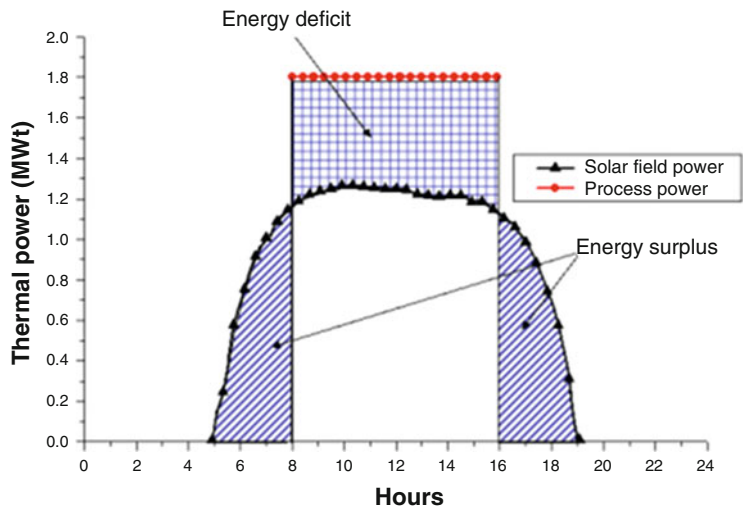
Fig. 4.10 Thermal power produced by the solar field and demanded by the process when the solar field feeds the plant for less hours than the sunlight hours
