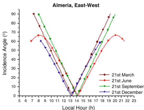
Fig. 4.8 Incidence angle variation between winter and summer, considering an east–west orientation
