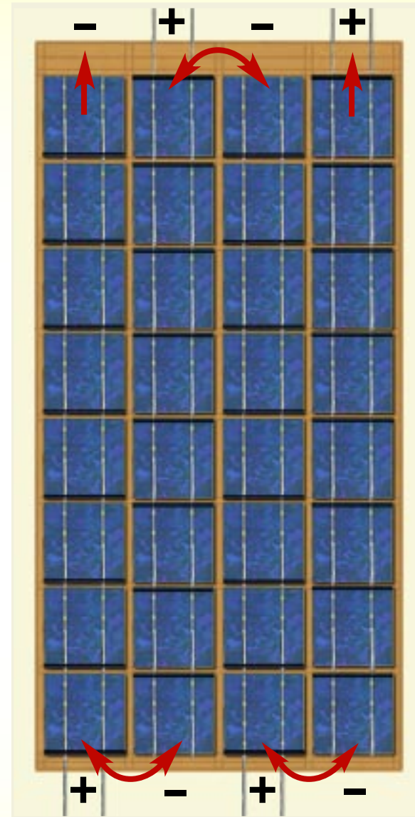
Strings of solar cells laid out on the template
