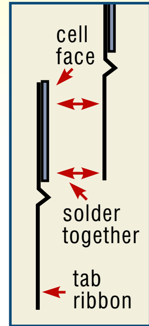
Solder the tabbed cells together (side view).
