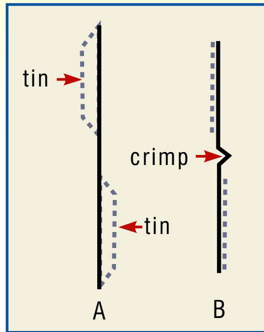
Side view of tinning and crimping the tab ribbon
