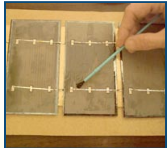
String layout board for soldering the cells together
